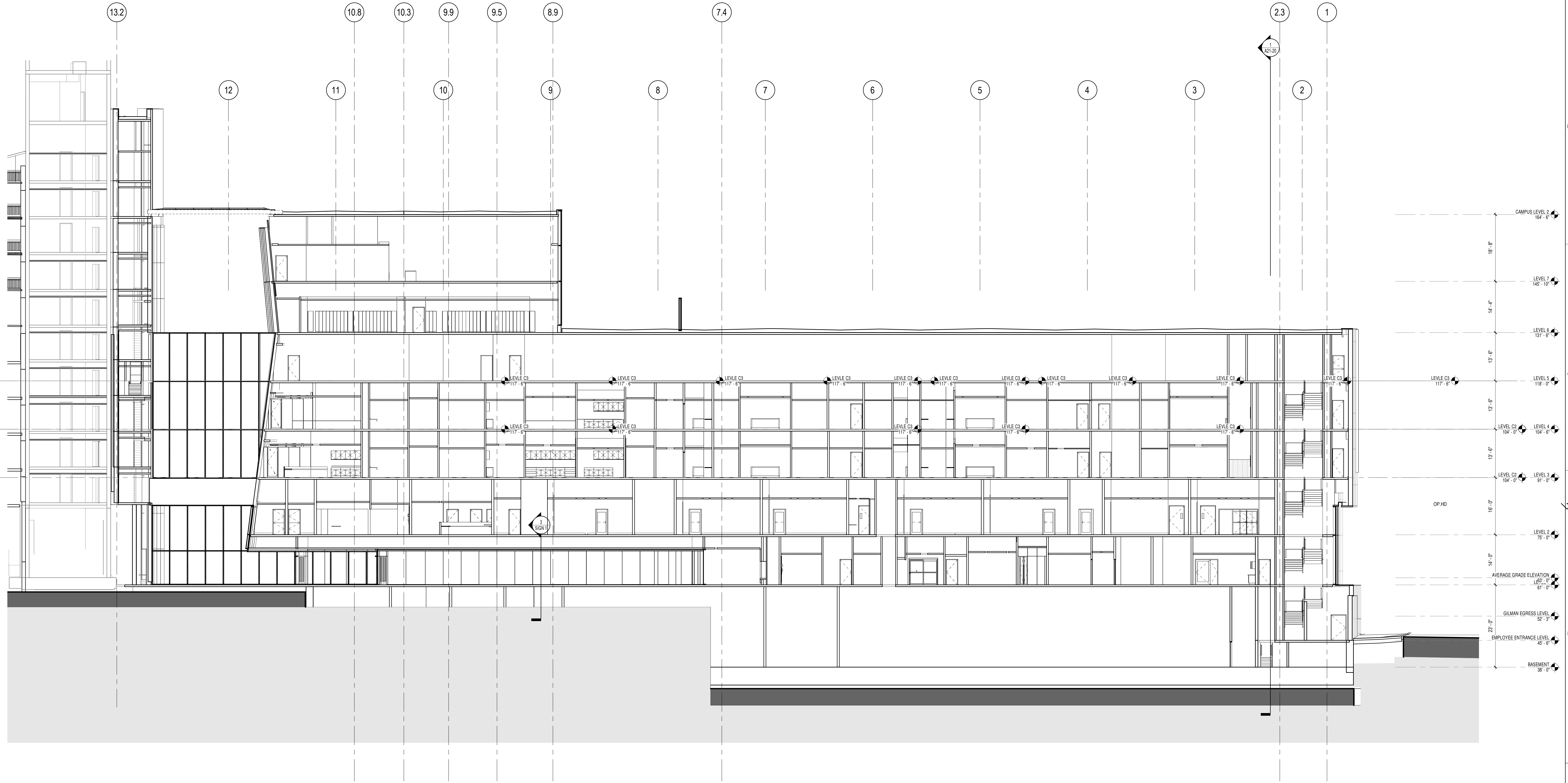
① BUILDING SECTION EAST / WEST (LOOKING SOUTH) 3/32" = 1'-0"
