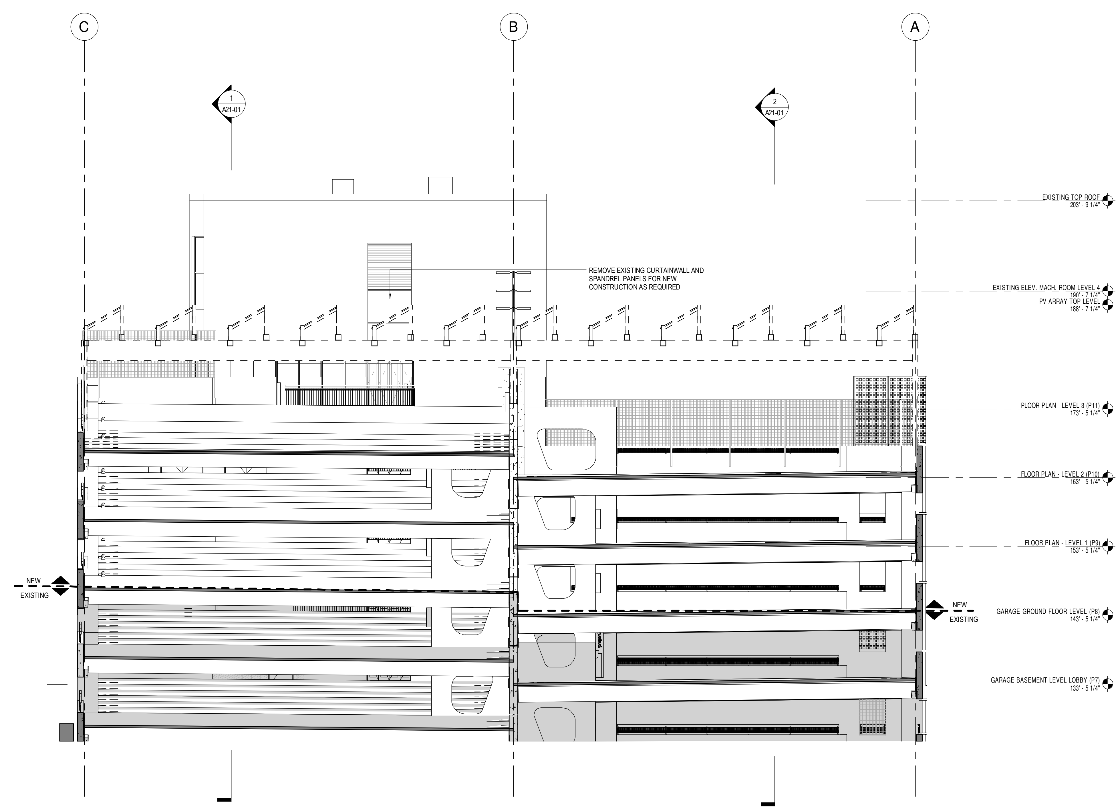
3 SECTION NORTH/SOUTH 1/8" = 1'-0"
