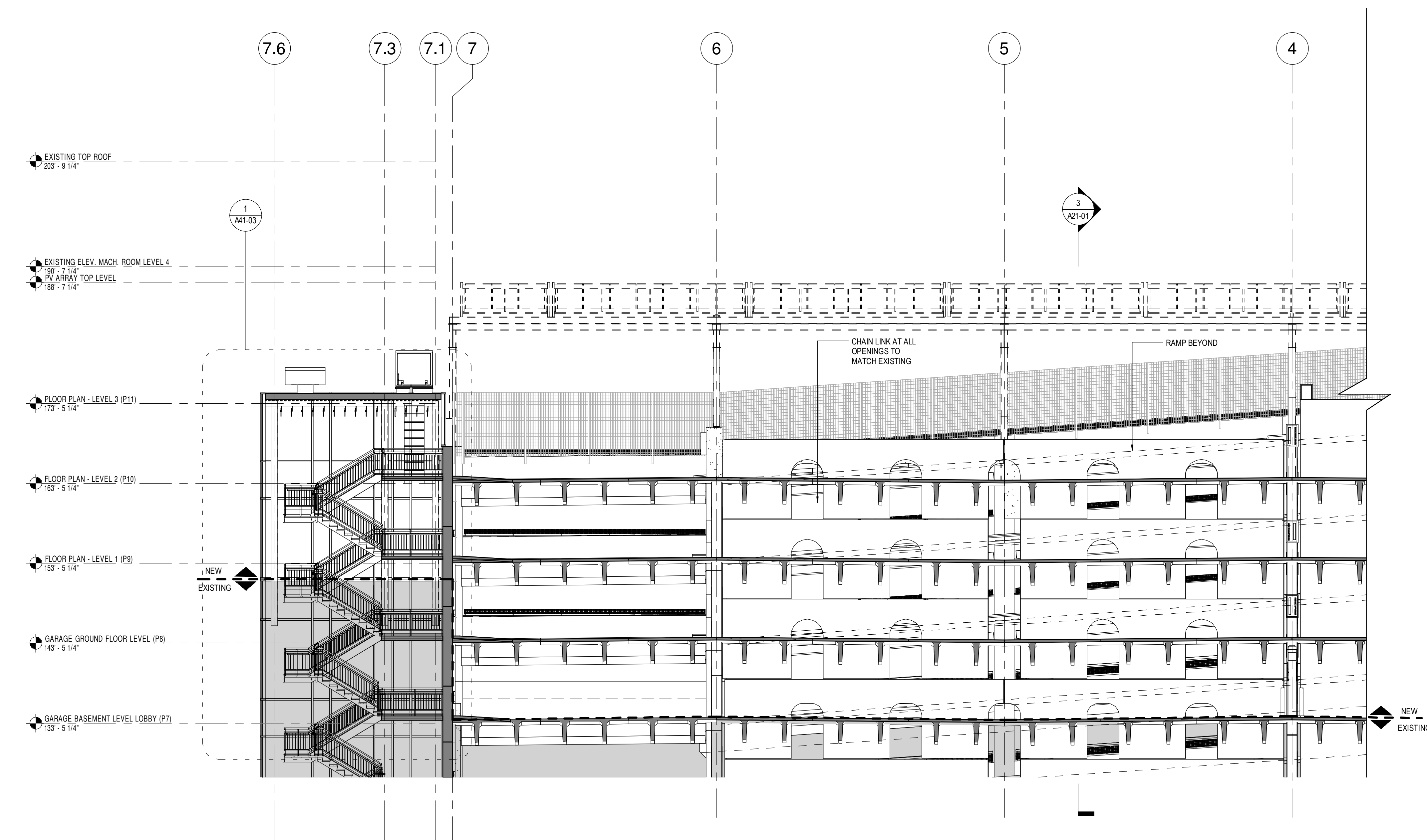
2 SECTION EAST/WEST THROUGH FLOOR 1/8" = 1'-0"
