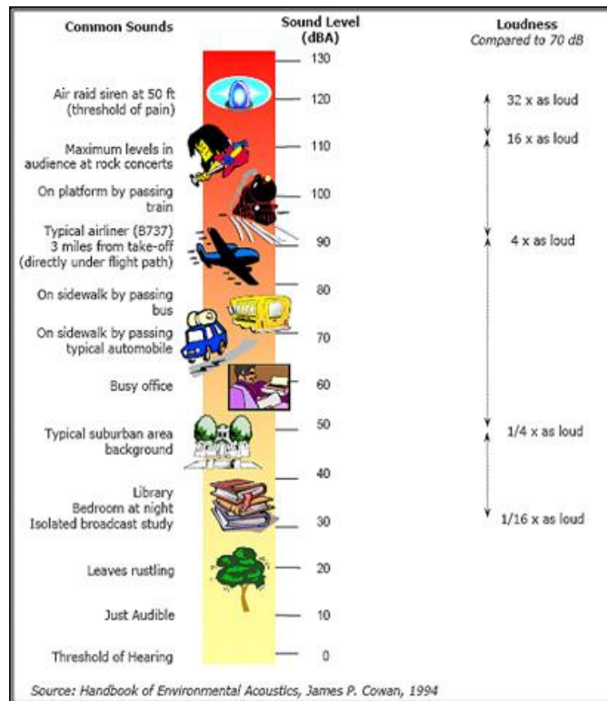
Figure 2 - Comparative Sound Levels
