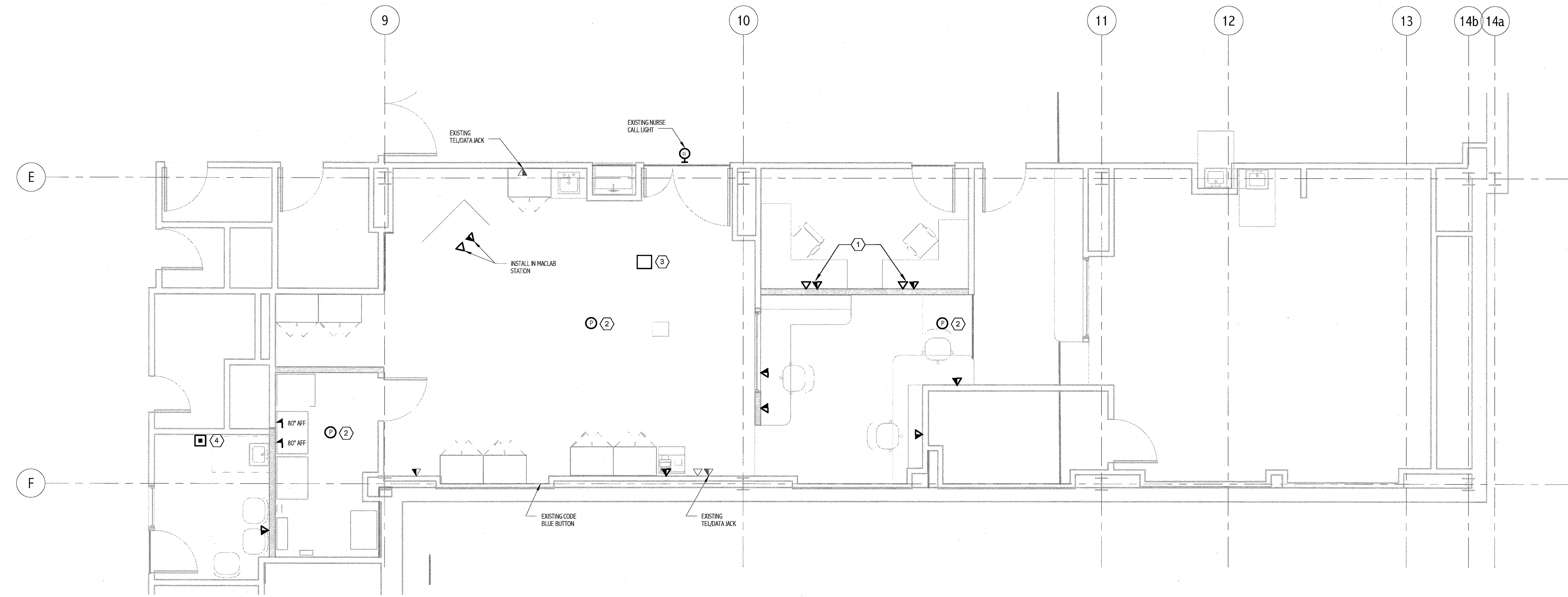
① CATH LAB #1 SYSTEMS PLAN 1/4" = 1'-0"
