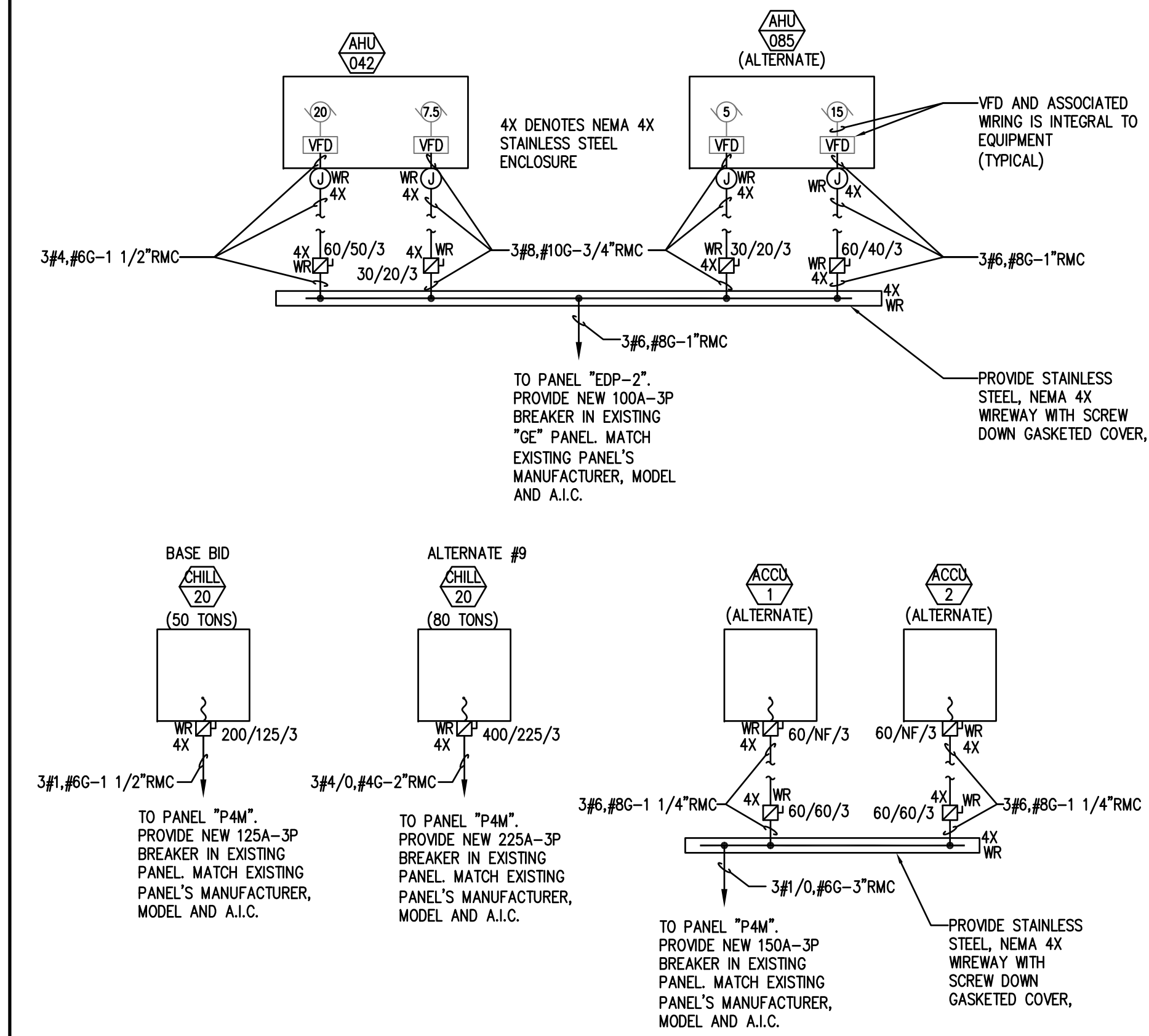
1 ROOF TOP WIRING DIAGRAMS SCALE: NOT TO SCALE
