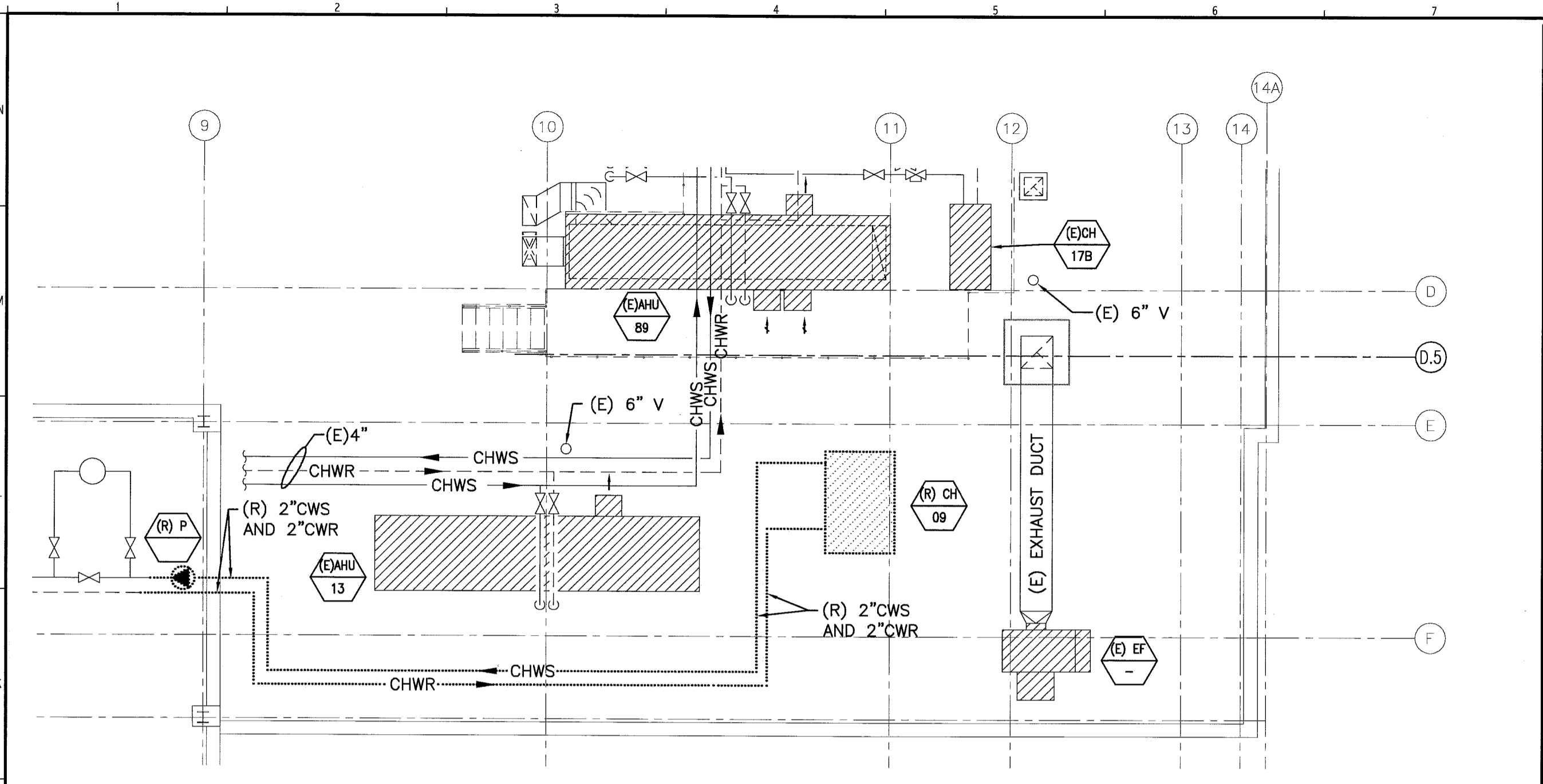
K1 MECHANICAL DEMOLITION ROOF PLAN
