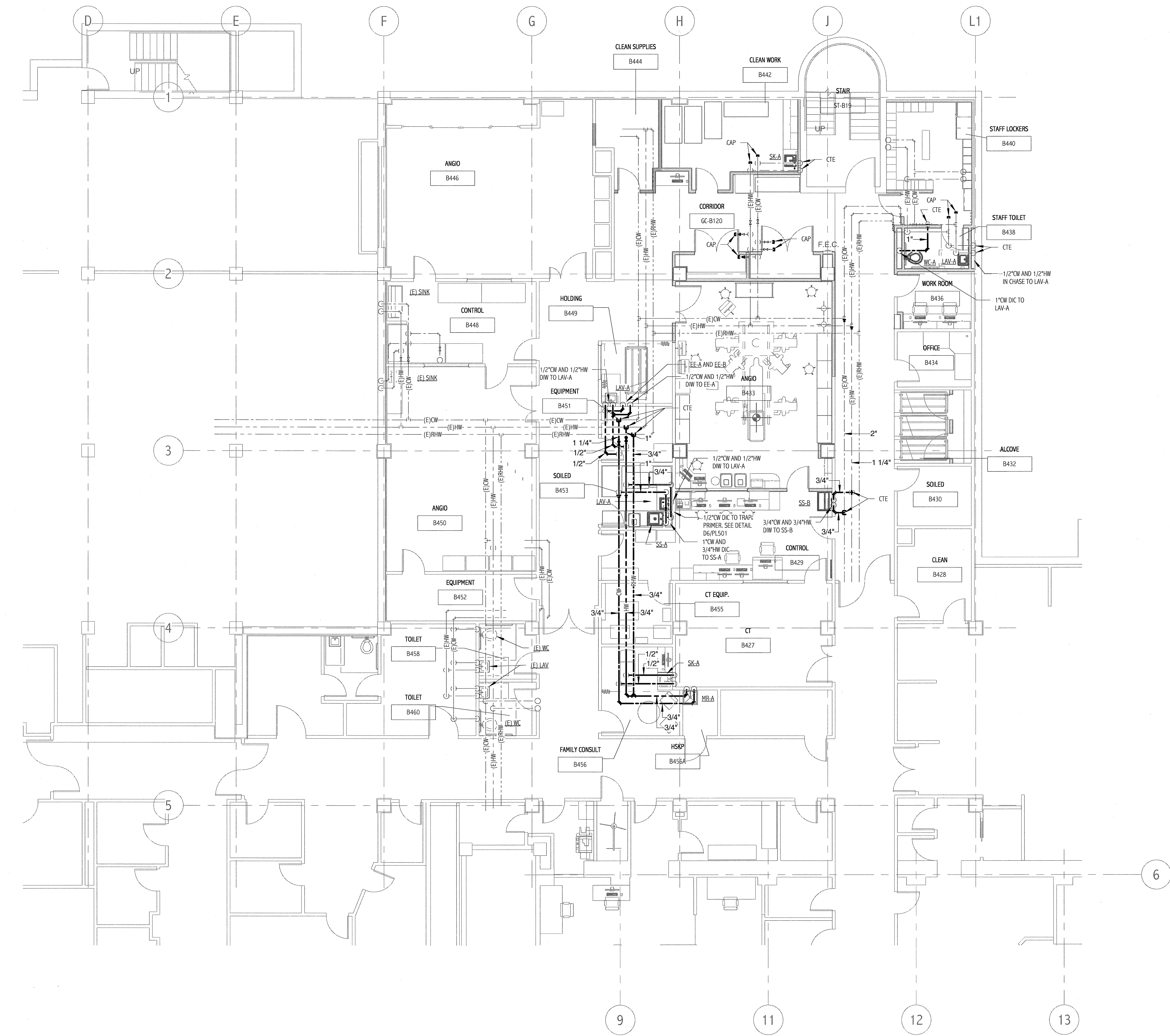
1 ANGIO DOMESTIC WATER PIPING PLAN 1/8" = 1'-0"
