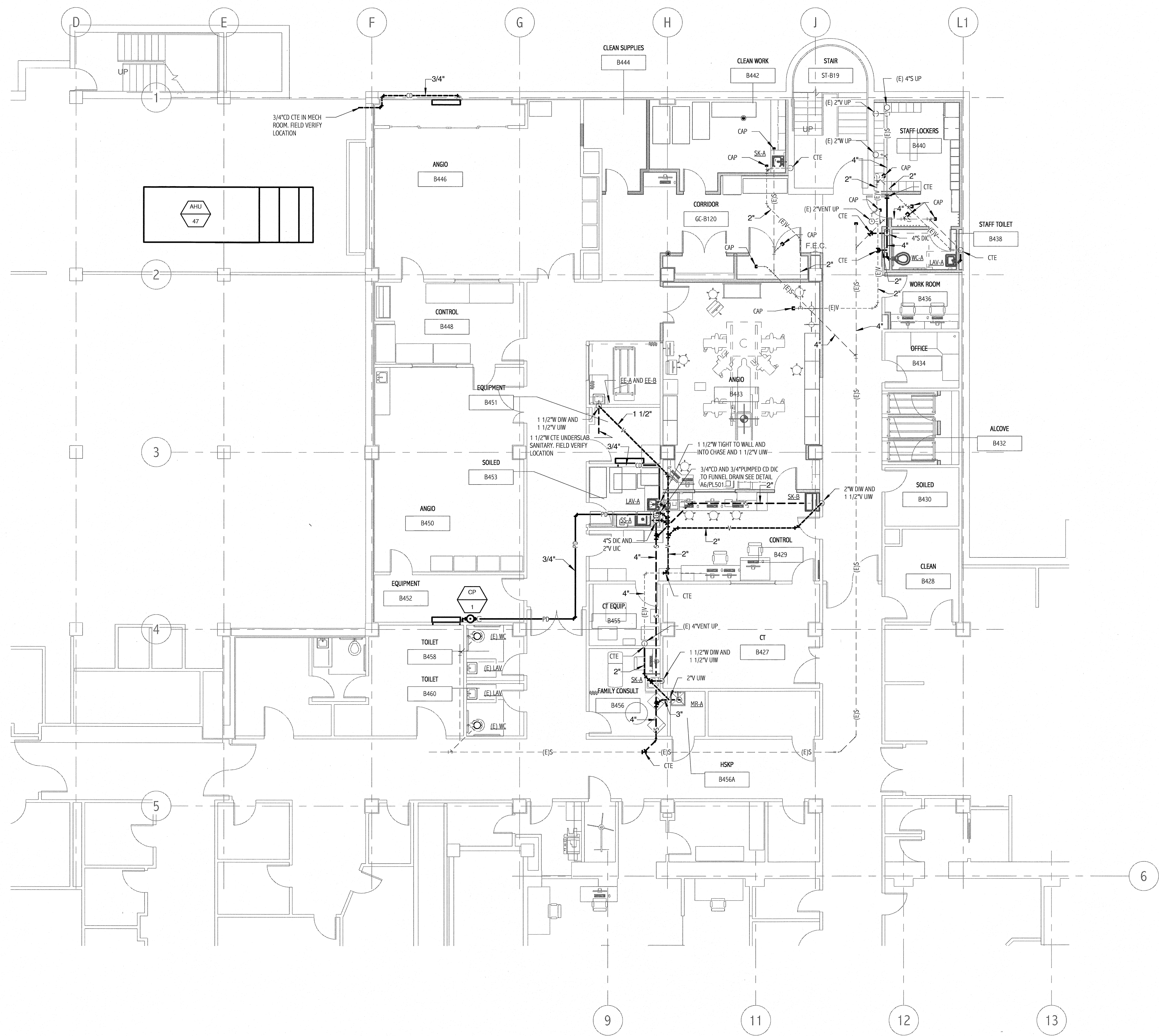
1 ANGIO SANITARY PIPING PLAN 1/8" = 1'-0"
