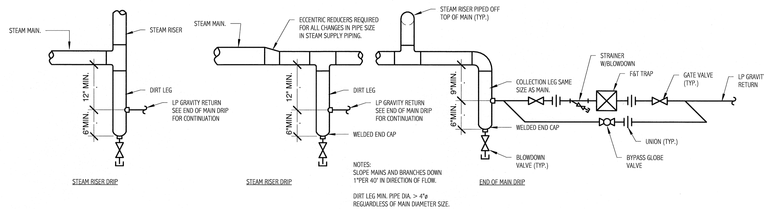
2 STEAM TRAP DETAILS NOT TO SCALE
