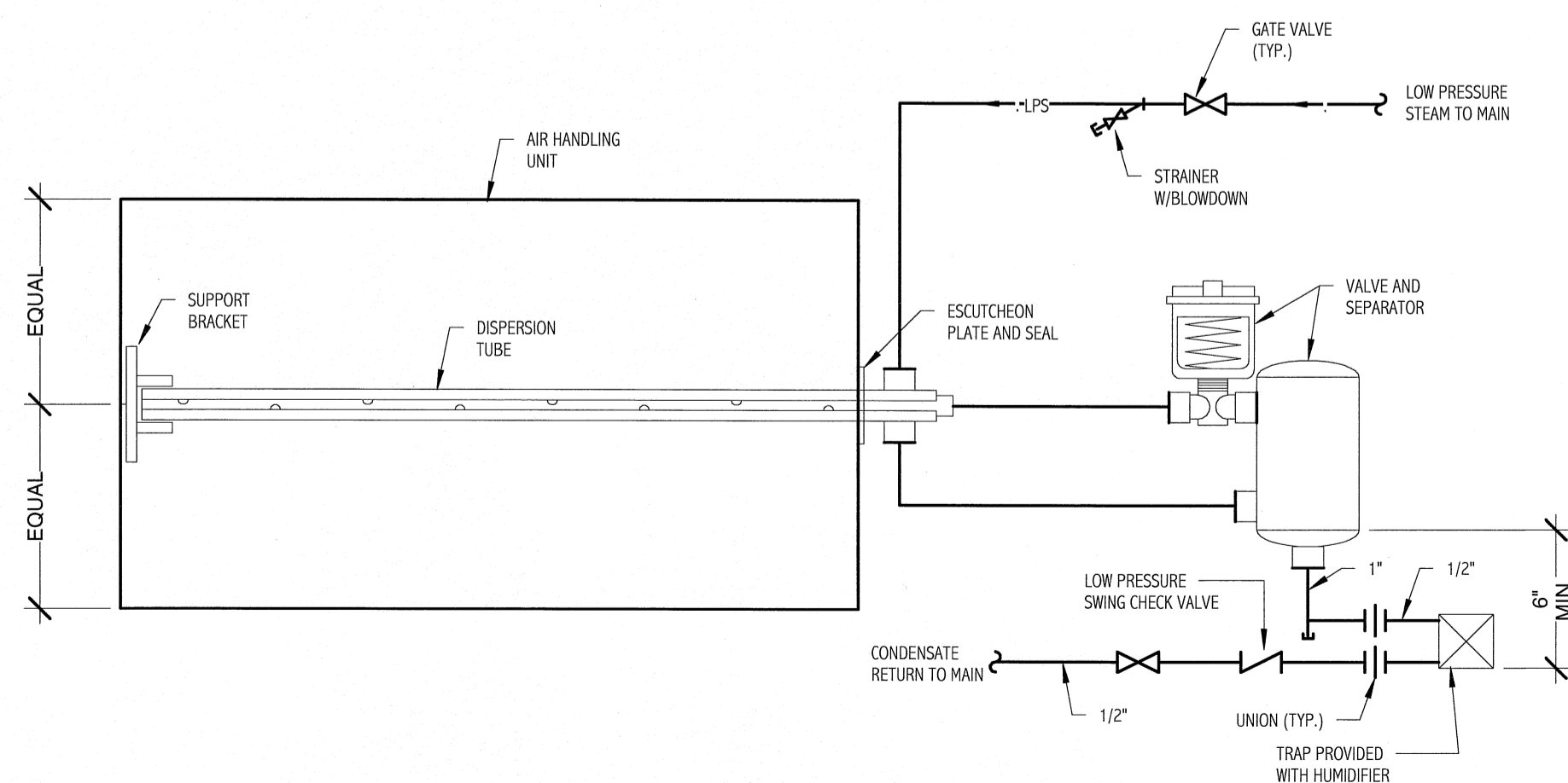
1 STEAM HUMIDIFIER DETAIL NOT TO SCALE
