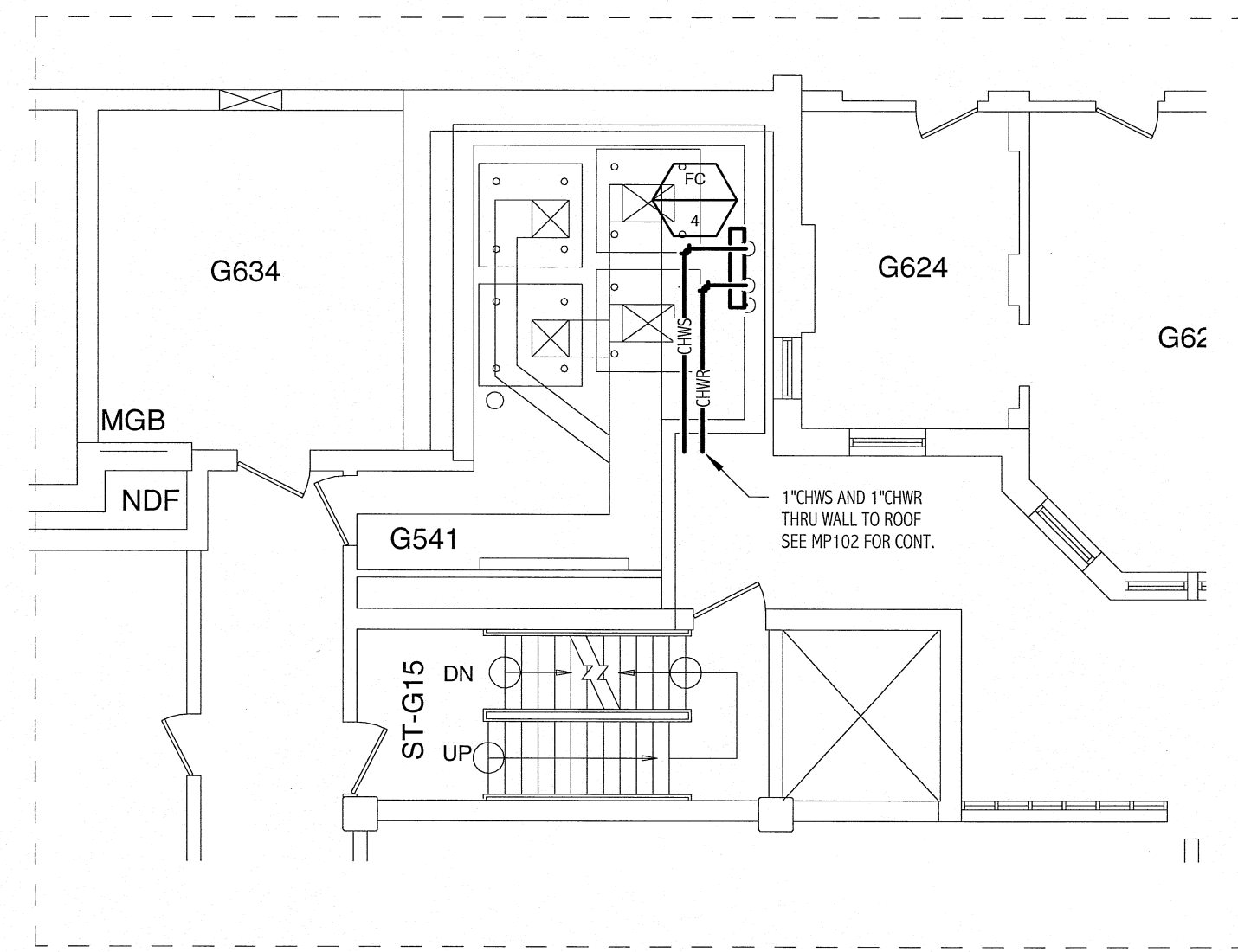
GROUND FLOOR UPS ROOM PIPING PLAN ② 1/8" = 1'-0"
