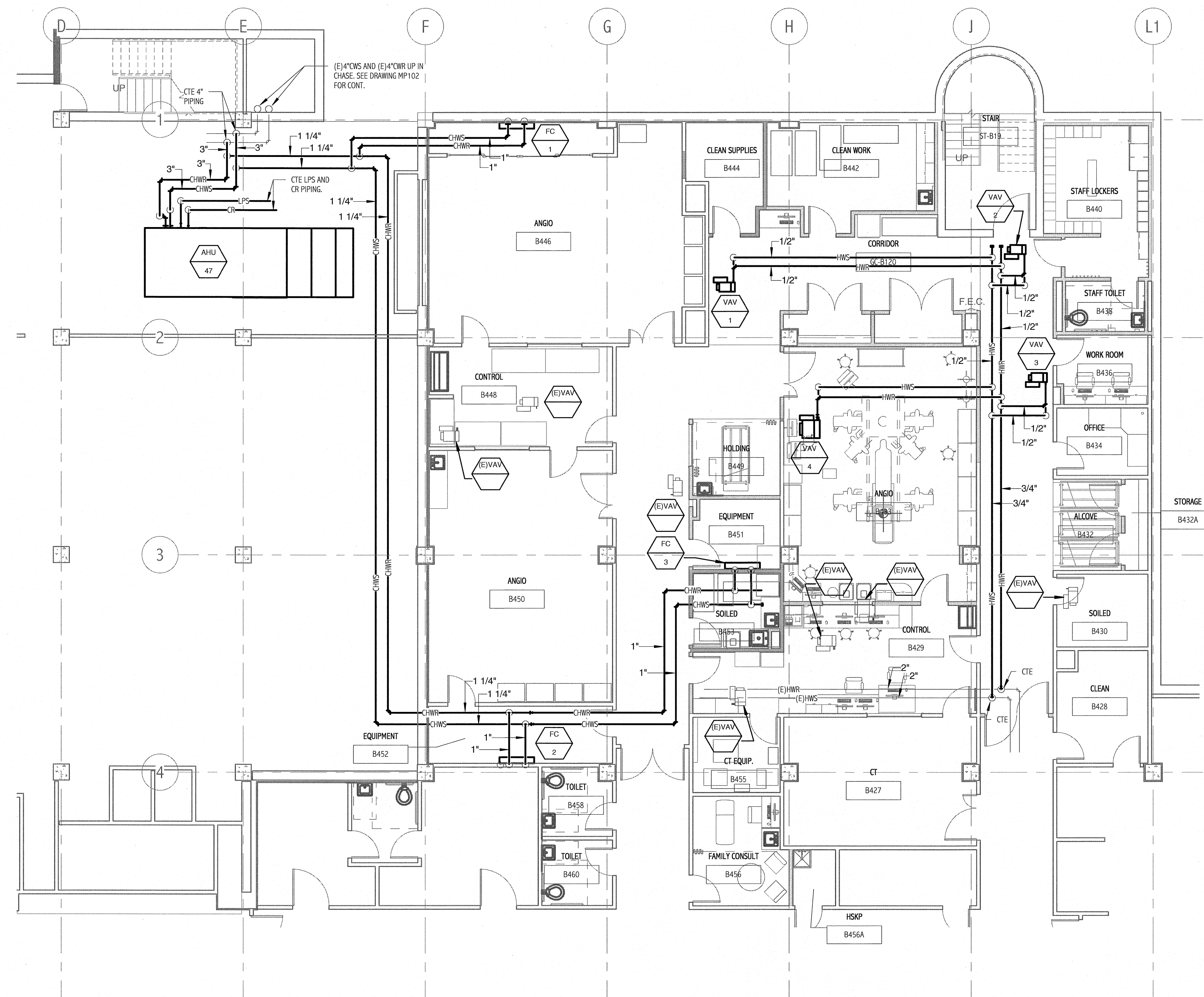
① ANGIO HVAC PIPING PLAN 1/8" = 1'-0"
