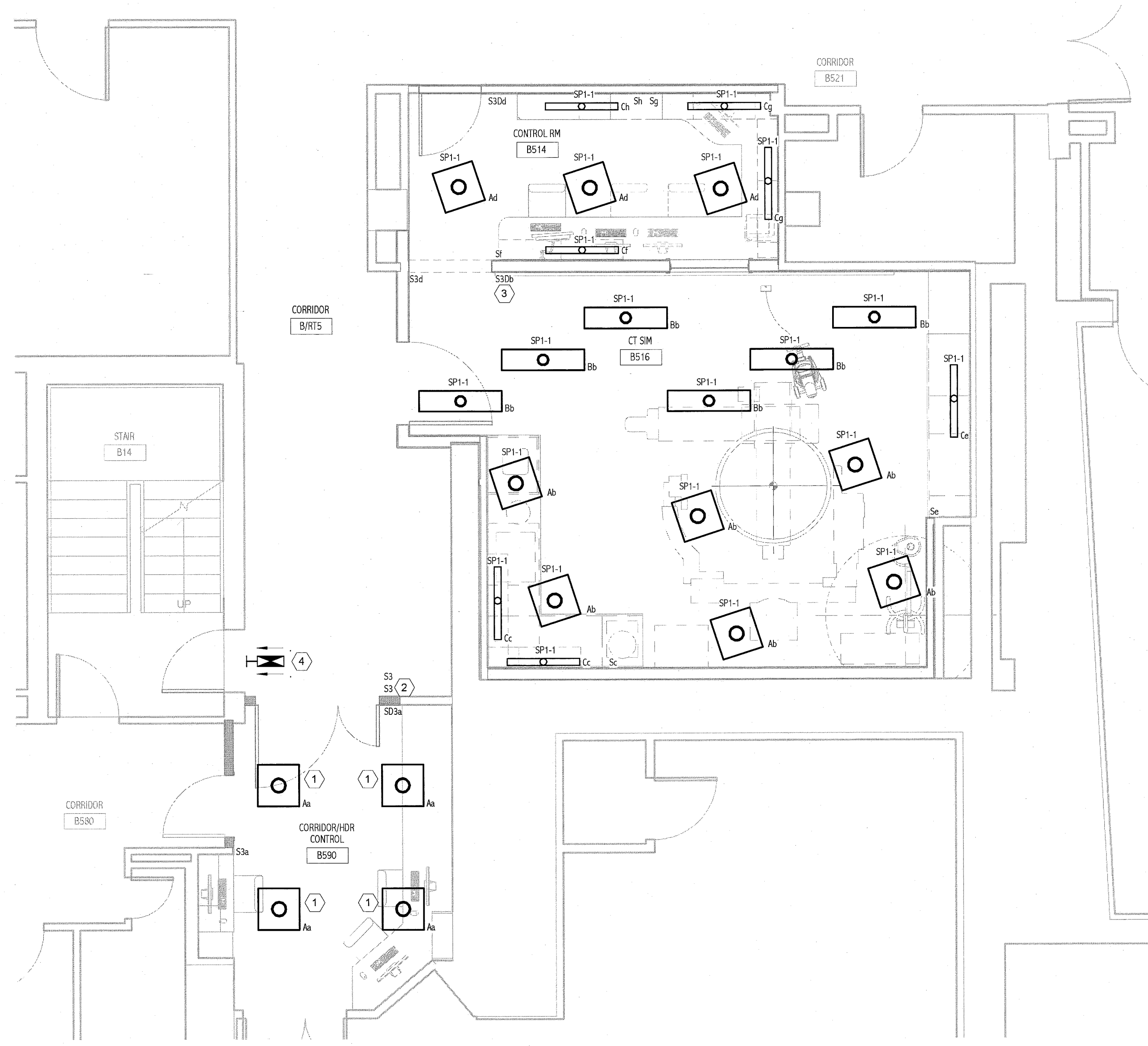
1 LIGHTING BASEMENT FLOOR PLAN 1/4" = 1'-0"
