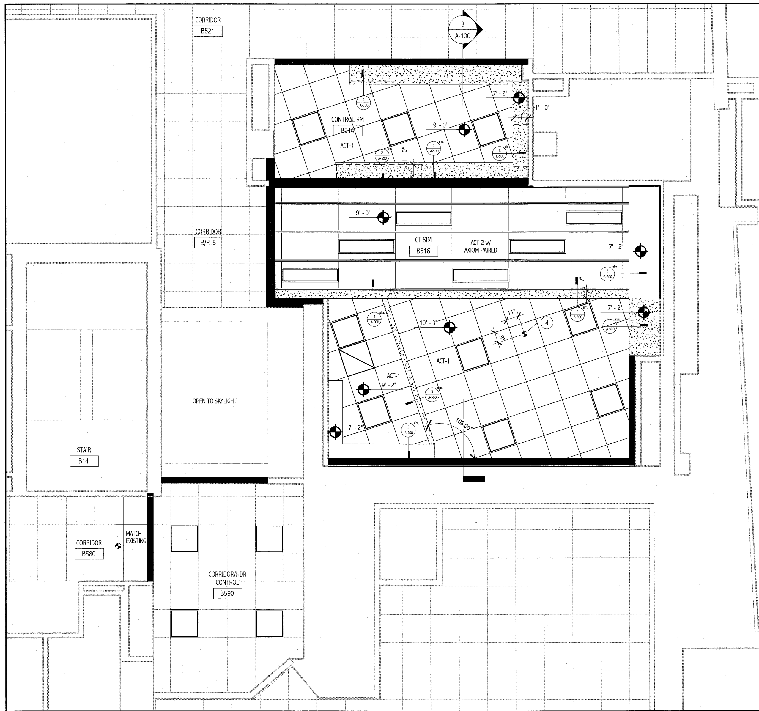
2 BASEMENT REFLECTED CEILING PLAN 1/4" = 1'-0"
