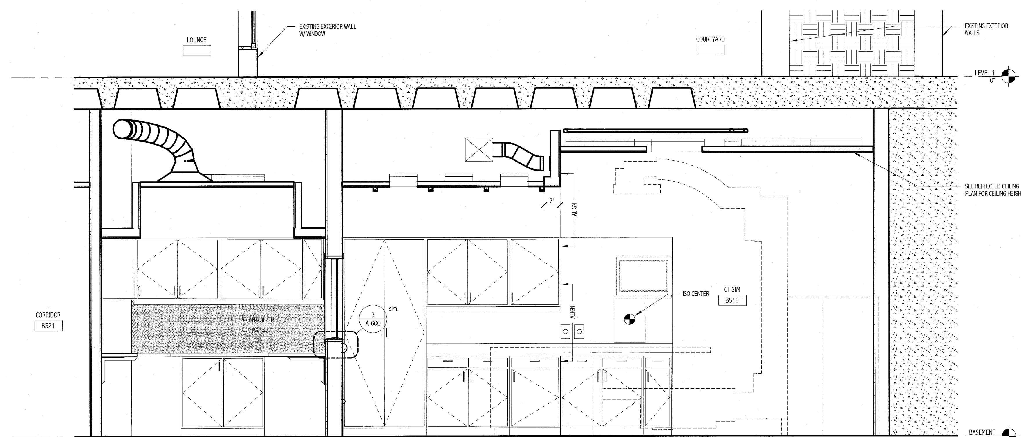
3 SECTION CT SIM 1/2" = 1'-0"
