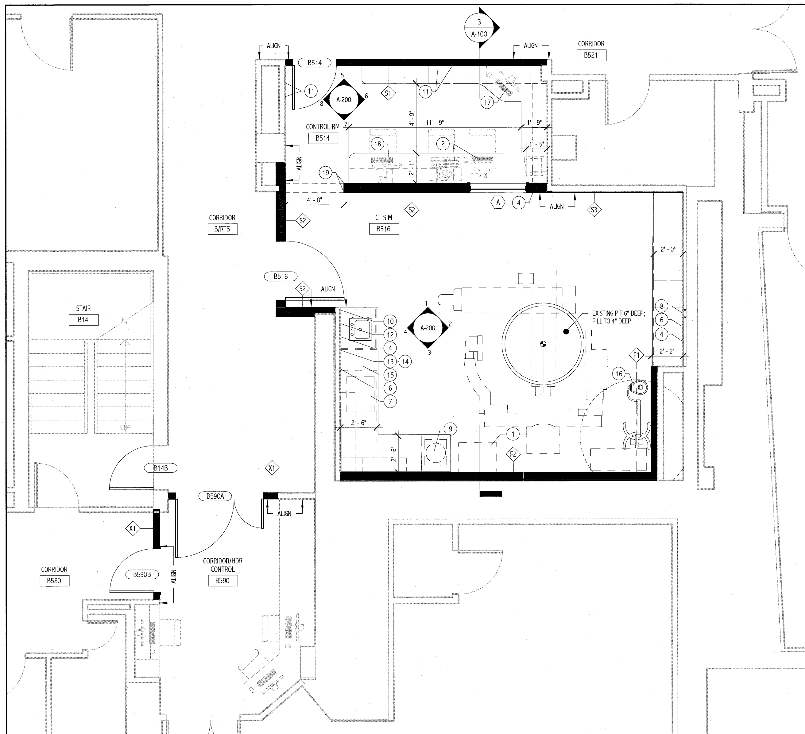
1 BASEMENT FLOOR PLAN 1/4" = 1'-0"
