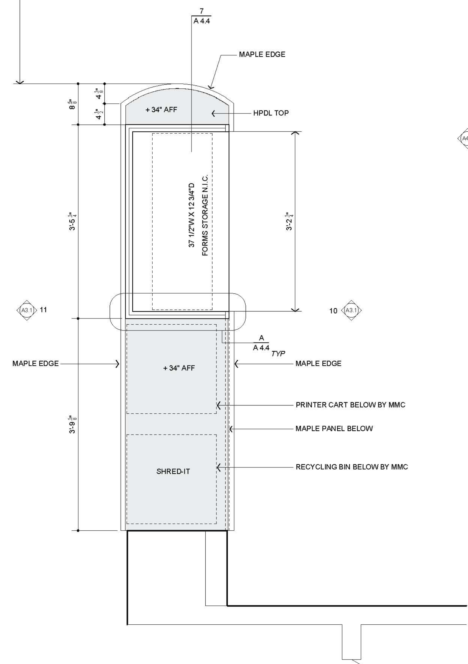
A CHARTING AREA PLAN 1"= 1'-0"
