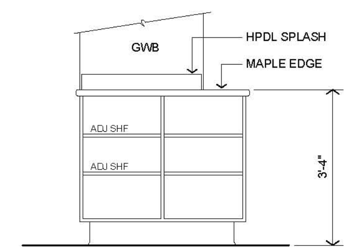
2 CHARTING ISLAND: EAST 1/2"= 1'-0"
