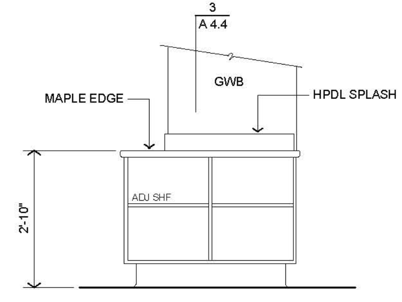
4 CHARTING ISLAND: WEST 1/2"= 1'-0"
