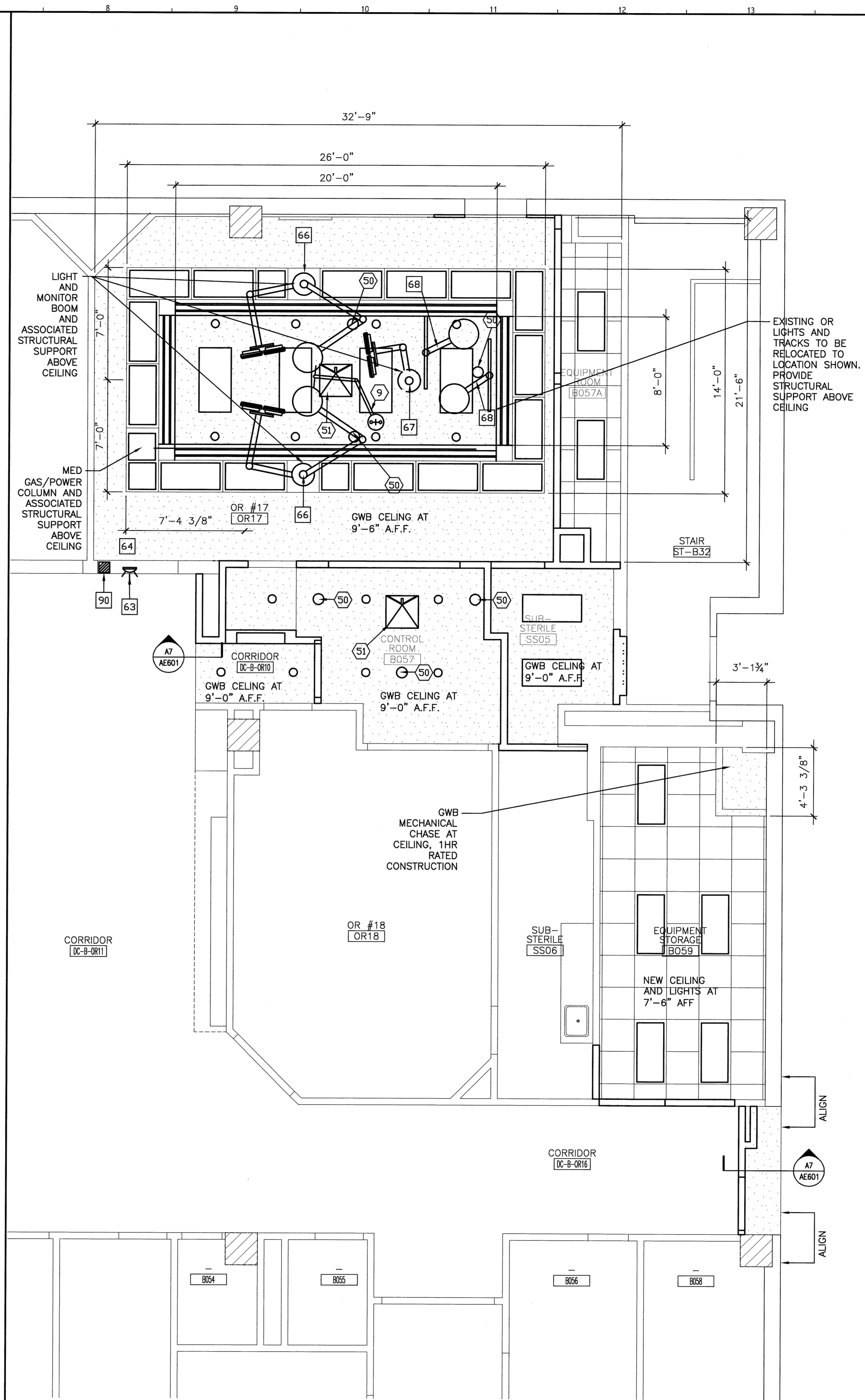
A7 REFLECTED CEILING PLAN 1/4" = 1'-0"
