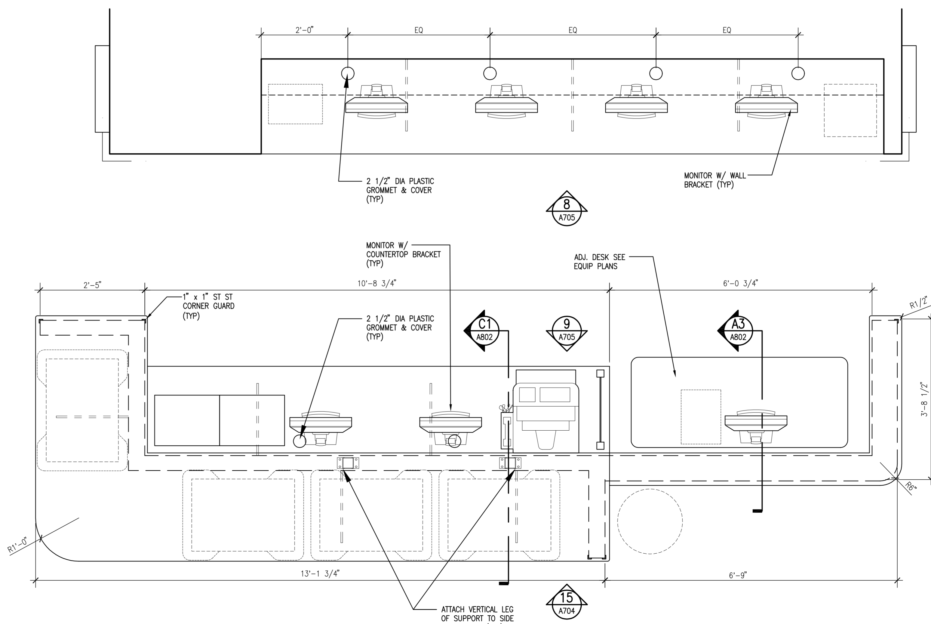
4 ENLARGED PLAN WORK STATION #B261-ER SCALE: 3/4" = 1'-0"
