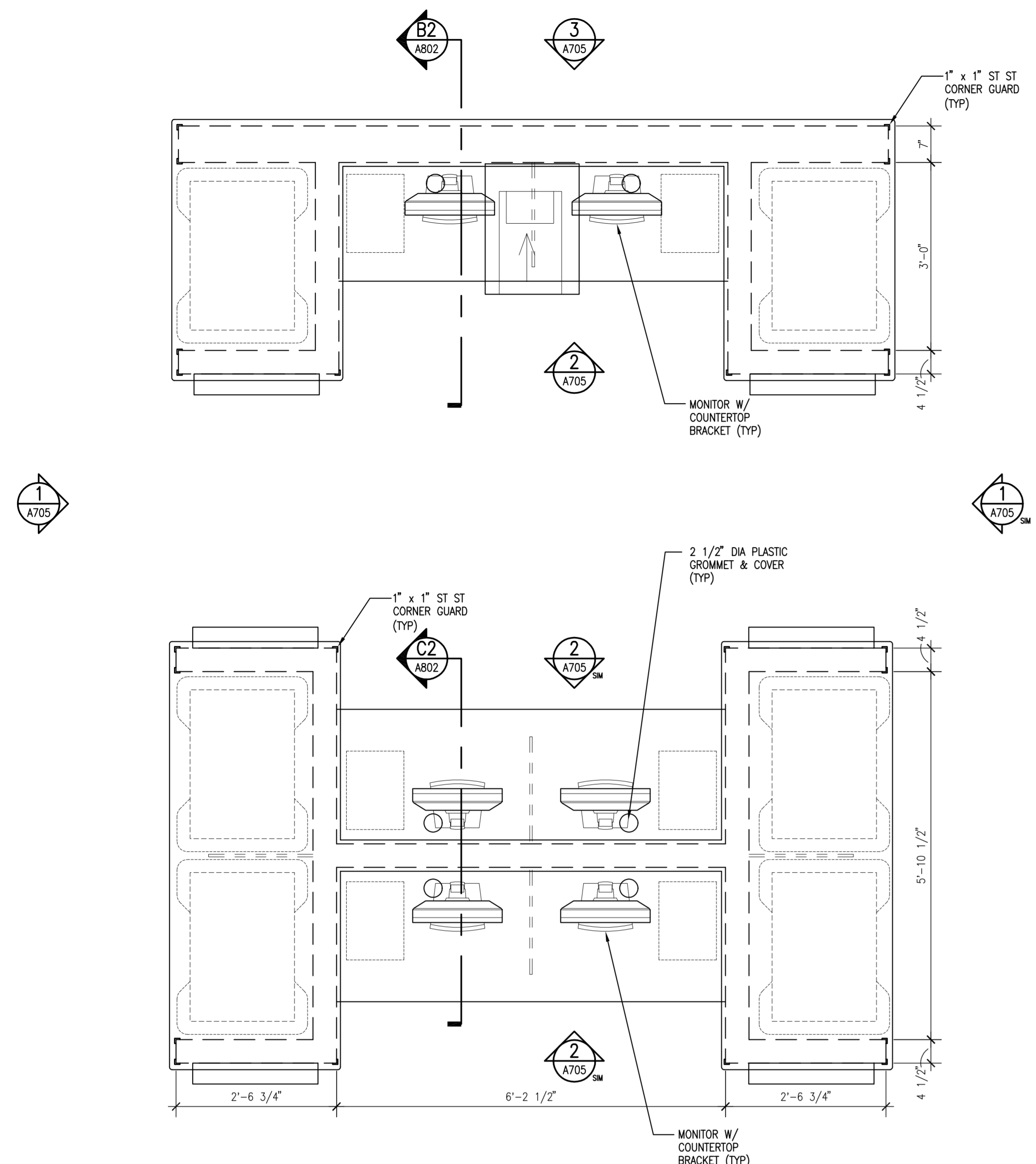
1 ENLARGED PLAN WORK STATION #B523-ER, #B522-ER SCALE: 3/4" = 1'-0"
