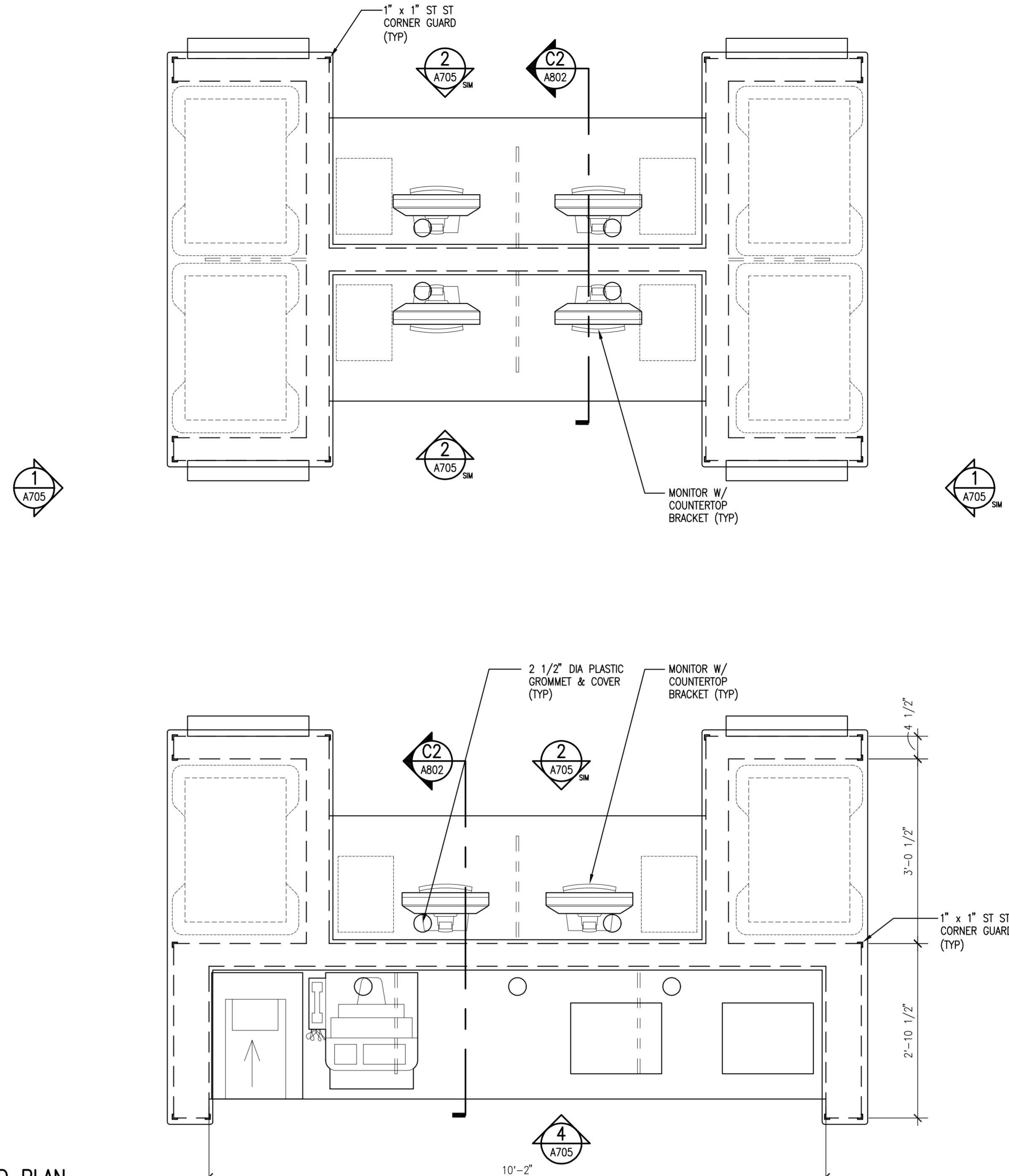
2 ENLARGED PLAN WORK STATION #B526-ER, #B525-ER, #B524-ER SCALE: 3/4" = 1'-0"
