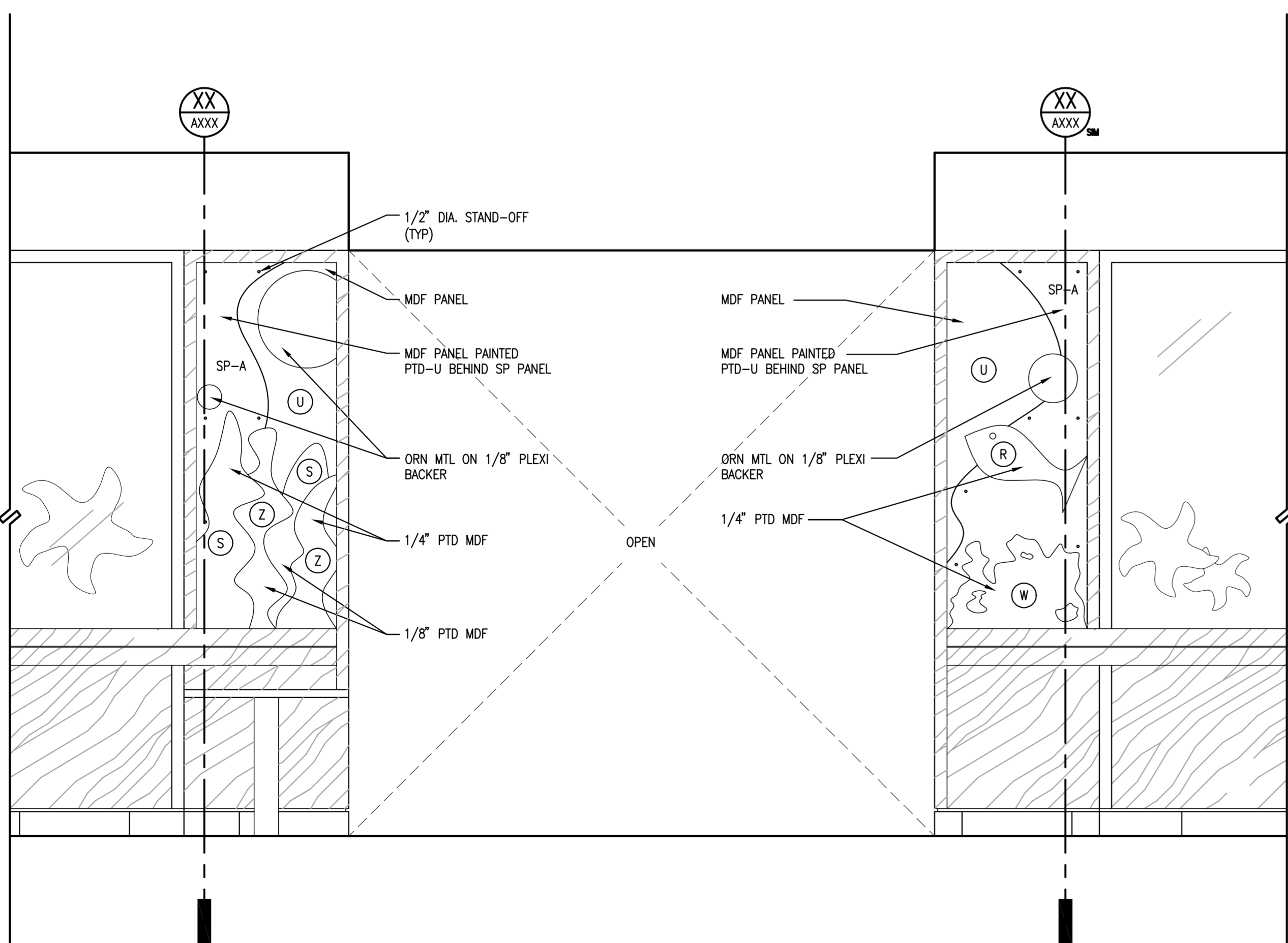
3 ENLARGED ELEVATION PEDIATRIC WAITING #B007-ER SCALE: 3/4" = 1'-0"
