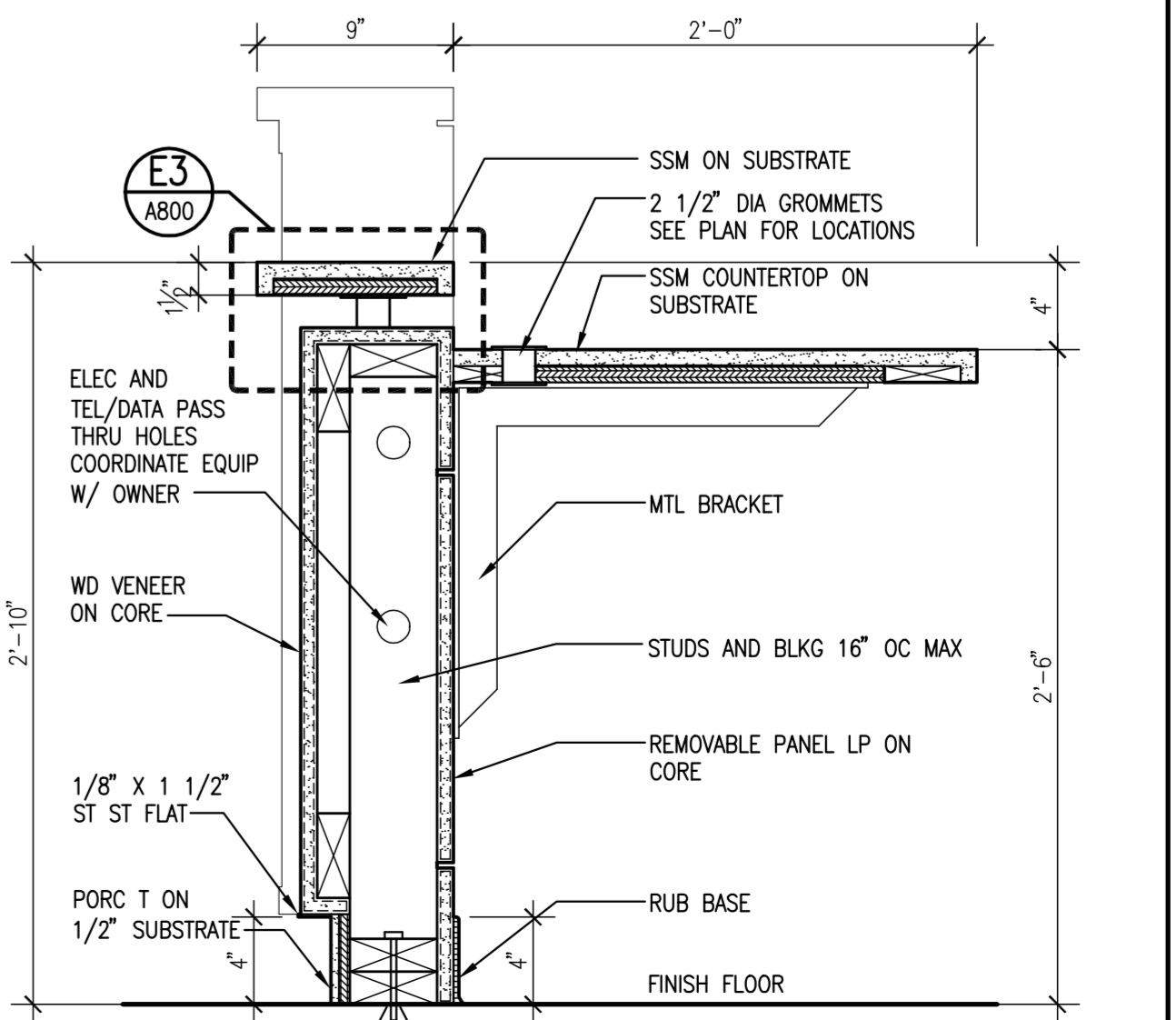
E4 SECTION AT RECEPTION - ADA HEIGHT SCALE: 1 1/2" = 1'-0"
