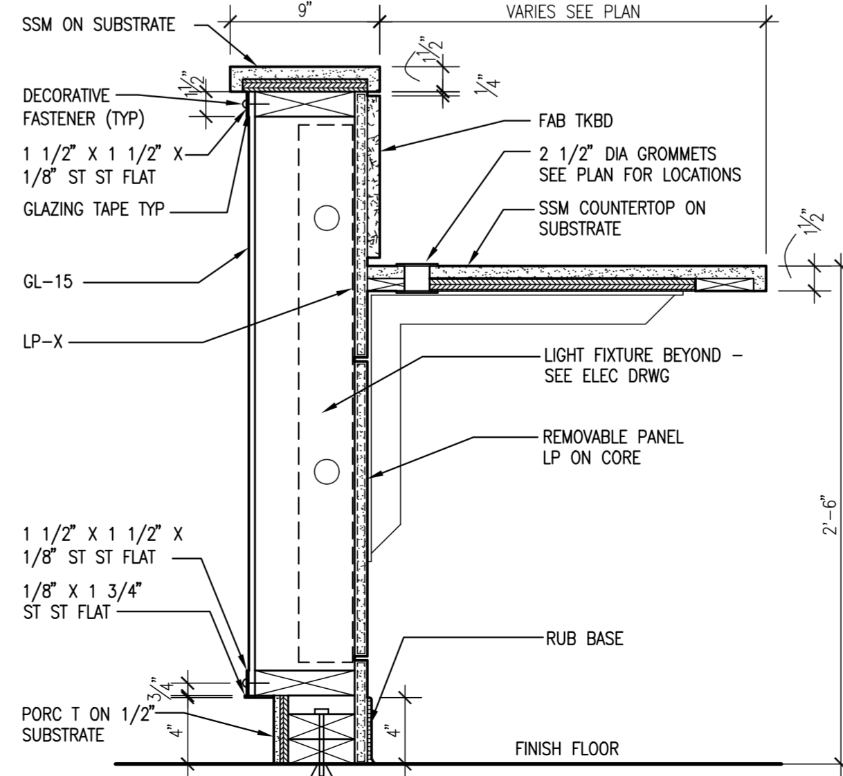
D4 SECTION AT RECEPTION SCALE: 1 1/2" = 1'-0"
