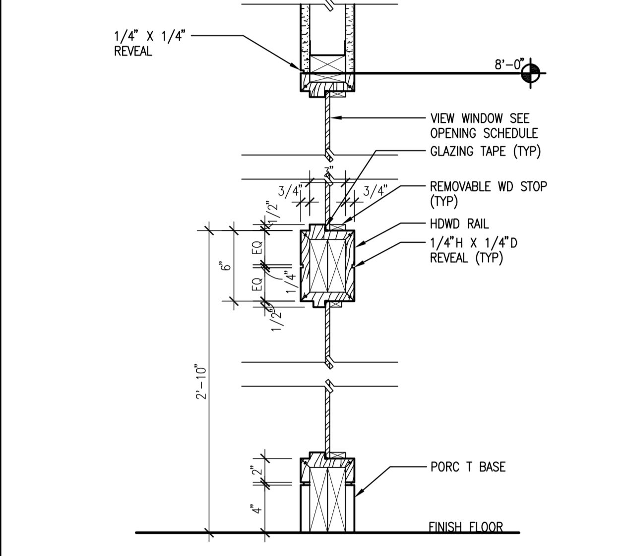
A2 WOOD FRAMED BORROWED LIGHT SCALE: 1 1/2" = 1'-0"
