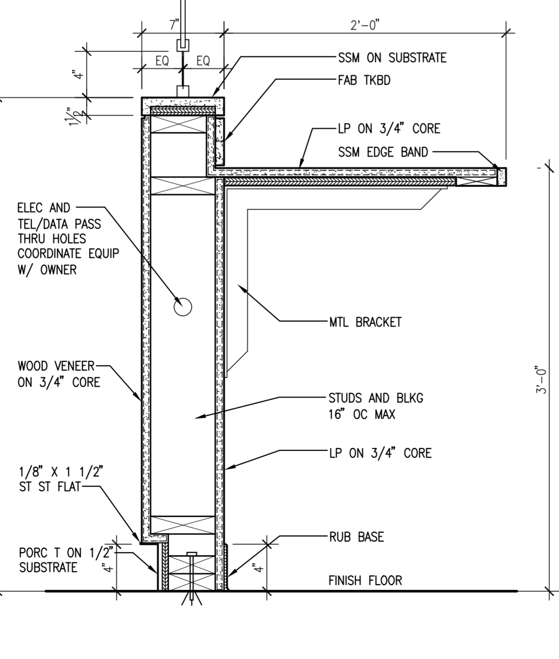
B4 REGISTRATION WORK STATION SCALE: 1 1/2" = 1'-0"
