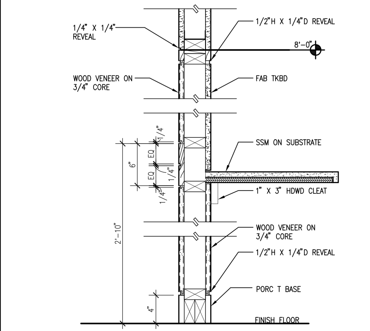
A4 WOOD/FABRIC WRAPPED PANEL AT TELEPHONE SCALE: 1 1/2" = 1'-0"
