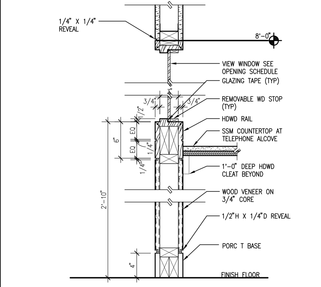
A3 WOOD FRAMED BORROWED LIGHT SCALE: 1 1/2" = 1'-0"
