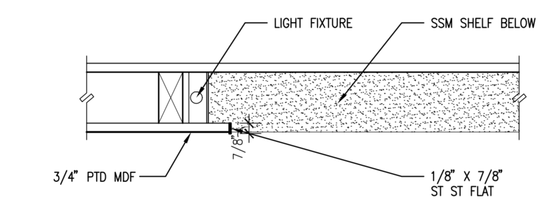
C2 WALL AT MAIN RECEPTION DESK - PART. PLAN SCALE: 1 1/2" = 1'-0"
