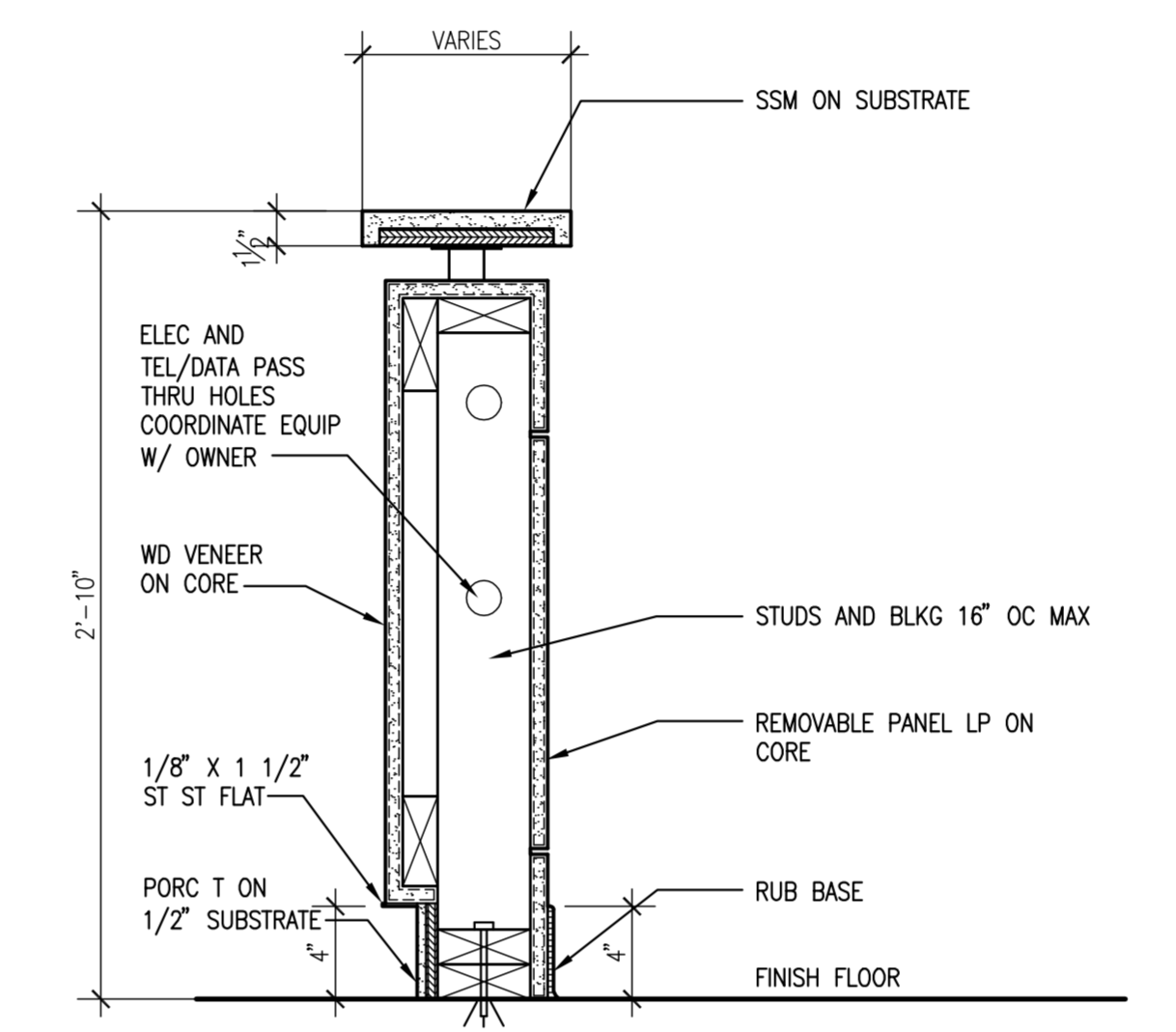
D2 SECTION AT PEDIATRIC RECEPTION SCALE: 1 1/2" = 1'-0"
