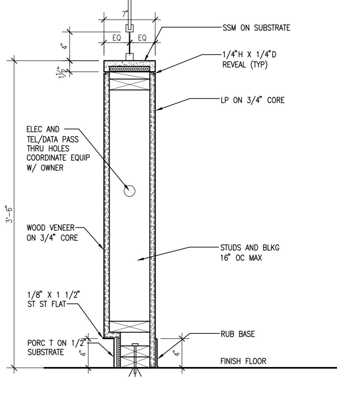
C4 WHEELCHAIR ALCOVE SCALE: 1 1/2" = 1'-0"
