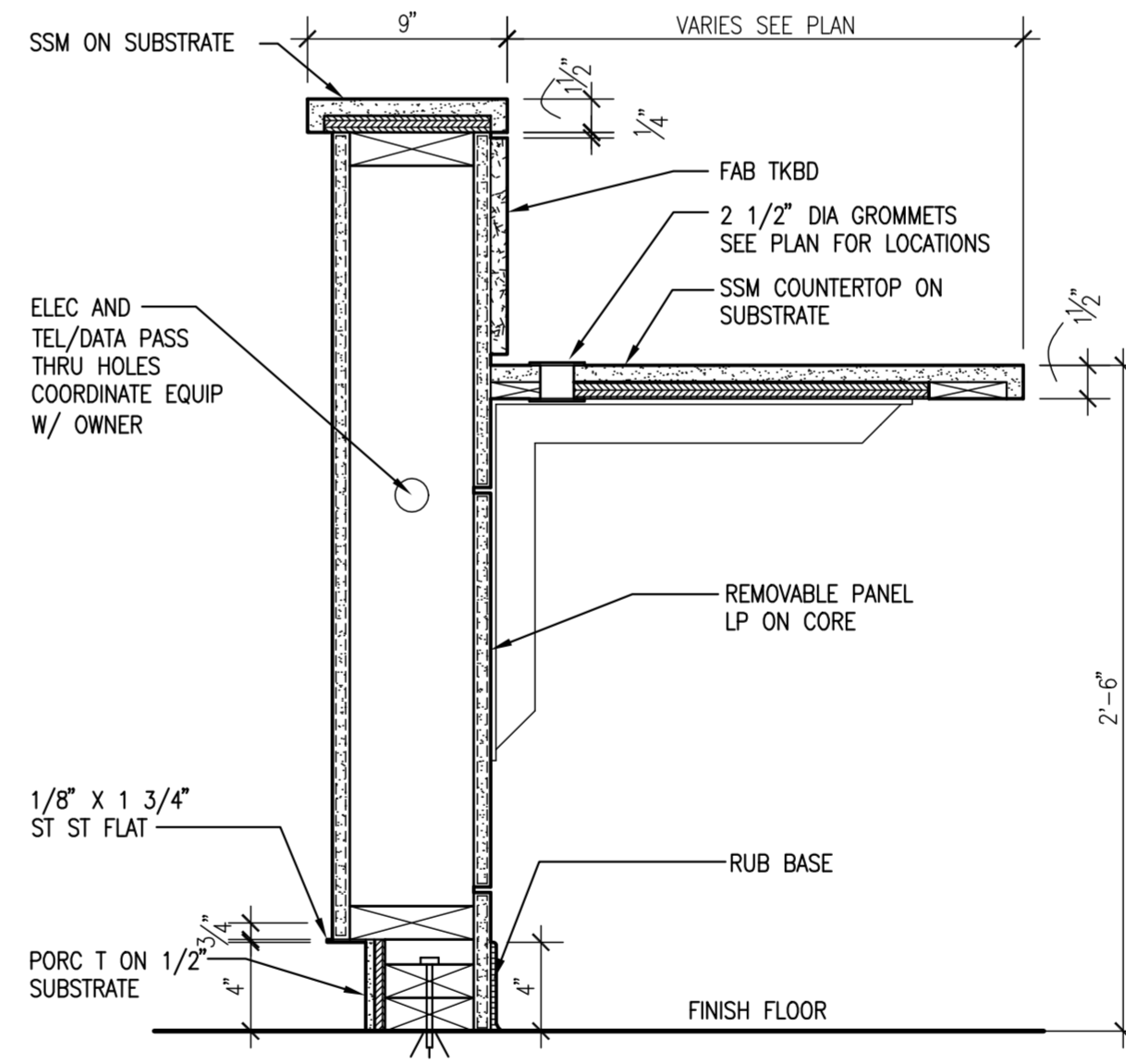
D3 SECTION AT RECEPTION SCALE: 1 1/2" = 1'-0"
