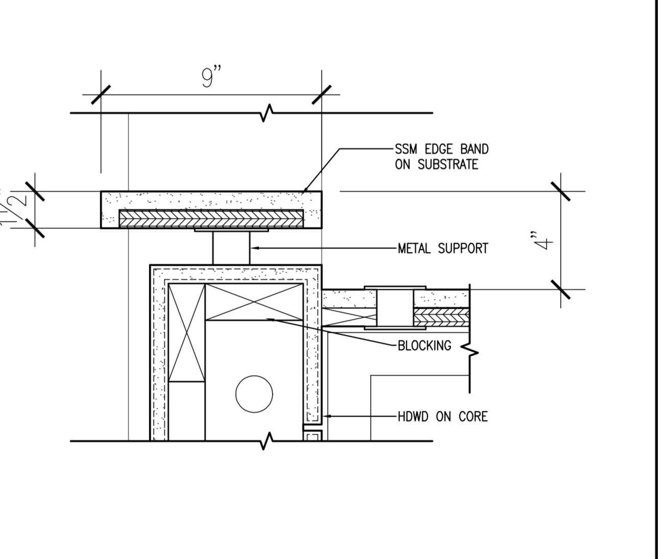
E3 SECTION - STAFF STATION SCALE: 3" = 1'-0"
