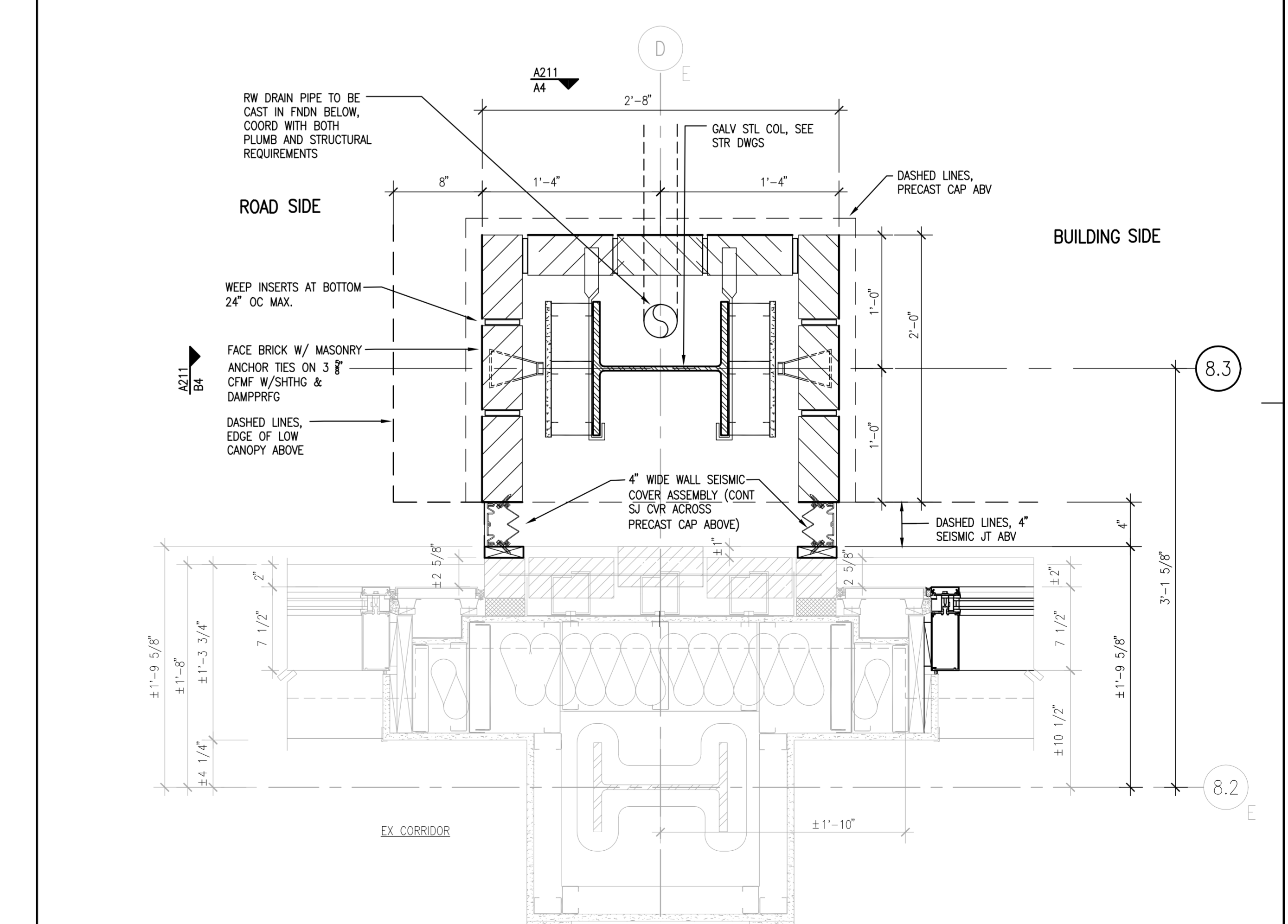
D3 MAIN ED CANOPY TYP PLAN DETAIL AT BRICK ENCLOSURE SCALE: 1 1/2" = 1'-0"
