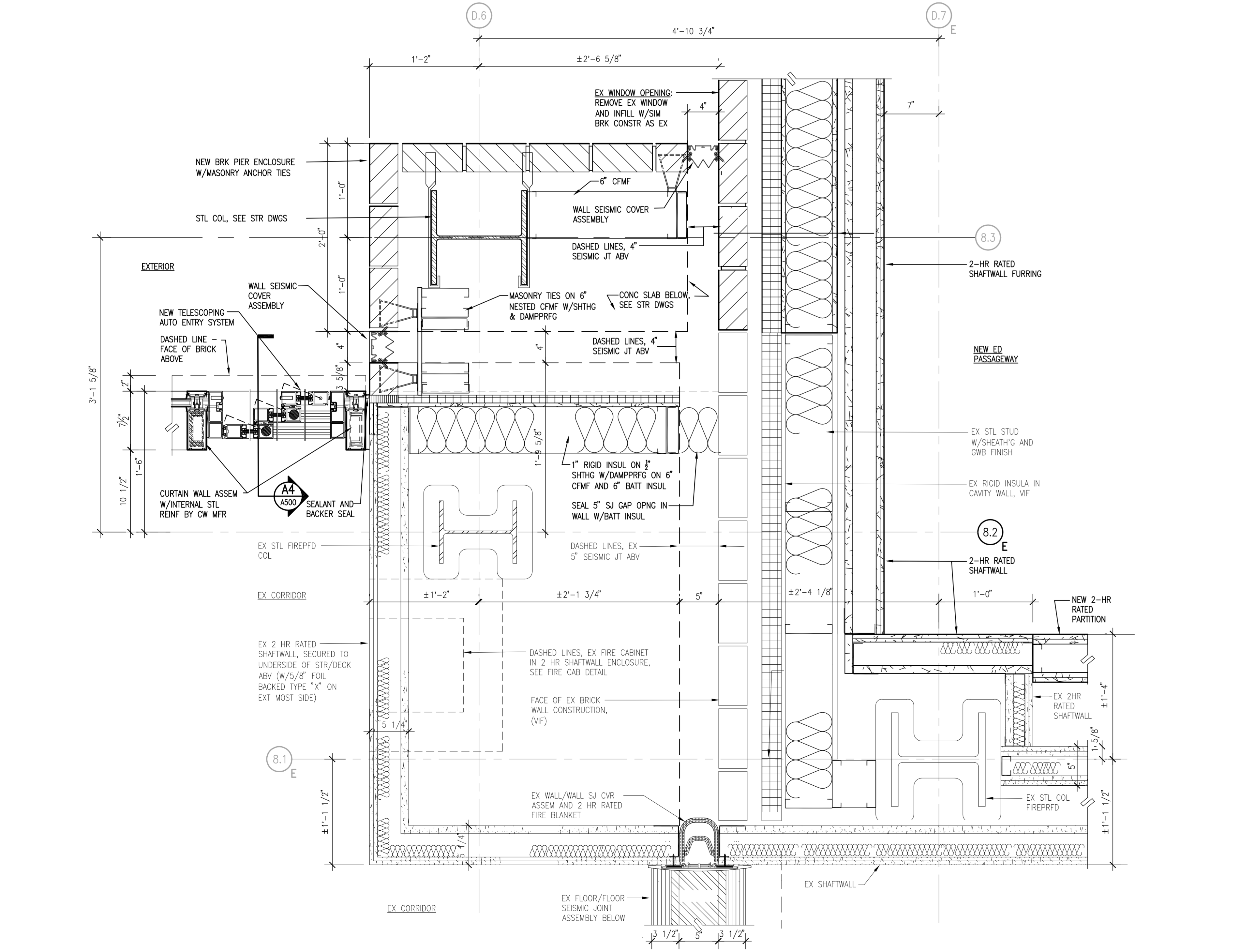
D3 MAIN ED CANOPY TYP PLAN DETAIL AT BRICK ENCLOSURE SCALE: 1 1/2" = 1'-0"
