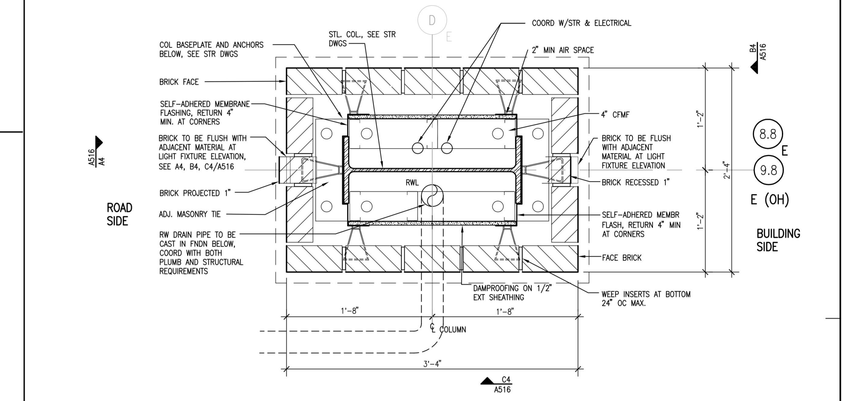
D3 MAIN ED CANOPY TYP PLAN DETAIL AT BRICK ENCLOSURE SCALE: 1 1/2" = 1'-0"
