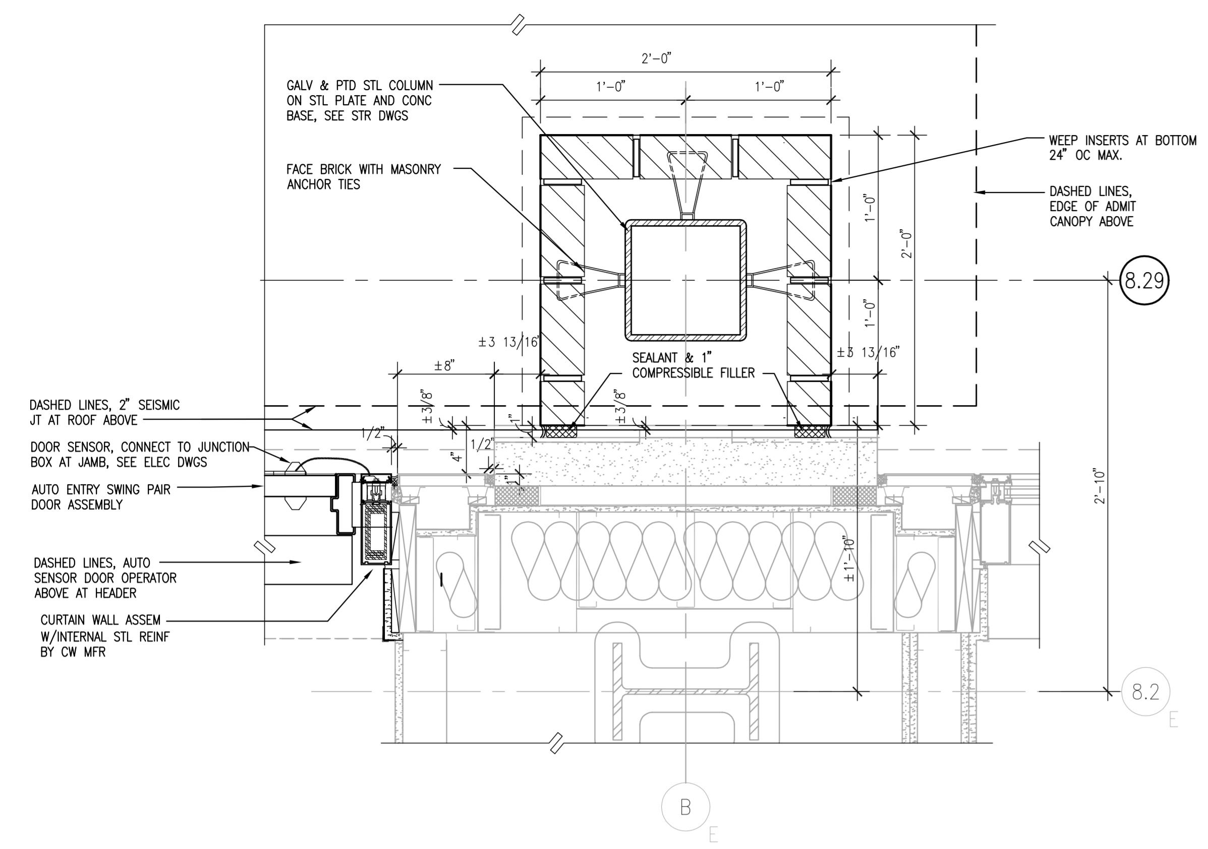
A1 ALTERNATE #2 - DIRECT ADMIT CANOPY PLAN DETAIL AT BRICK COL ENCLOSURE SCALE: 1 1/2" = 1'-0"
