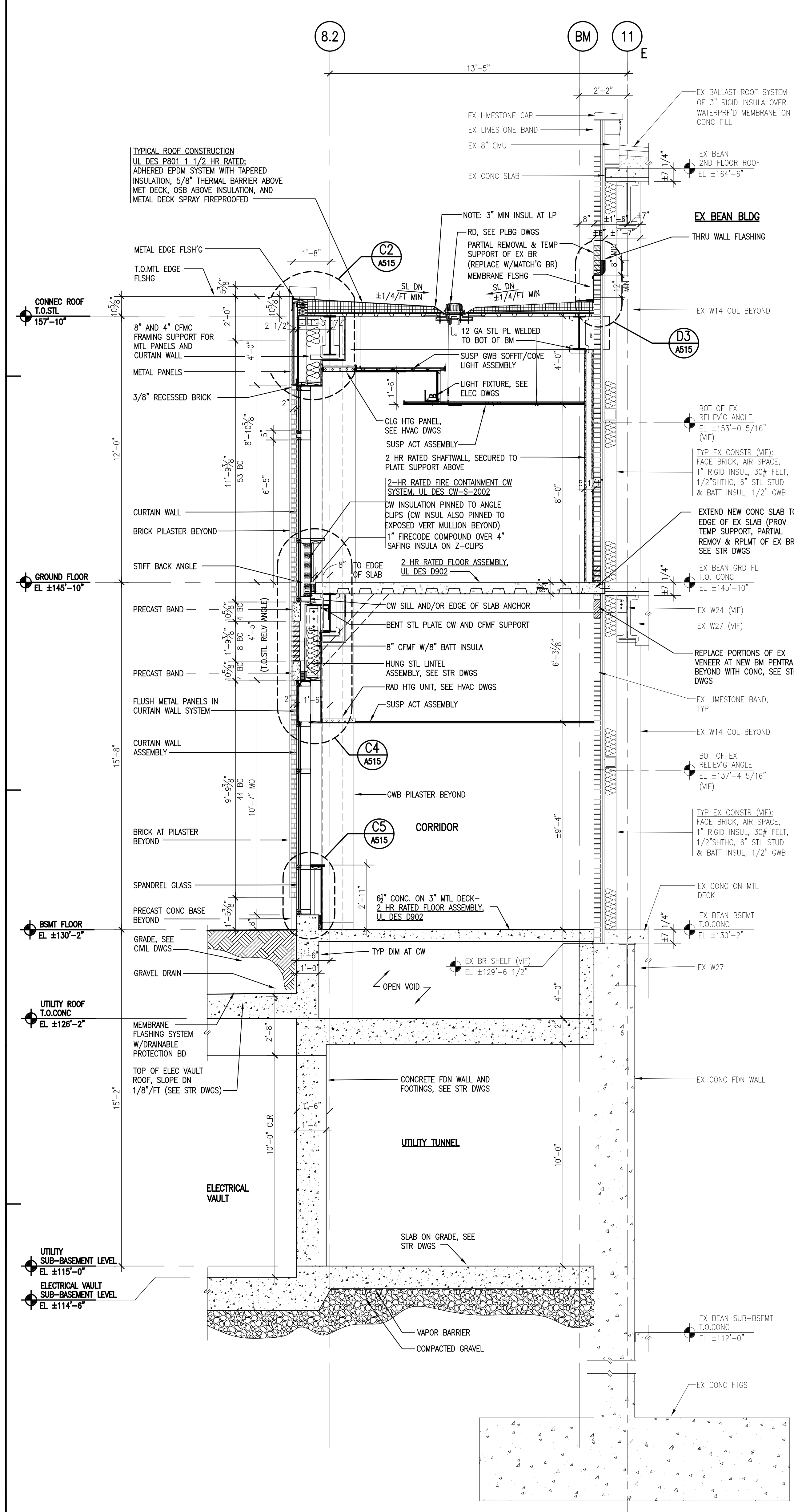
A5 NORTH CORRIDOR LINK WALL SECTION AT CW SCALE: 3/8" = 1'-0"
