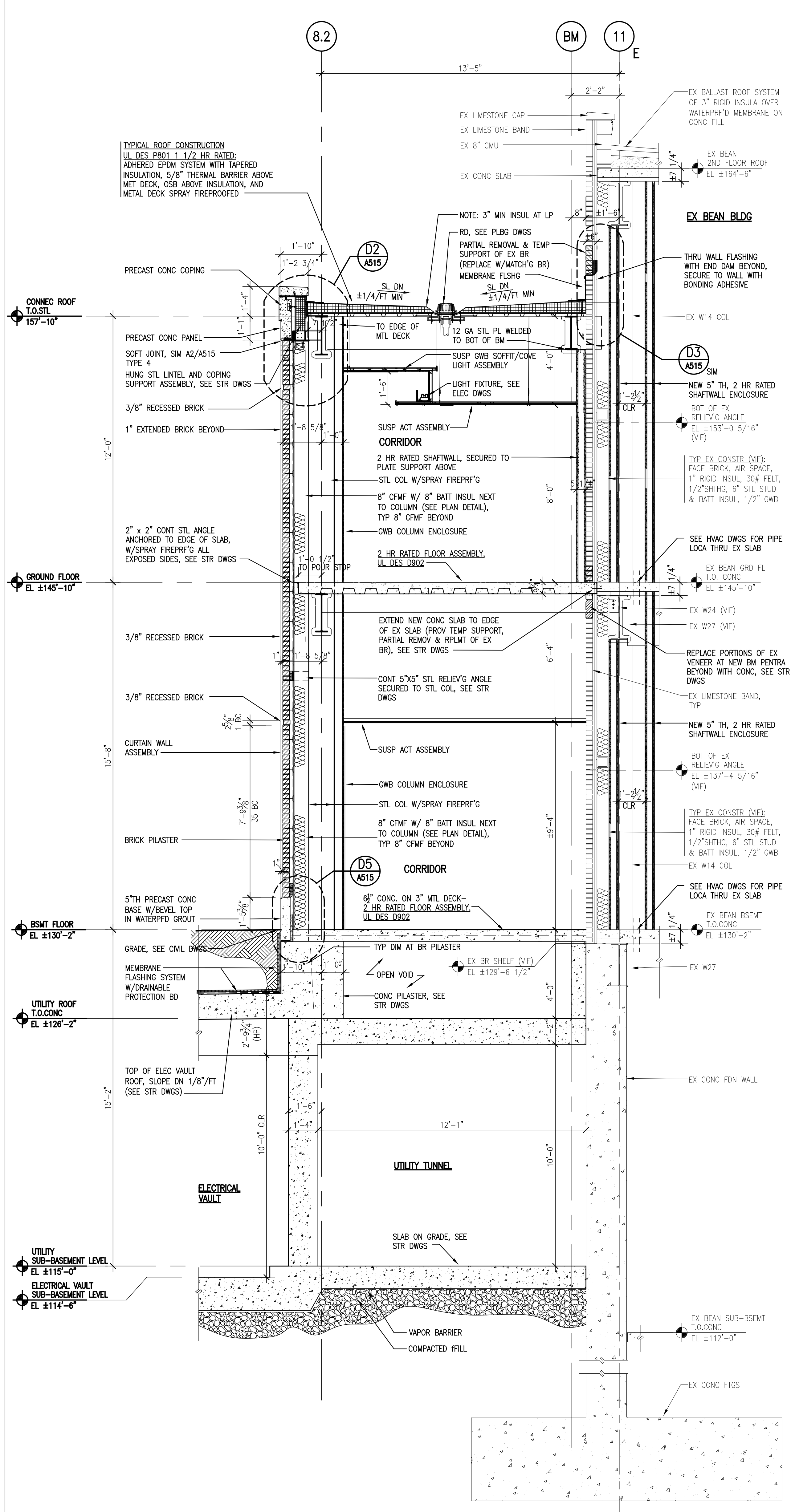
C5 NORTH CORRIDOR LINK WALL SECTION AT BRICK PILASTER SCALE: 3/8" = 1'-0"
