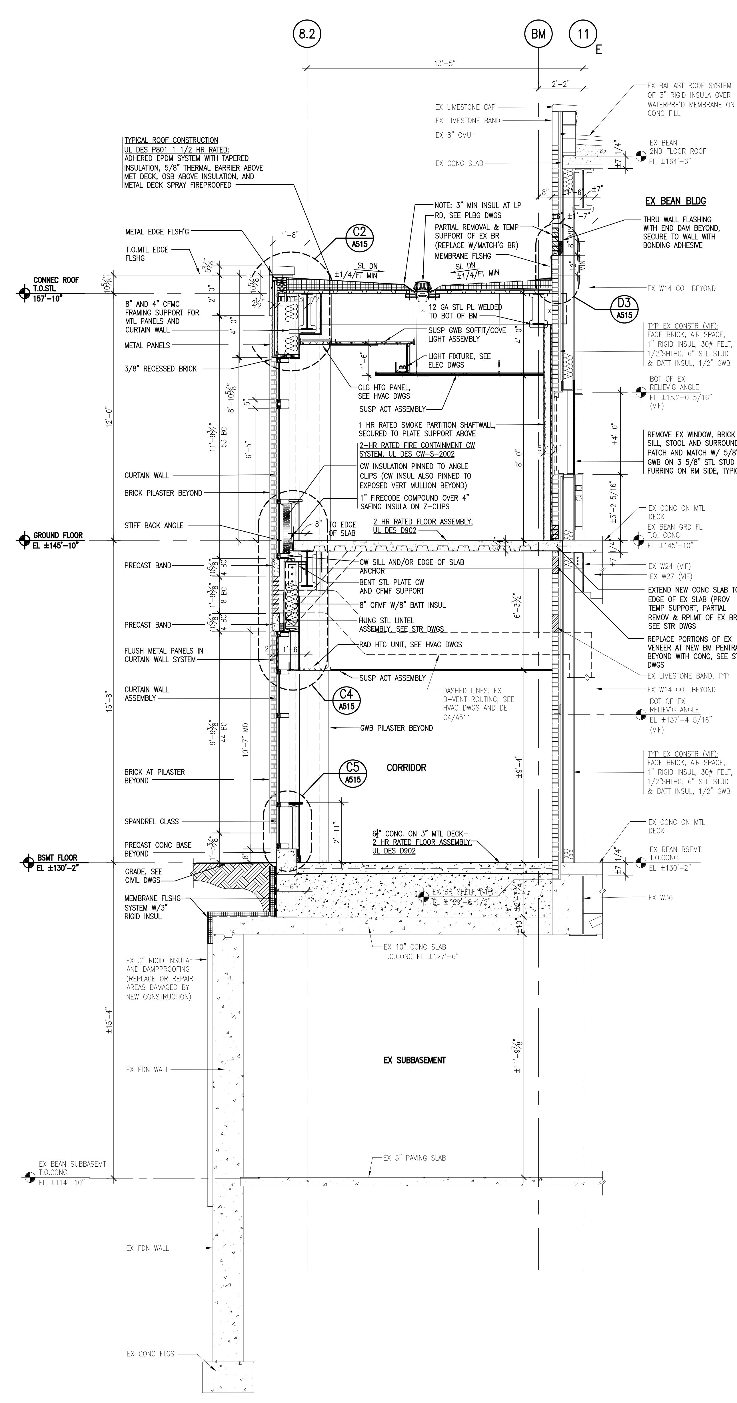
E5 NORTH CORRIDOR LINK WALL SECTION AT CW SCALE: 3/8" = 1'-0"
