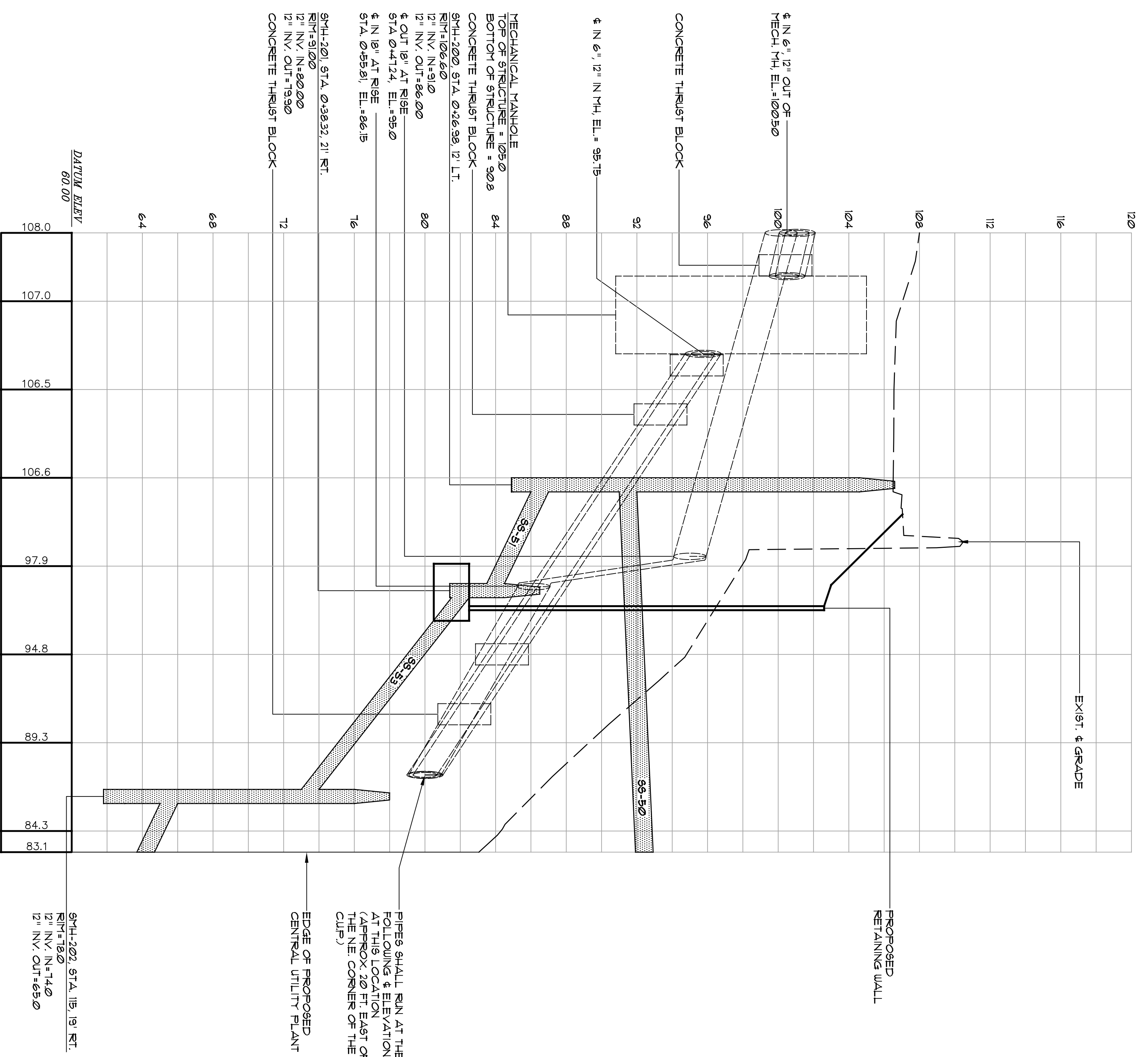
PROFILE: UTILITY BASELINE 1 (SANITARY SEWER AND MECHANICAL PIPING) SCALE: 1/32" VERT.
