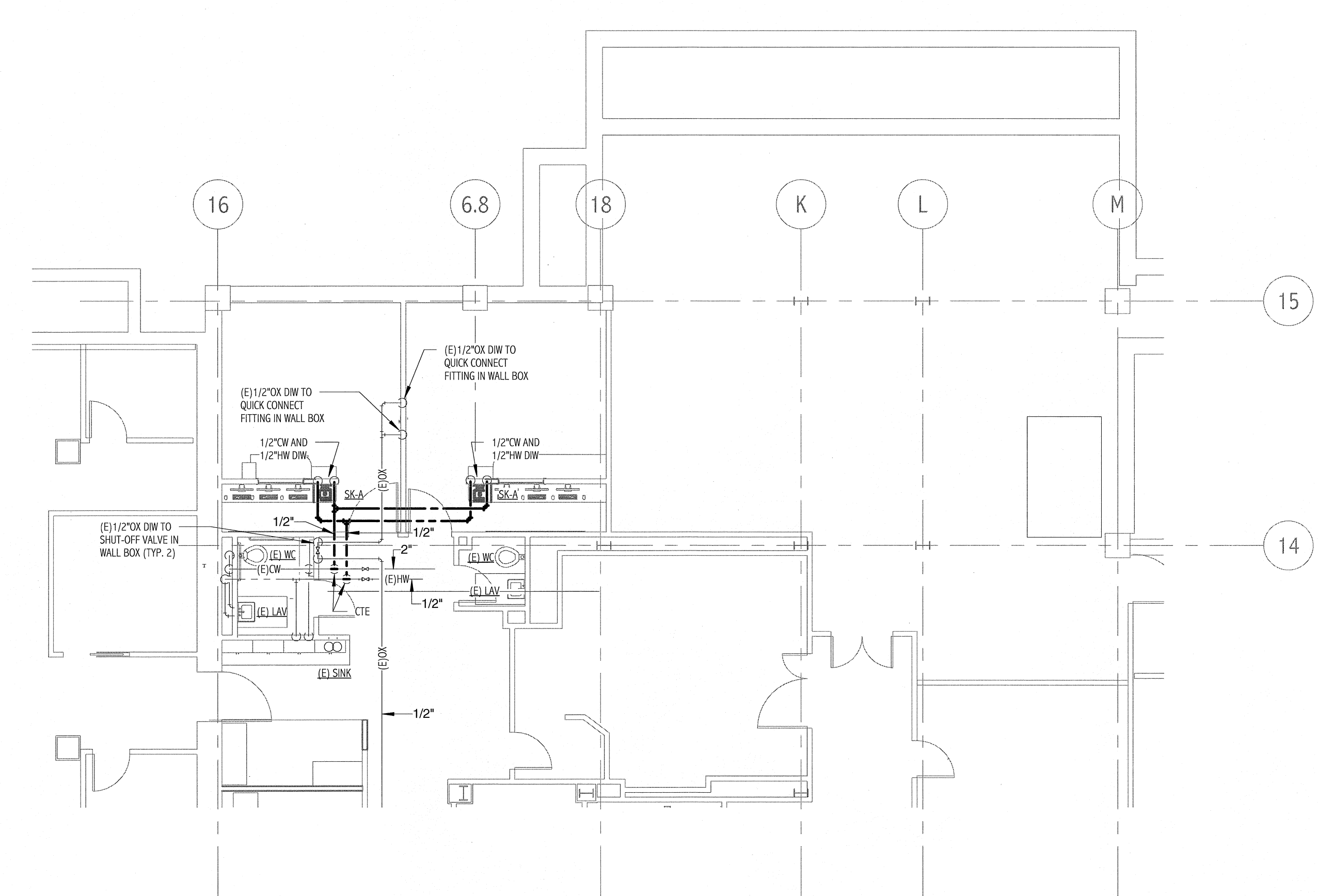
② FLUORO DOMESTIC WATER PIPING PLAN 1/8" = 1'-0"
