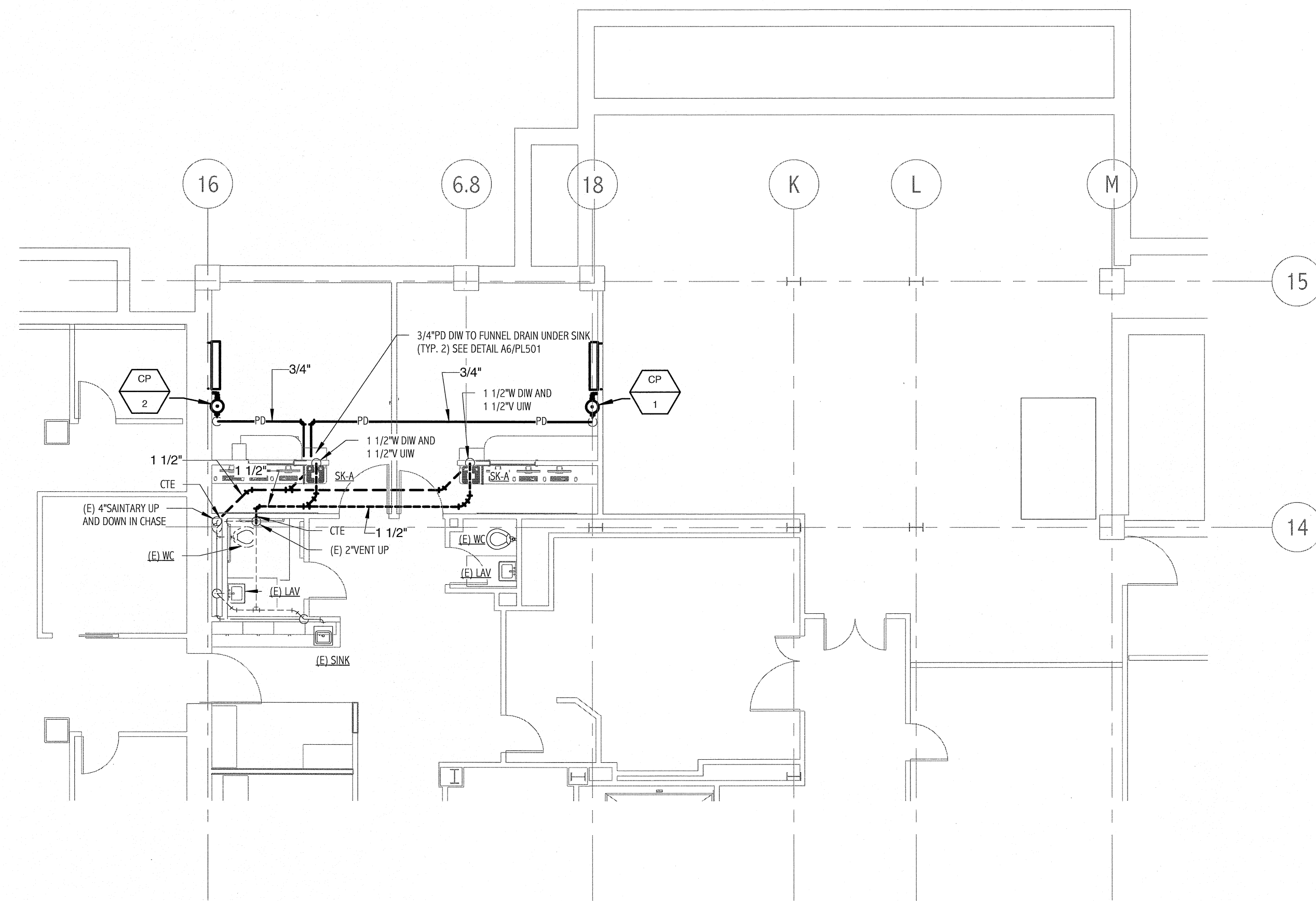
① FLUORO SANITARY PIPING PLAN 1/8" = 1'-0"
