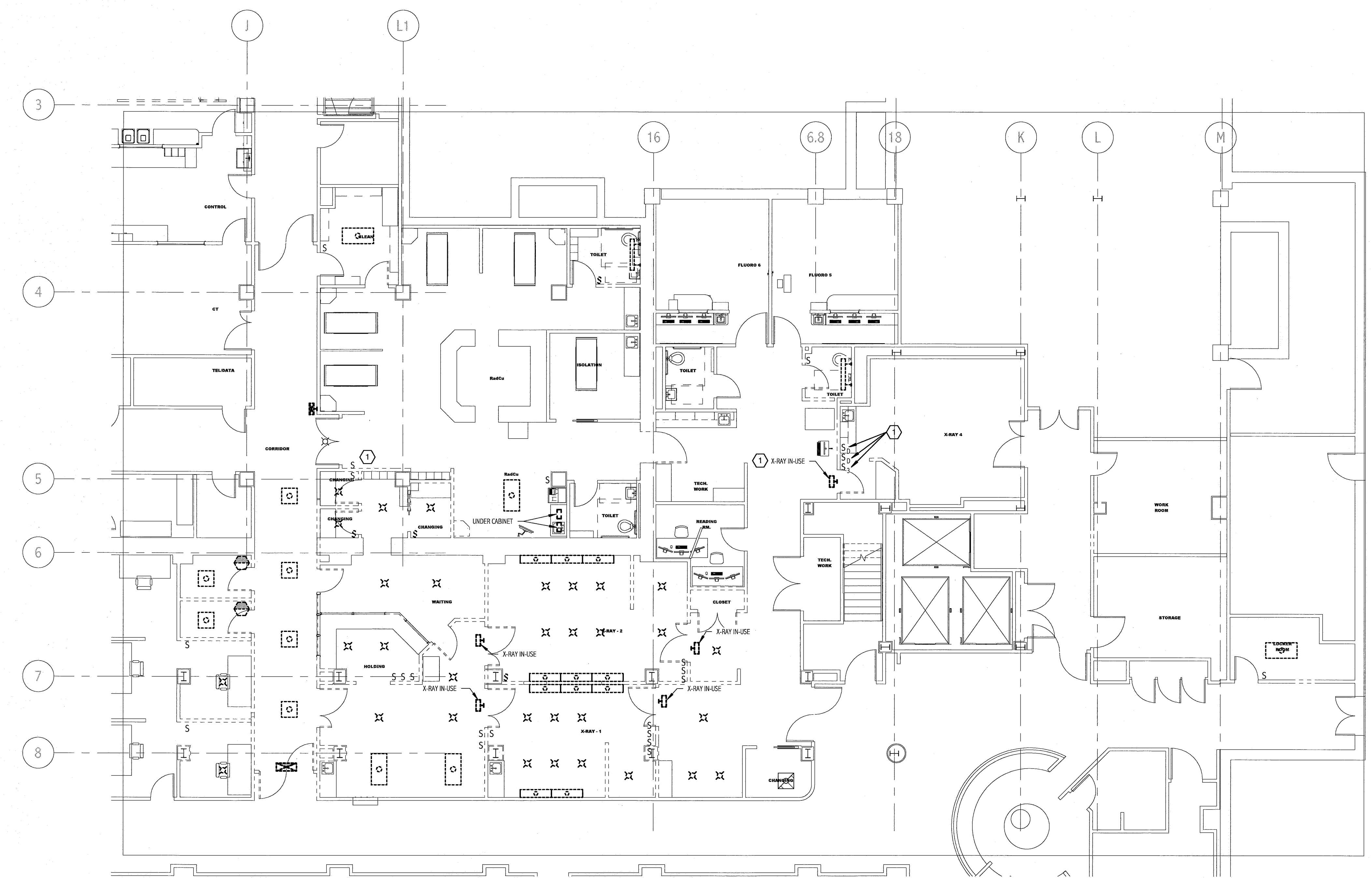
BASEMENT LEVEL LIGHTING DEMOLITION PLAN 1/8" = 1'-0"
