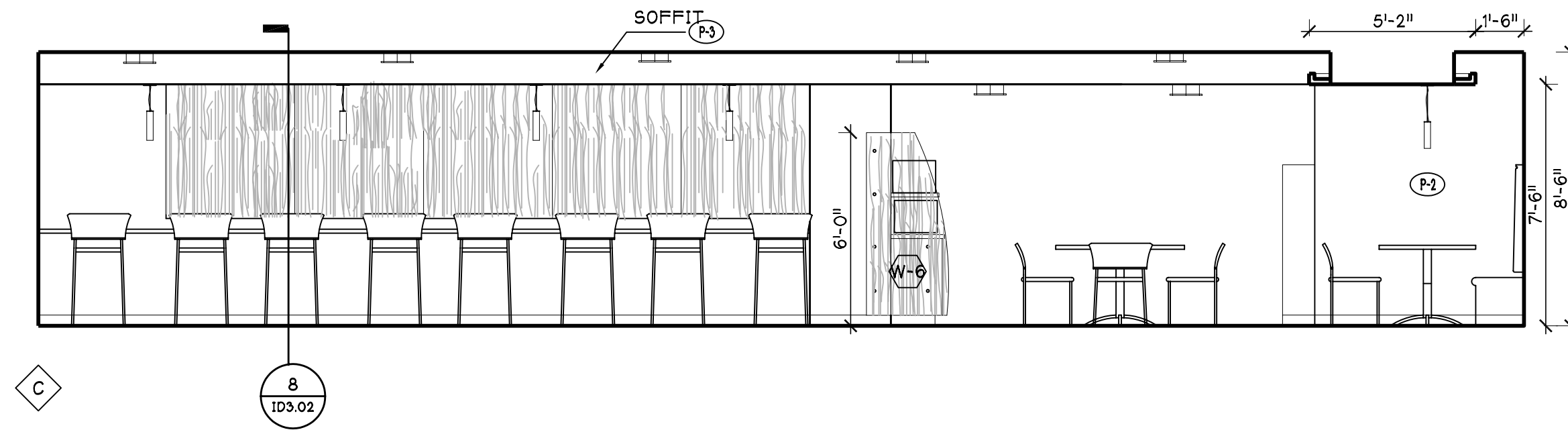
3 DINING AREA 4 1/4" = 1'-0"
