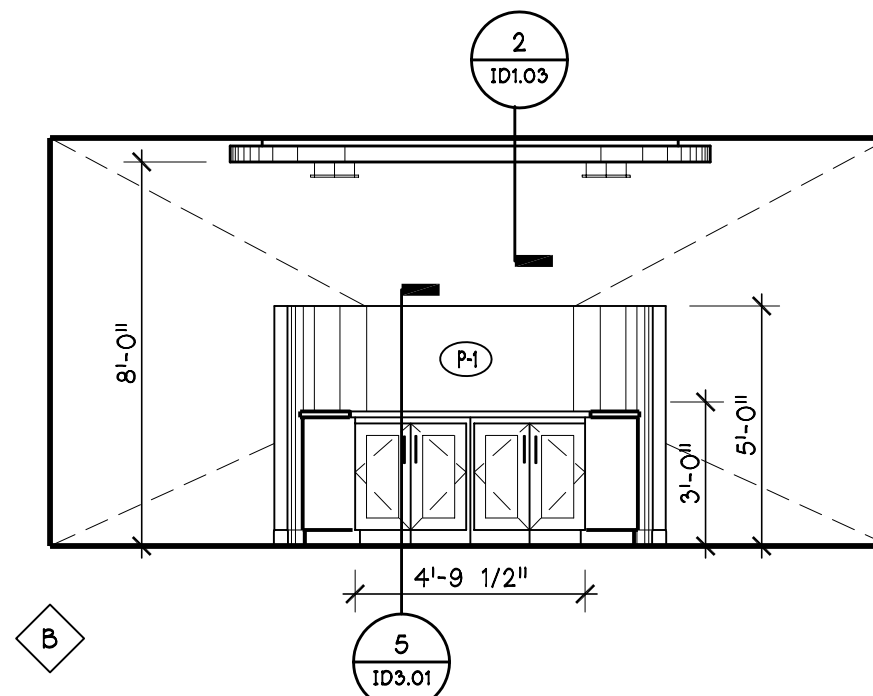
4 TRASH AREA 1/4" = 1'-0"
