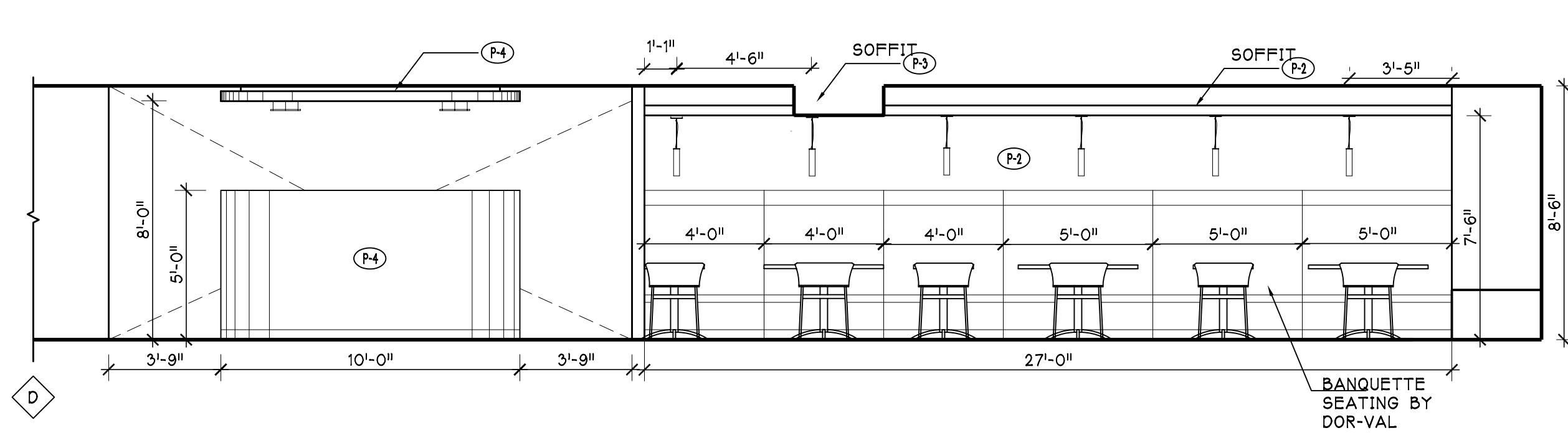
3 DINING AREA 4 1/4" = 1'-0"
