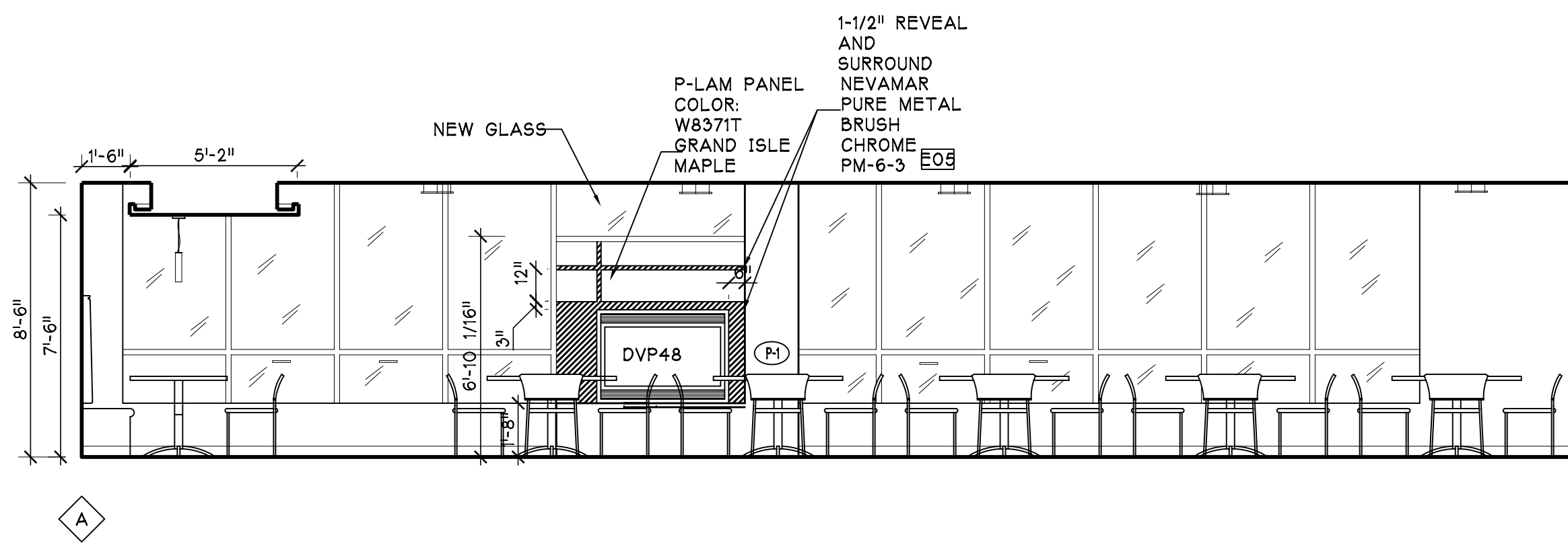
3 DINING AREA 4 1/4" = 1'-0"
