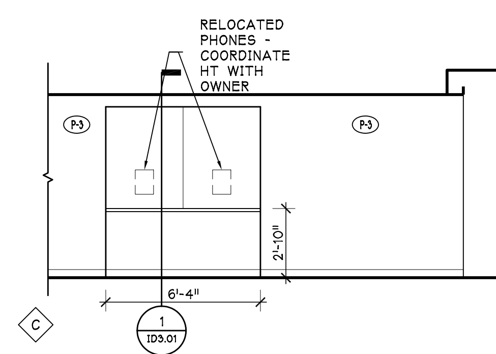
5 PHONE AREA 1/4" = 1'-0"
