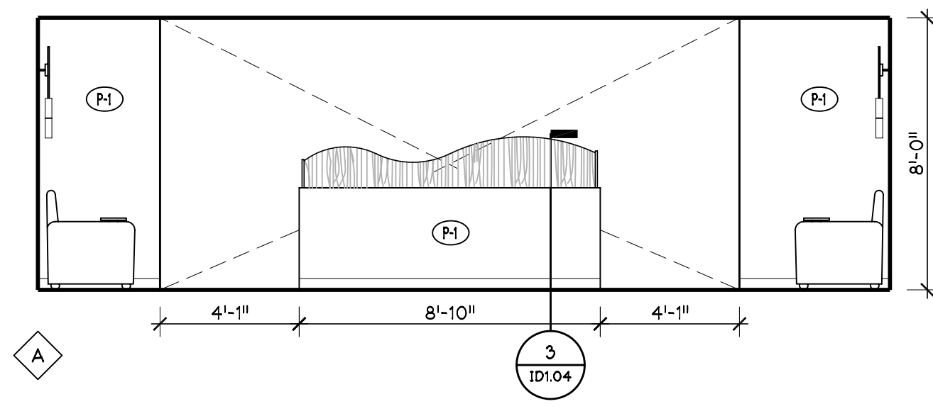
6 DINING AREA 1 1/4" = 1'-0"
