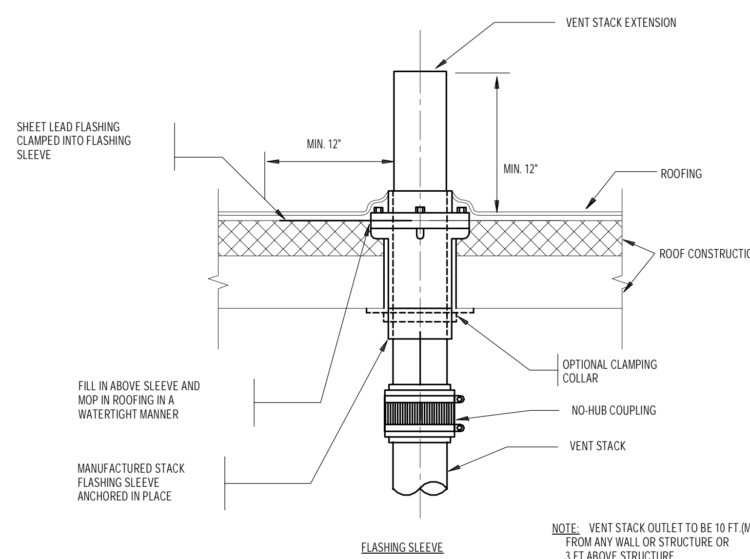
2 VENT THROUGH ROOF SCALE: 1/8" = 1'-0"
