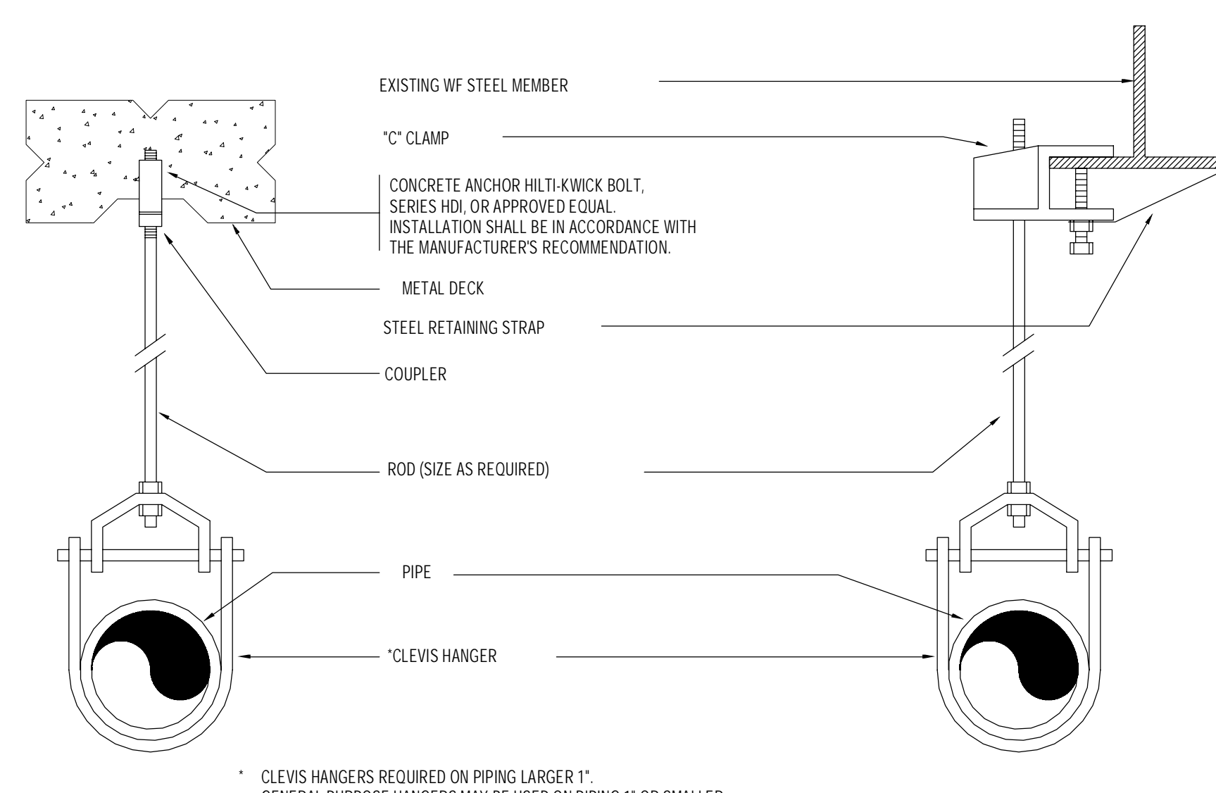
3 TYPICAL HANGER DETAIL SCALE: 1/8" = 1'-0"
