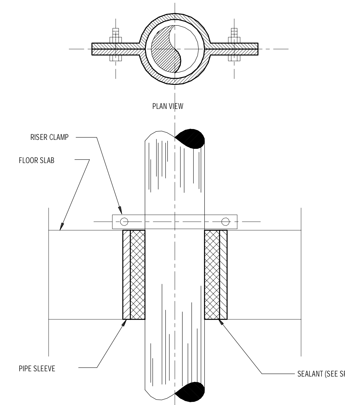
1 PIPE SLEEVE THROUGH FLOOR SLAB SCALE: 1/8" = 1'-0"
