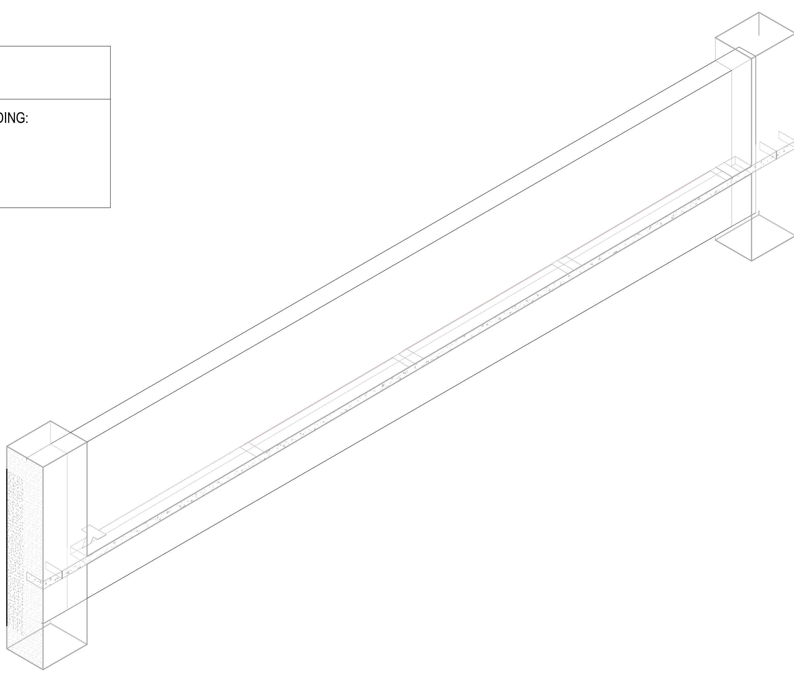
3 PRECAST SPANDREL (S1) INTERIOR AXONOMETRIC
