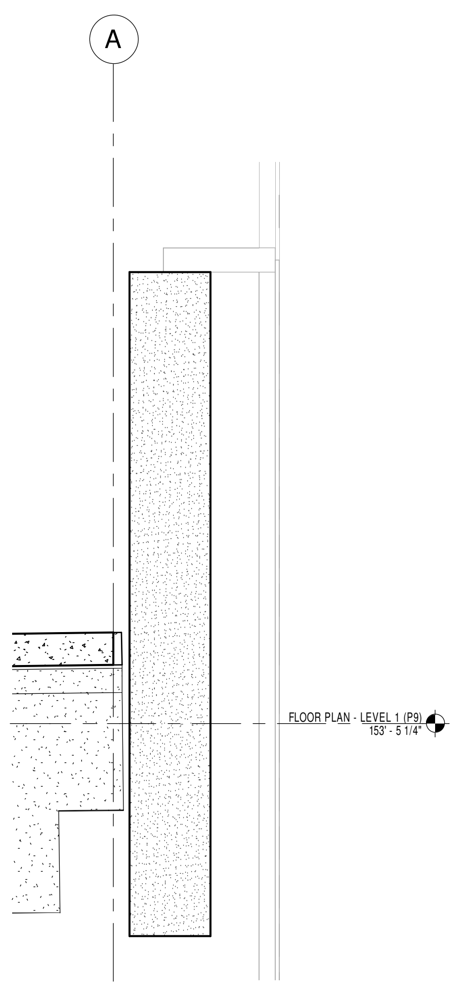
5 PRECAST SPANDREL (S1) SECTION 1" = 1'-0"
