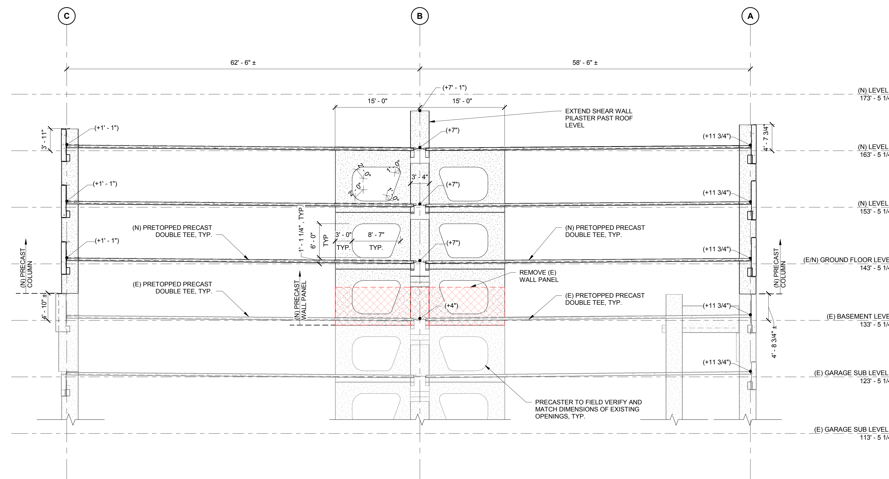
2 WALL ELEVATION - GRID LINE "6" 1/8" = 1'-0"
