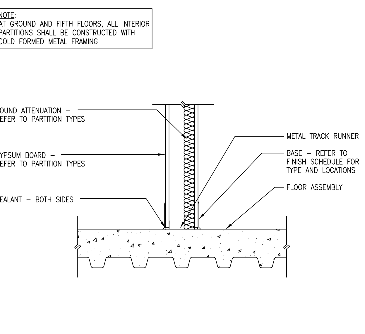
E4 BOTTOM OF WALL DETAIL SCALE: 1 1/2\"/>
