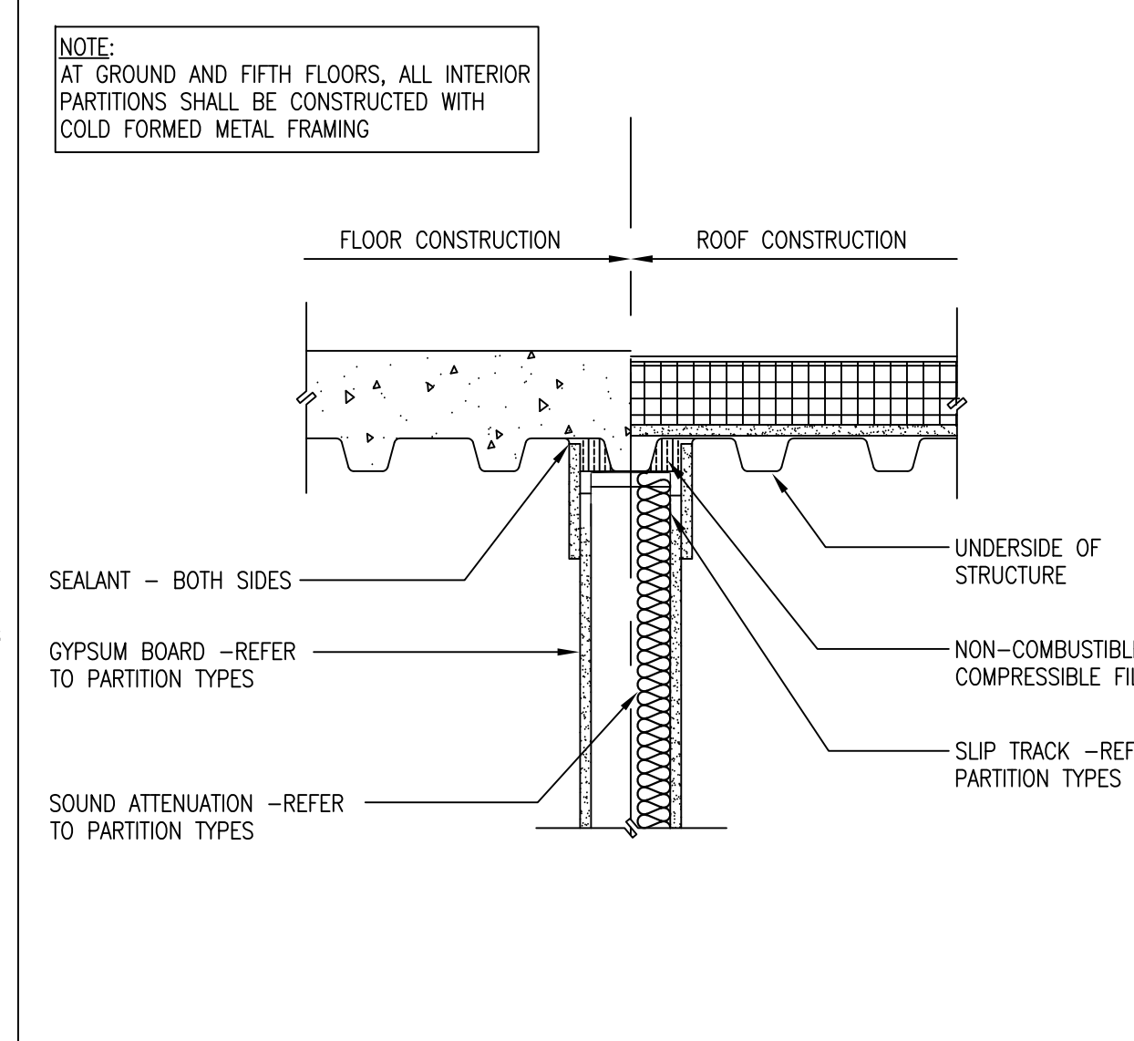
B4 NON-RATED PARTITION -TOP OF WALL DETAIL SCALE: 1 1/2\"/>
