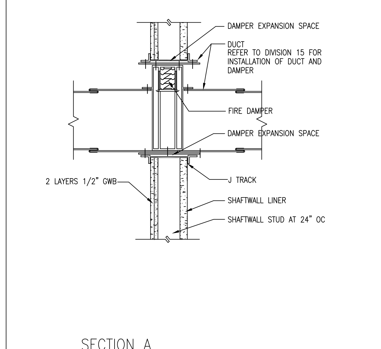
B5 SECTION A DUCT OPENING INTO 2-HOUR SHAFT WALL SCALE: 1 1/2\"/>
