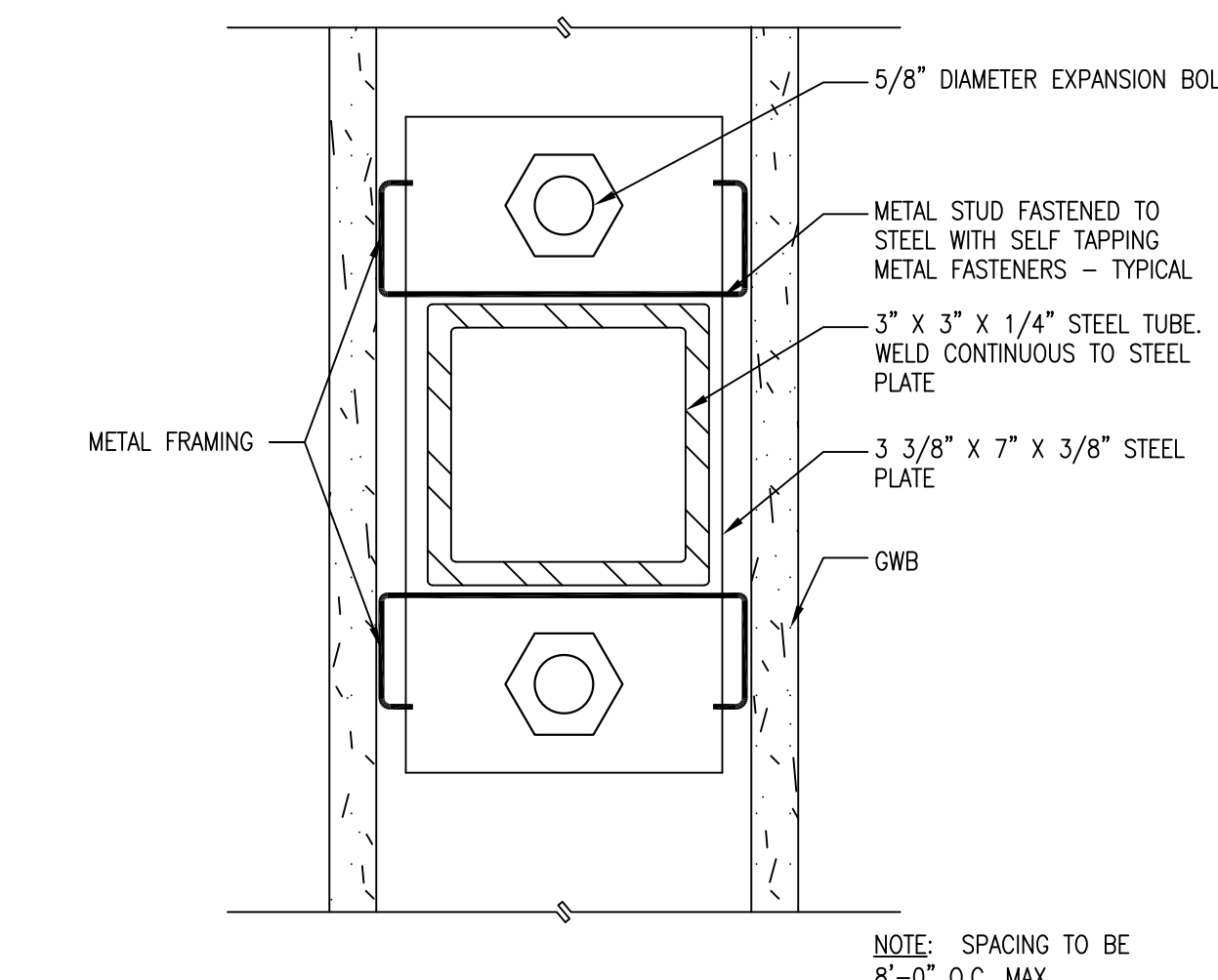
E1 STEEL BRACING DETAIL FOR LOW PARTITIONS W/ UNBRACED ENDS SCALE: 6\"/>
