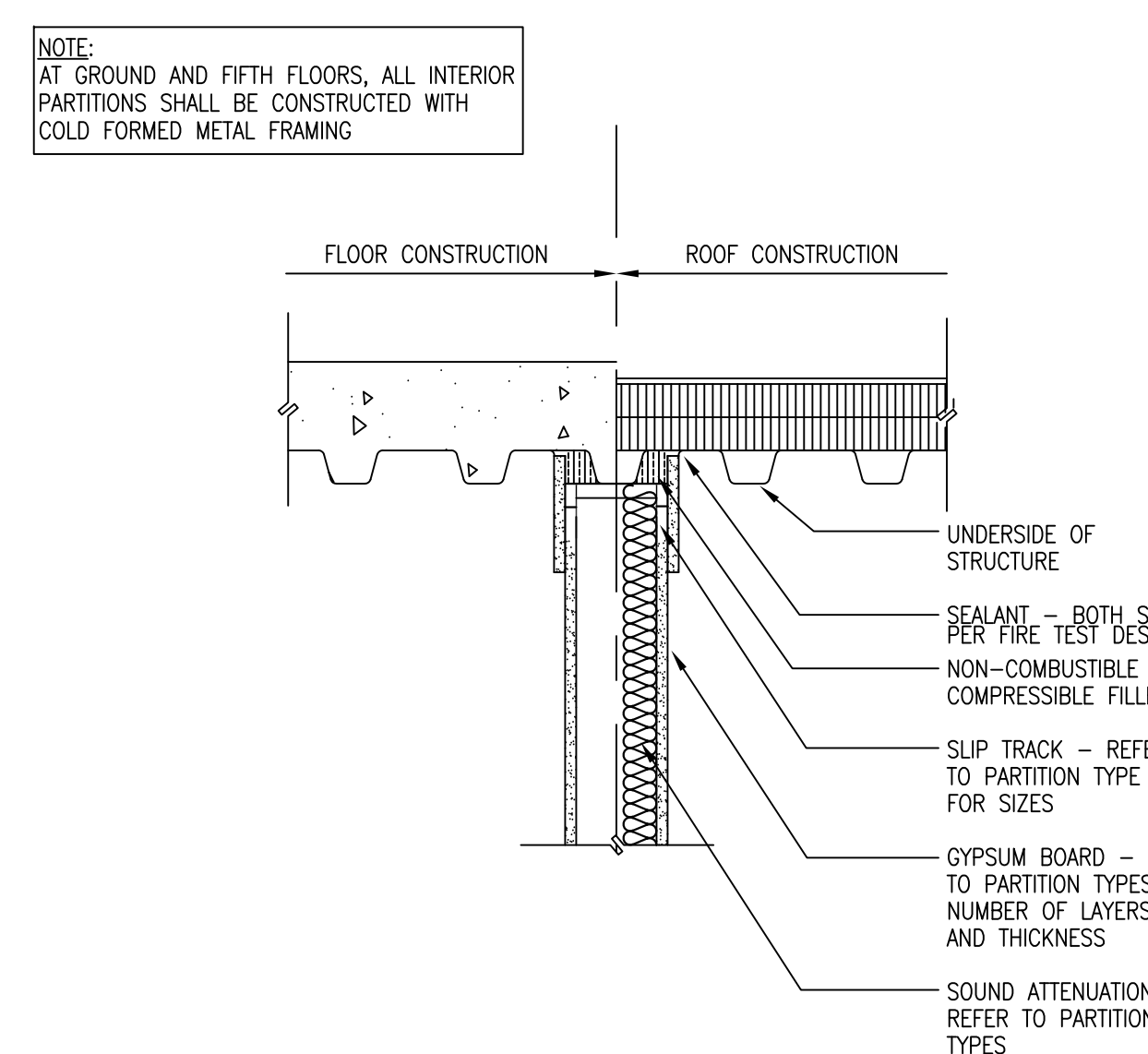
C4 RATED PARTITION -TOP OF WALL DETAIL SCALE: 1 1/2\"/>
