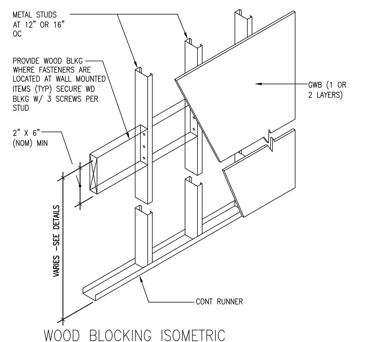
E5 WOOD BLOCKING ISOMETRIC FOR WALL MOUNTED ITEMS SCALE: 3/4\"/>
