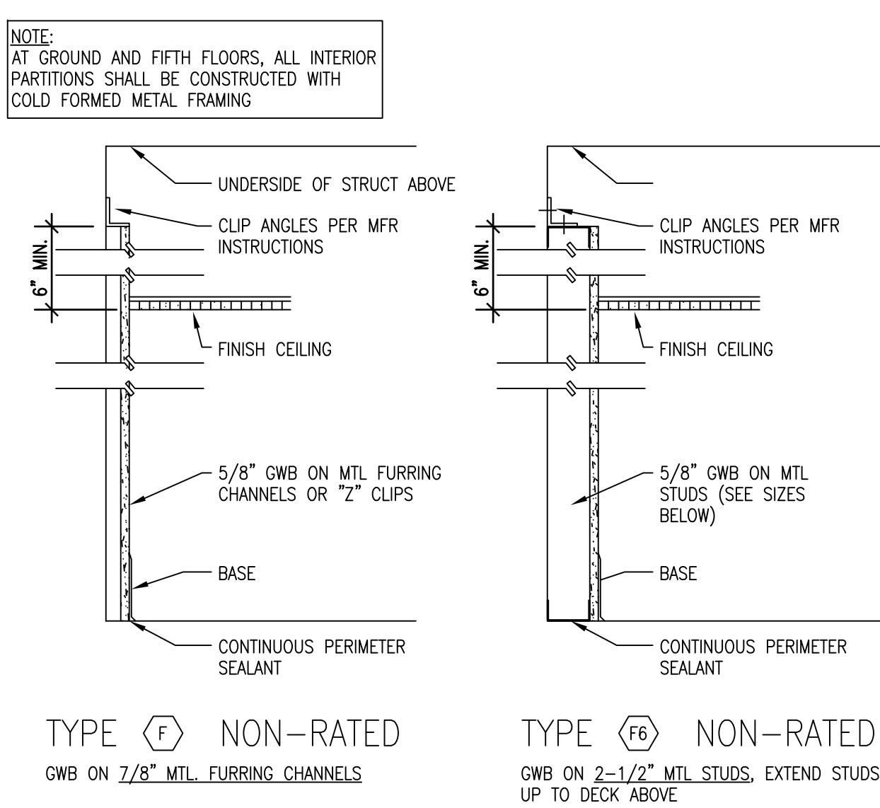
F5 WALL FURRING TYPES SCALE: 1 1/2\"/>
