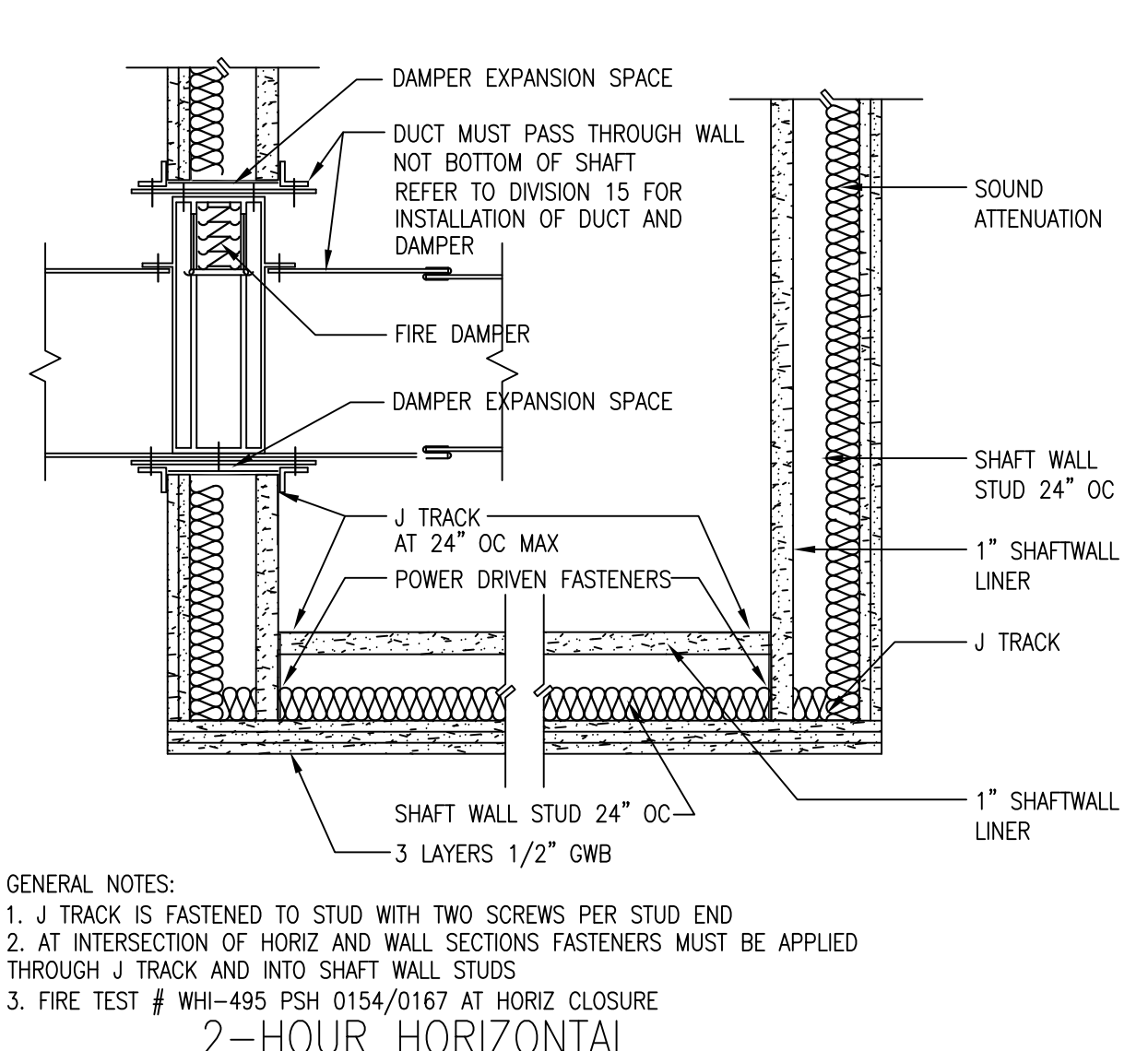
D5 2-HOUR HORIZONTAL SHAFT WALL SHAFT CLOSURE SCALE: 1 1/2\"/>
