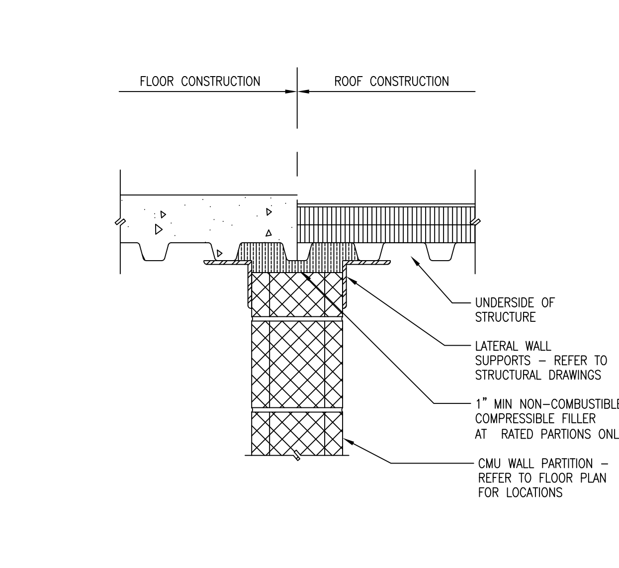
D4 CMU PARTITION -TOP OF WALL DETAIL SCALE: 1 1/2\"/>
