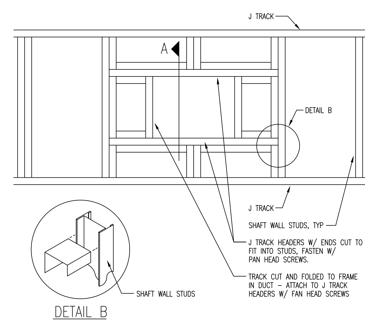
C5 DUCT OPENING INTO 2-HOUR SHAFT WALL SCALE: 1 1/2\"/>
