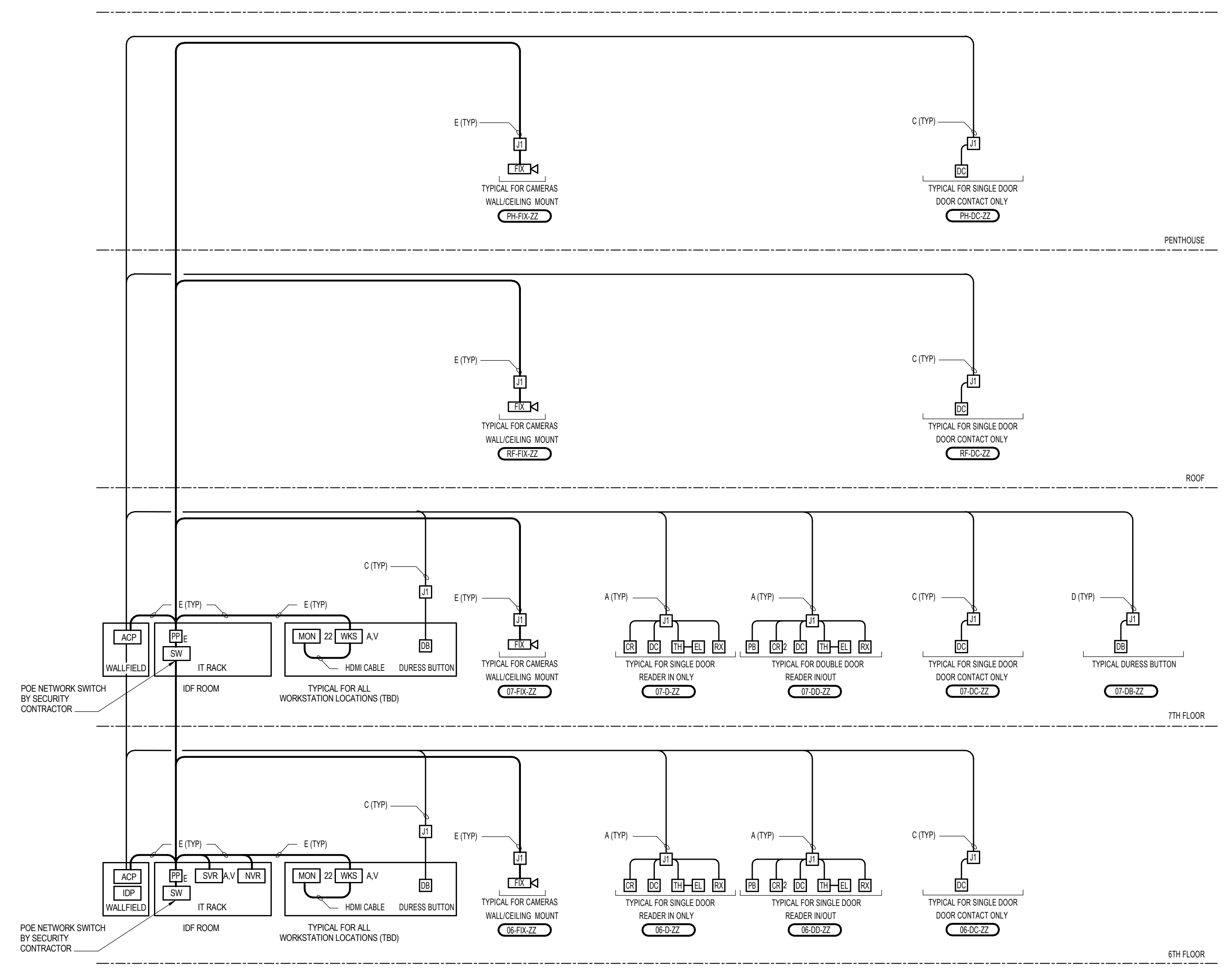
1 SECURITY RISER DIAGRAM SCALE: NTS
