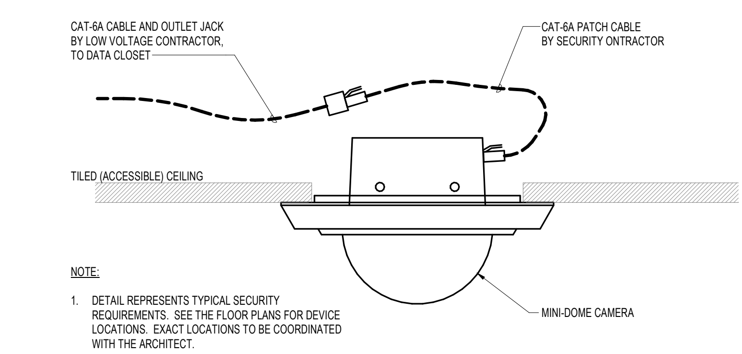
3 CCTV MINI-DOME CAMERA EXTERIOR-INTERIOR FLUSH CEILING MOUNT SCALE: NONE
