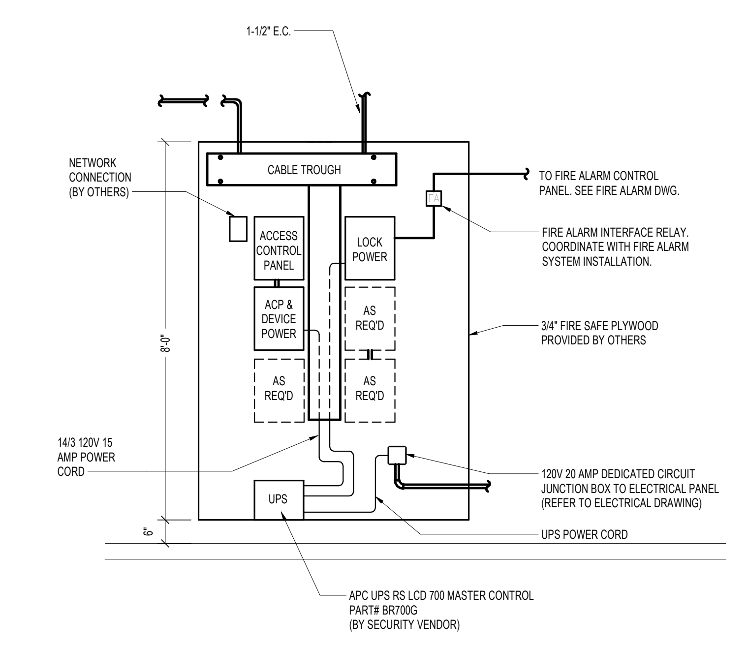
7 SECURITY DISTRIBUTION FRAME ELEVATION VIEW SCALE: NONE
