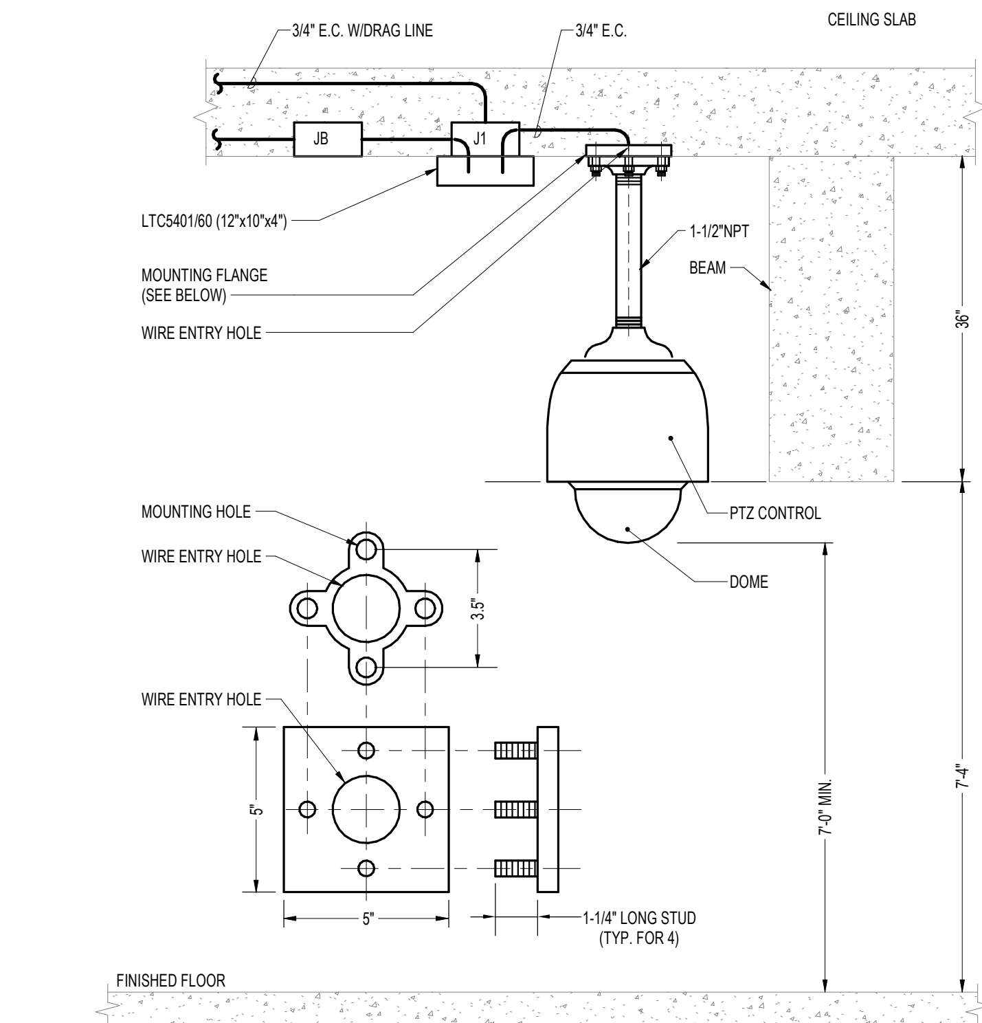
4 CCTV DOME CAMERA CEILING MOUNT SCALE: NONE
