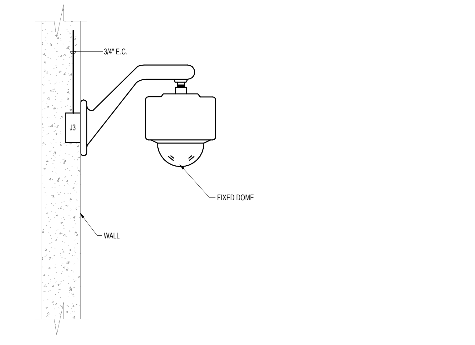
6 CCTV DOME CAMERA WALL MOUNT SCALE: NONE
