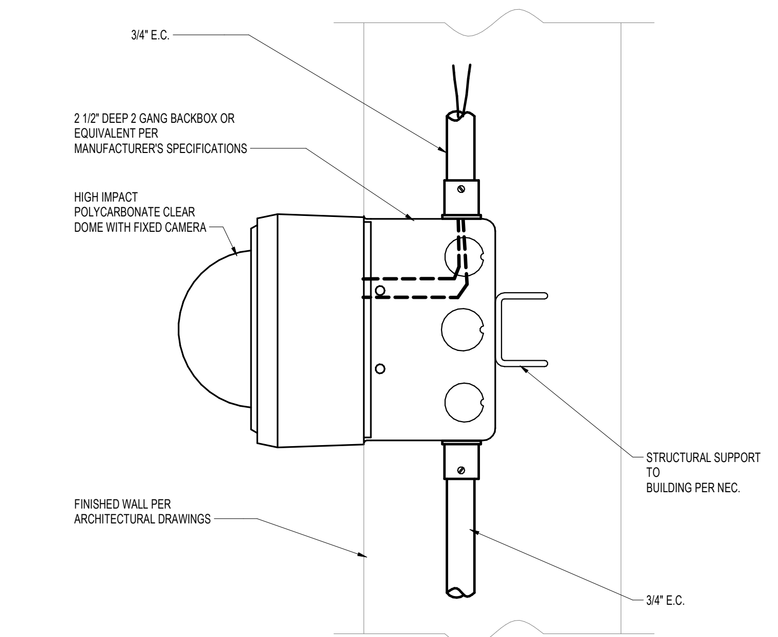
2 CCTV MINI-DOME CAMERA INTERIOR WALL MOUNT SCALE: NONE
