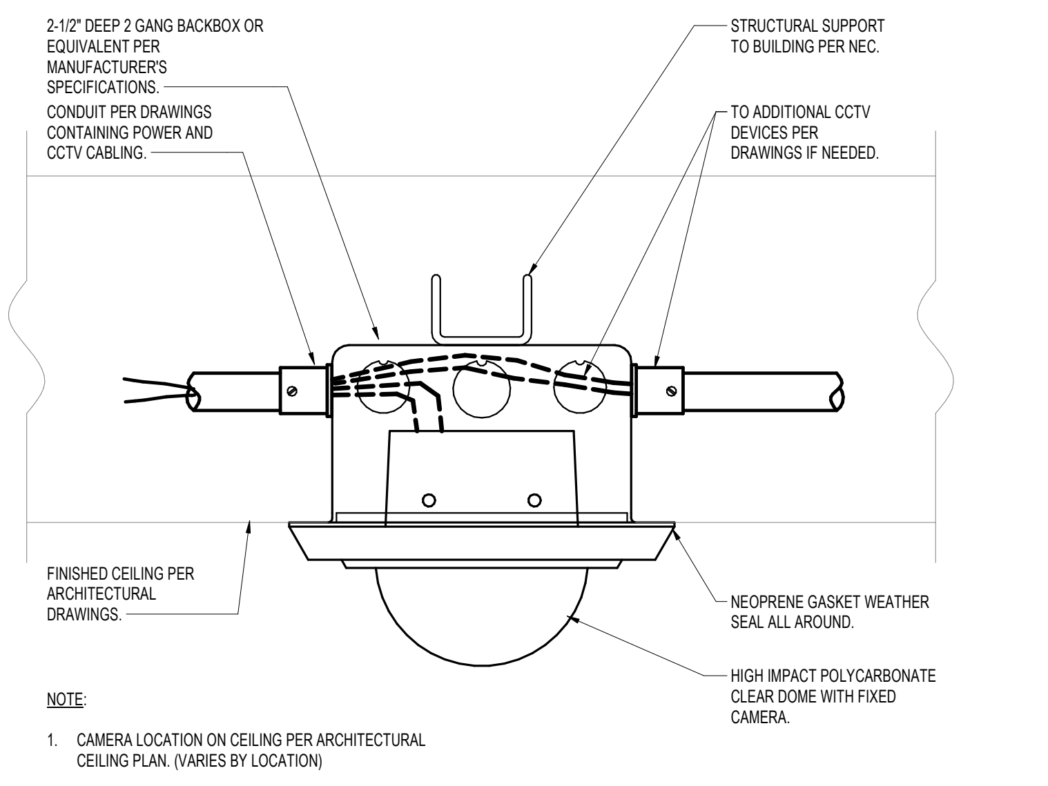
5 CCTV MINI-DOME CAMERA INTERIOR CEILING MOUNT SCALE: NONE
