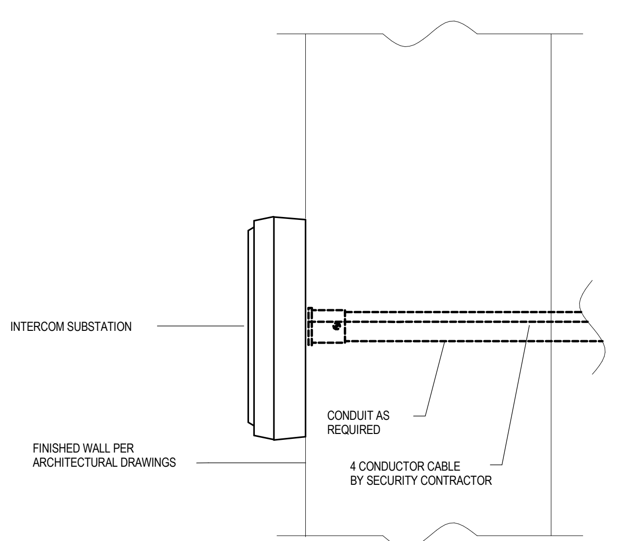
11 INT/EXT WALL MOUNT INTERCOM SUBSTATION (2/4 WIRE) SCALE: NTS
