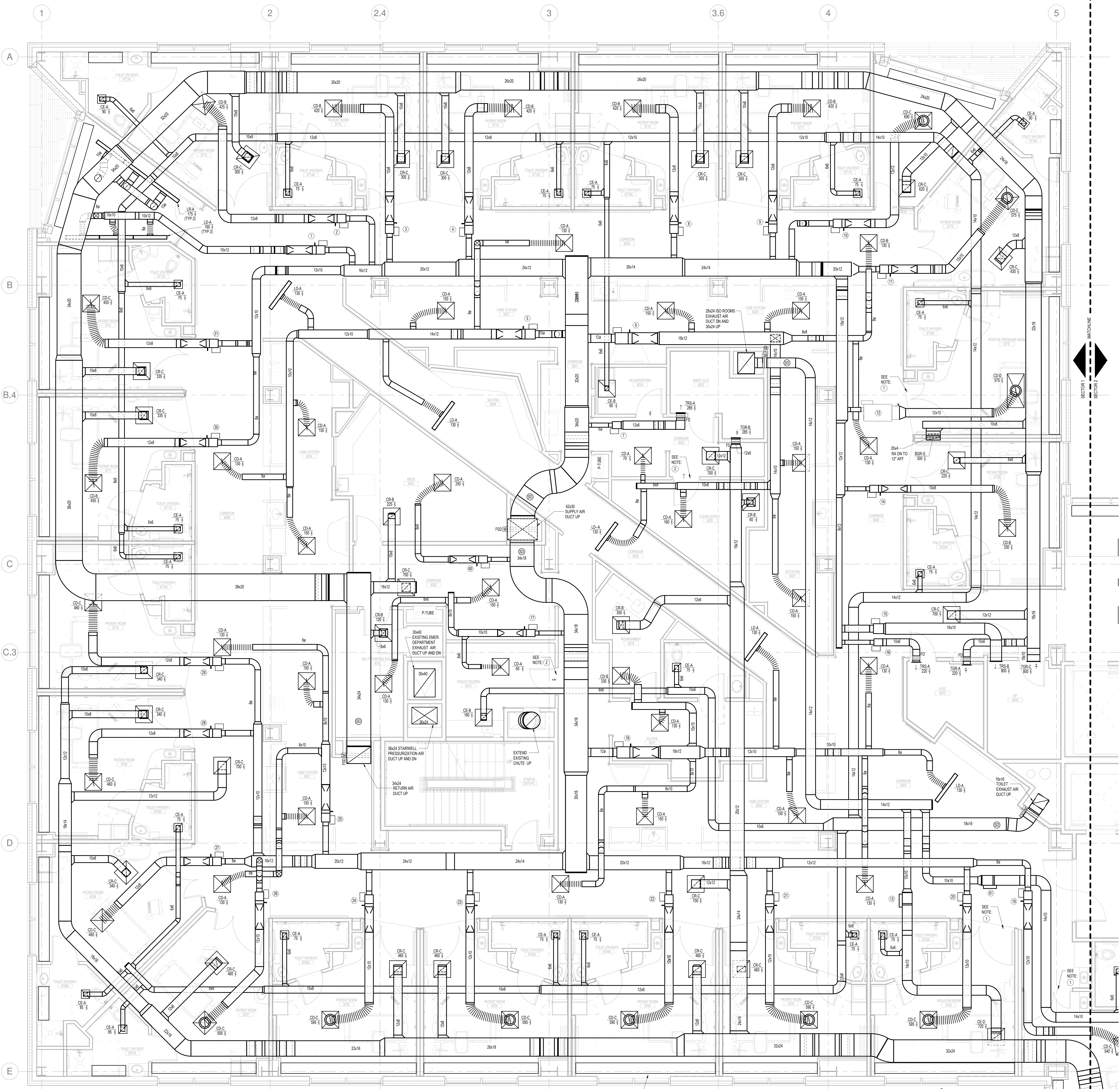
1 LEVEL 6 - SECTOR 1 SCALE: 1/4" = 1'-0"
