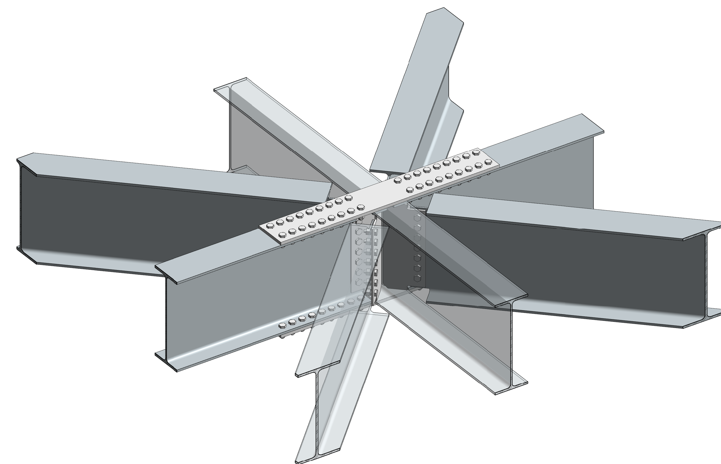
1 HELIPAD CENTER CONNECTION
