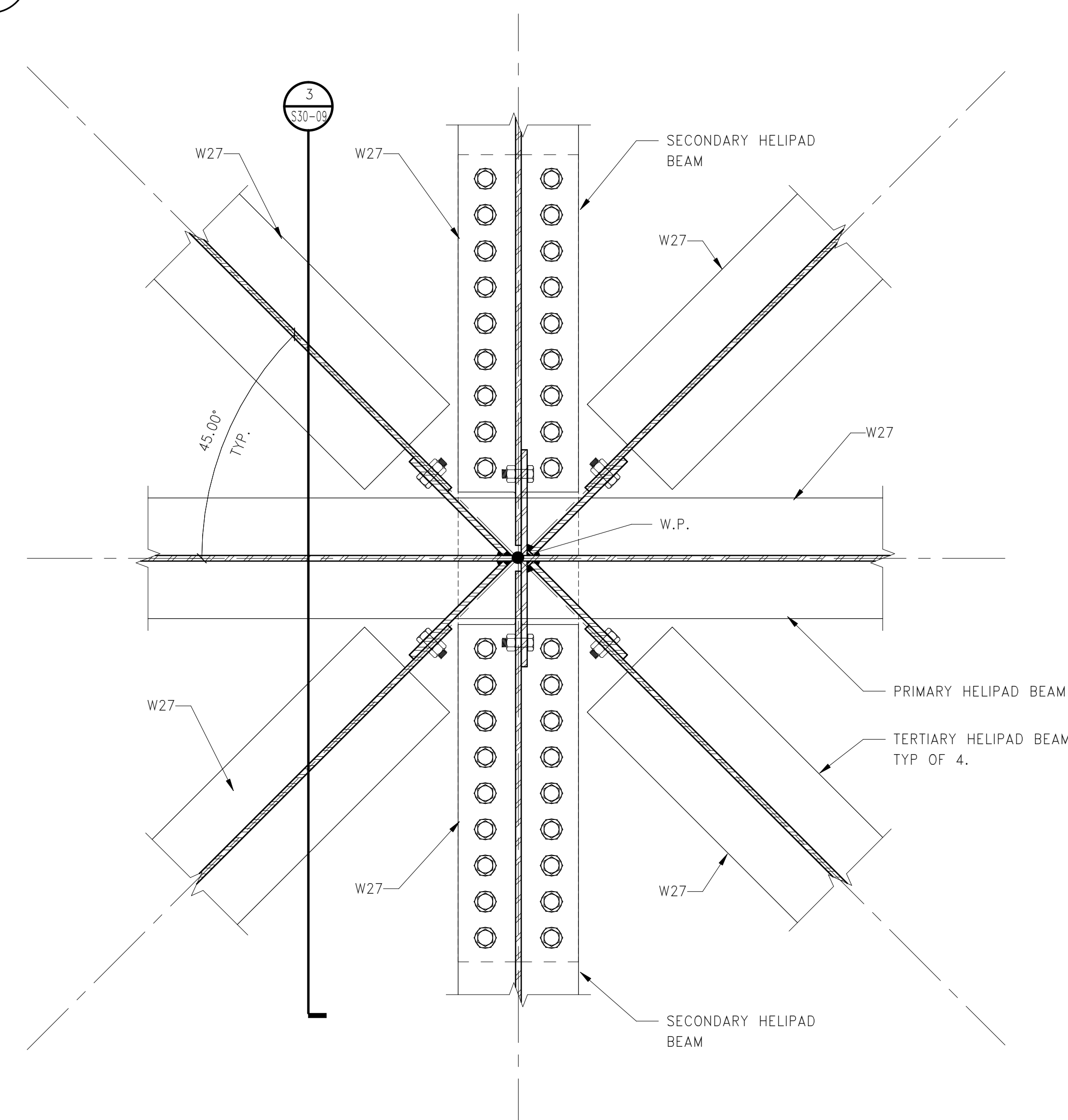
2 HELIPAD CENTER CONNECTION PLAN DETAIL
