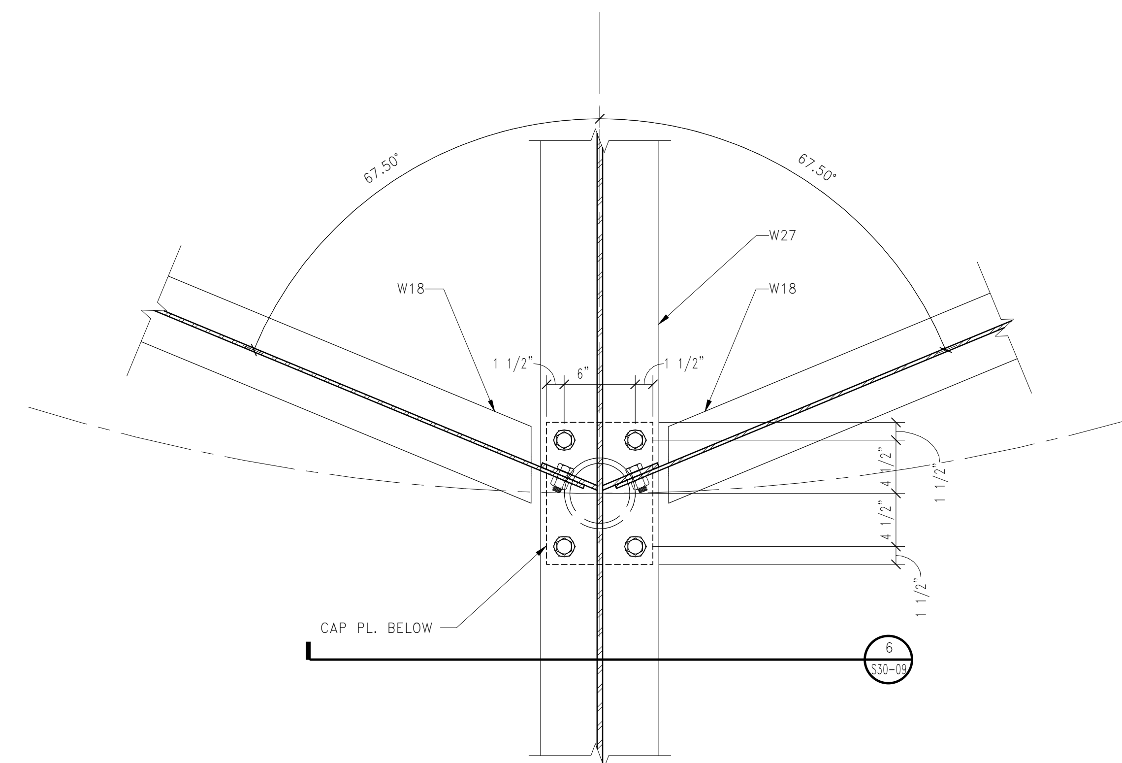
5 HELIPAD BEAM OVER COLUMN PLAN DETAIL
