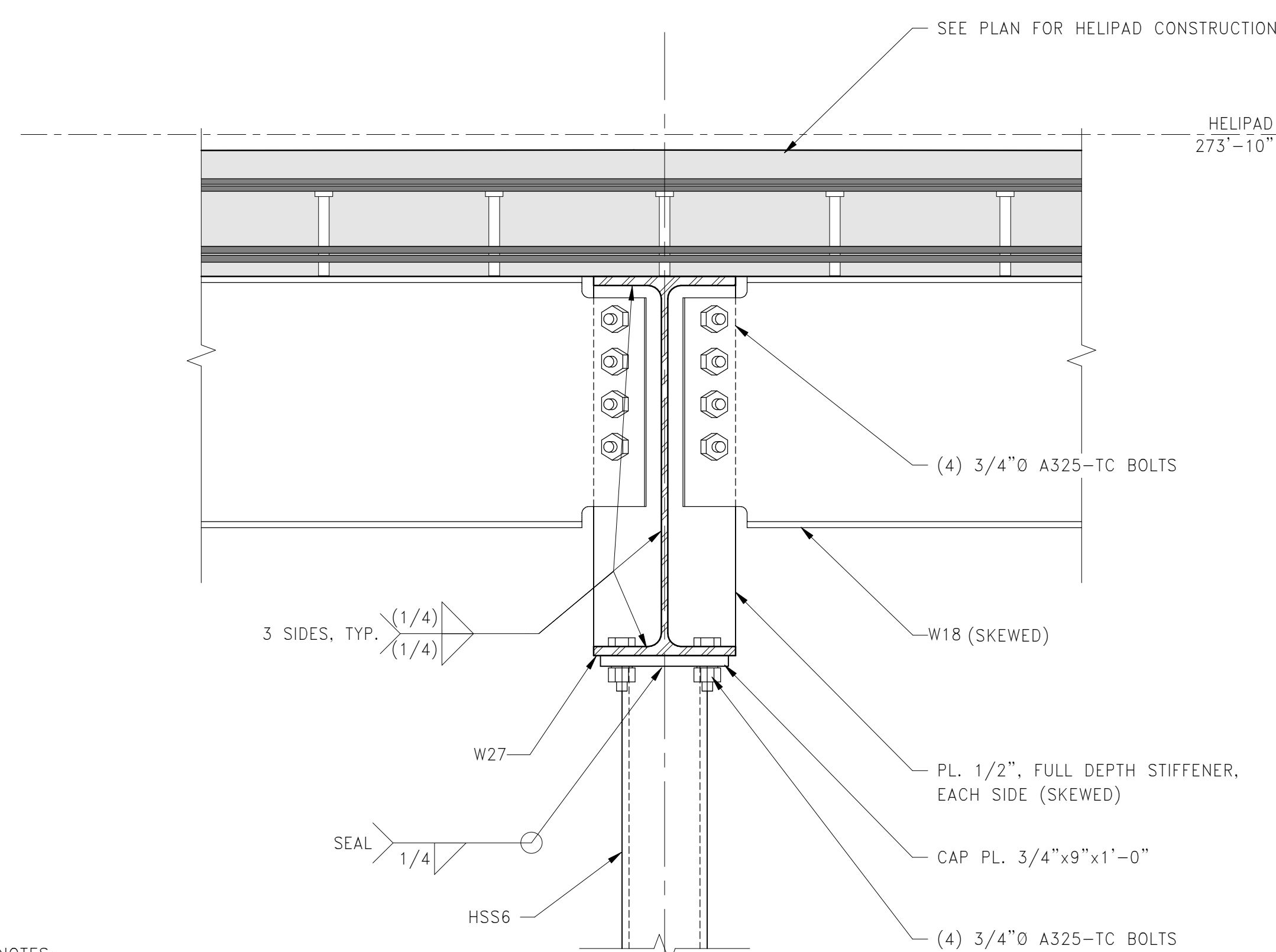
6 SECTION: HELIPAD BEAM OVER COLUMN
