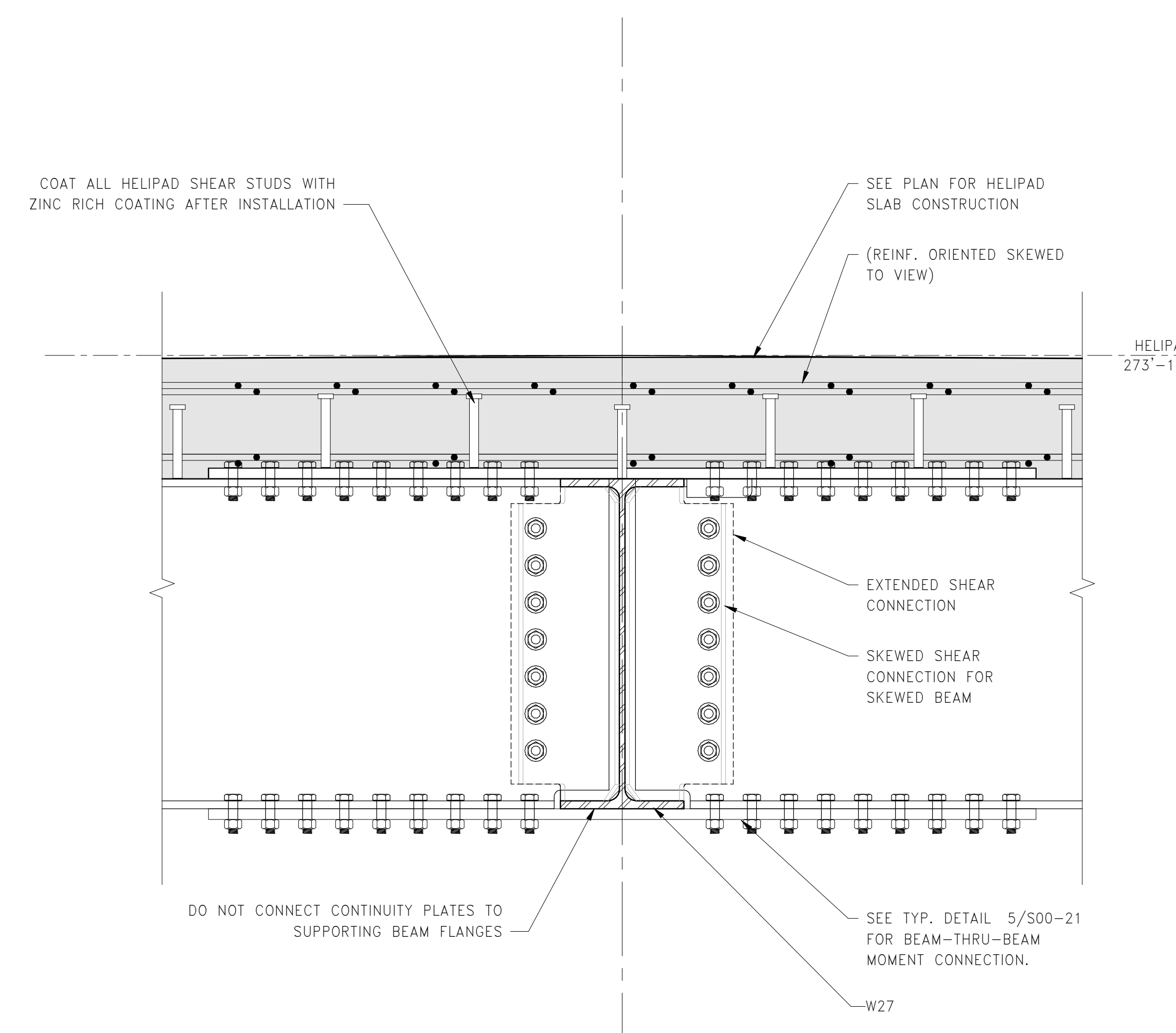
6 SECTION: HELIPAD BEAM OVER COLUMN
