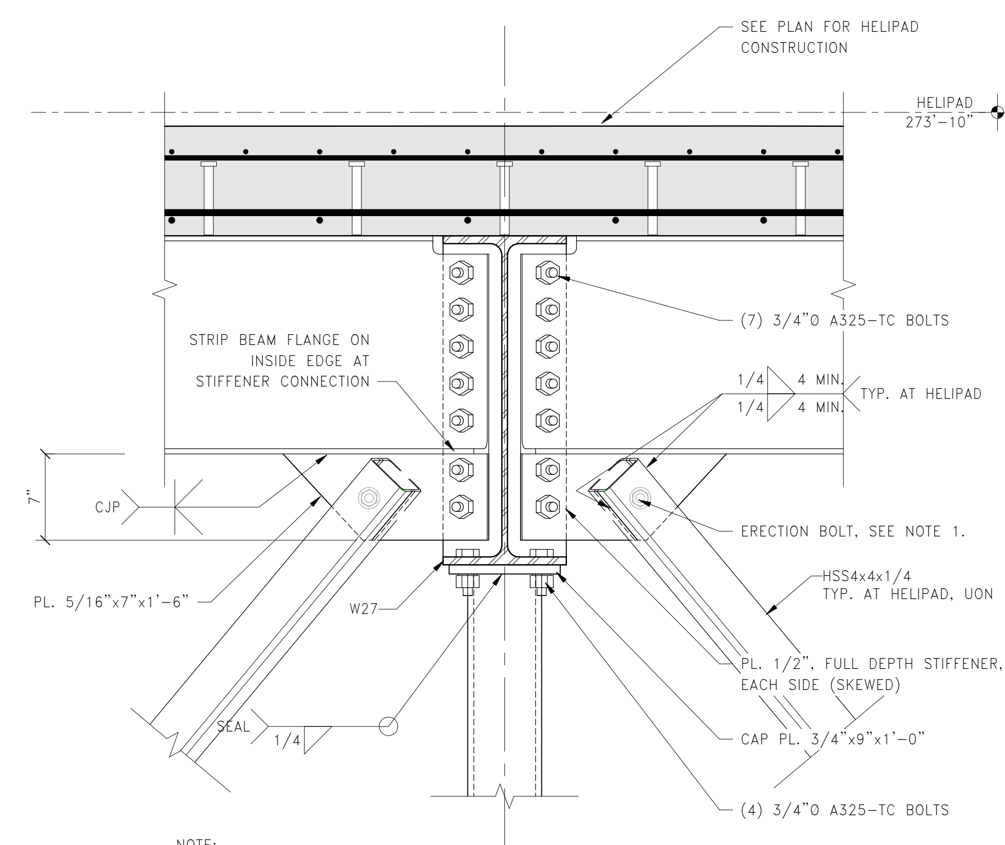
9 SECTION: HELIPAD BEAM OVER COLUMN W/BRACES
