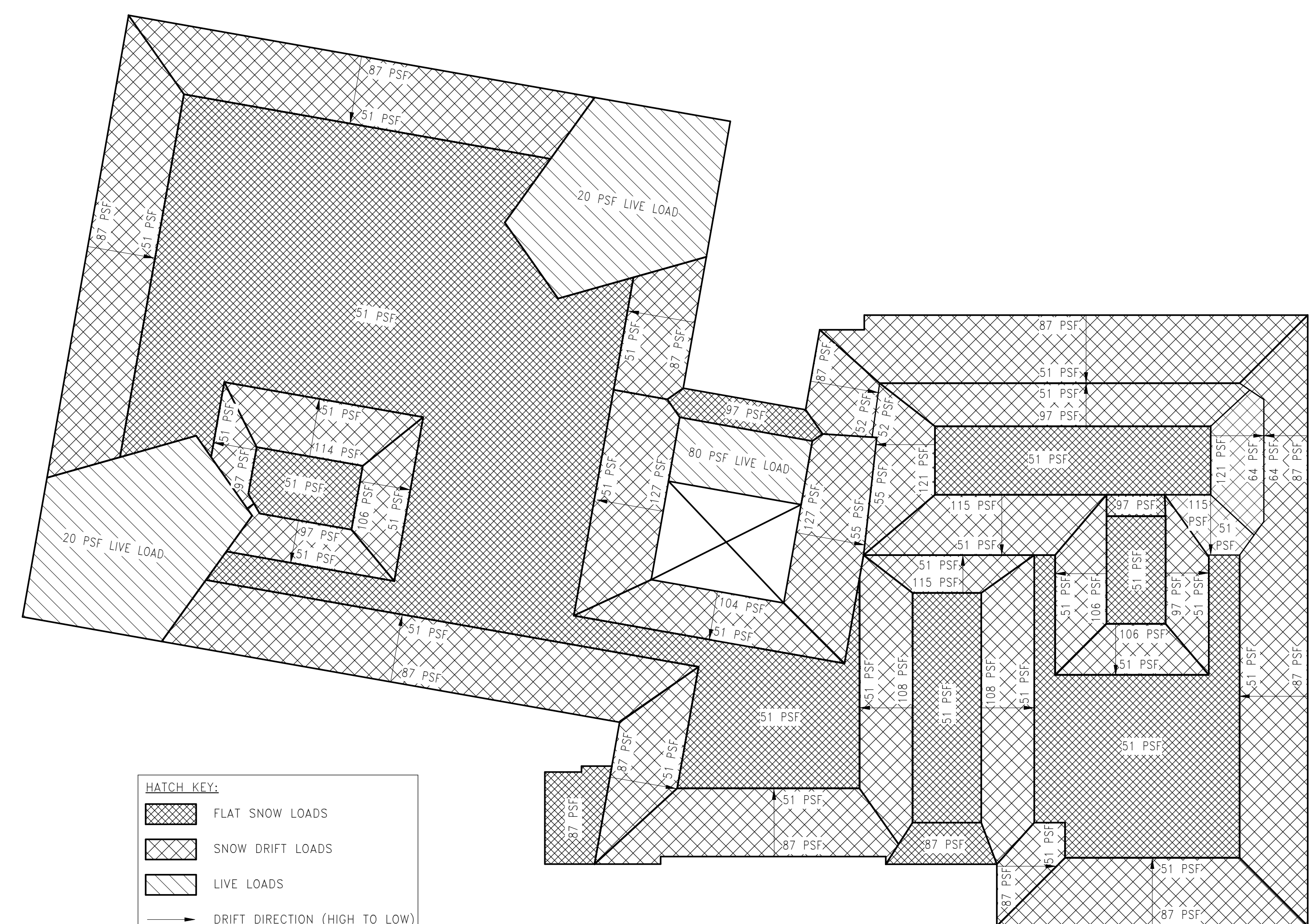
ROOF LIVE LOADS AND SNOW LOADS 1/16" = 1'-0"
