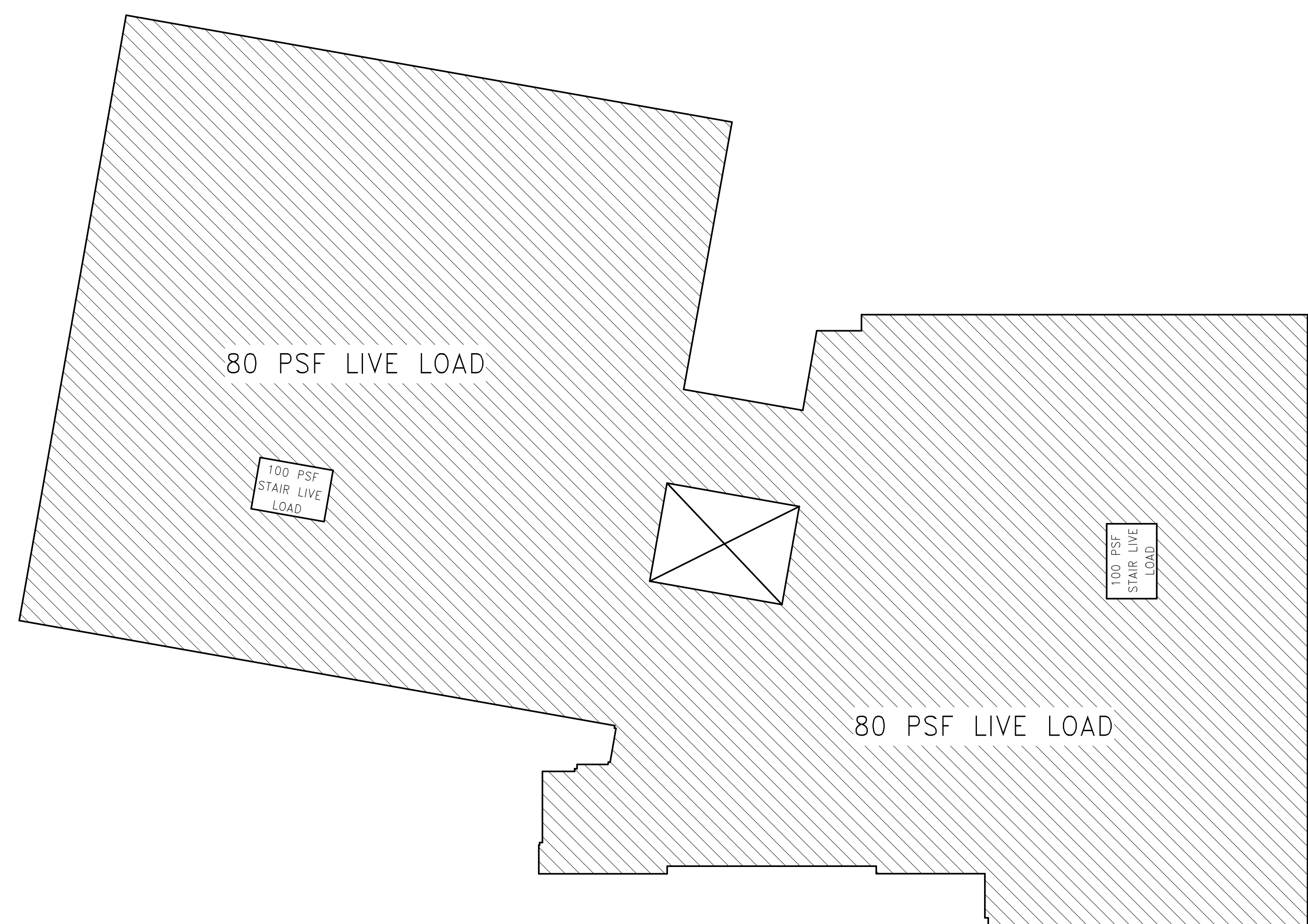
LEVEL 6 LIVE LOADS 1/16" = 1'-0"
