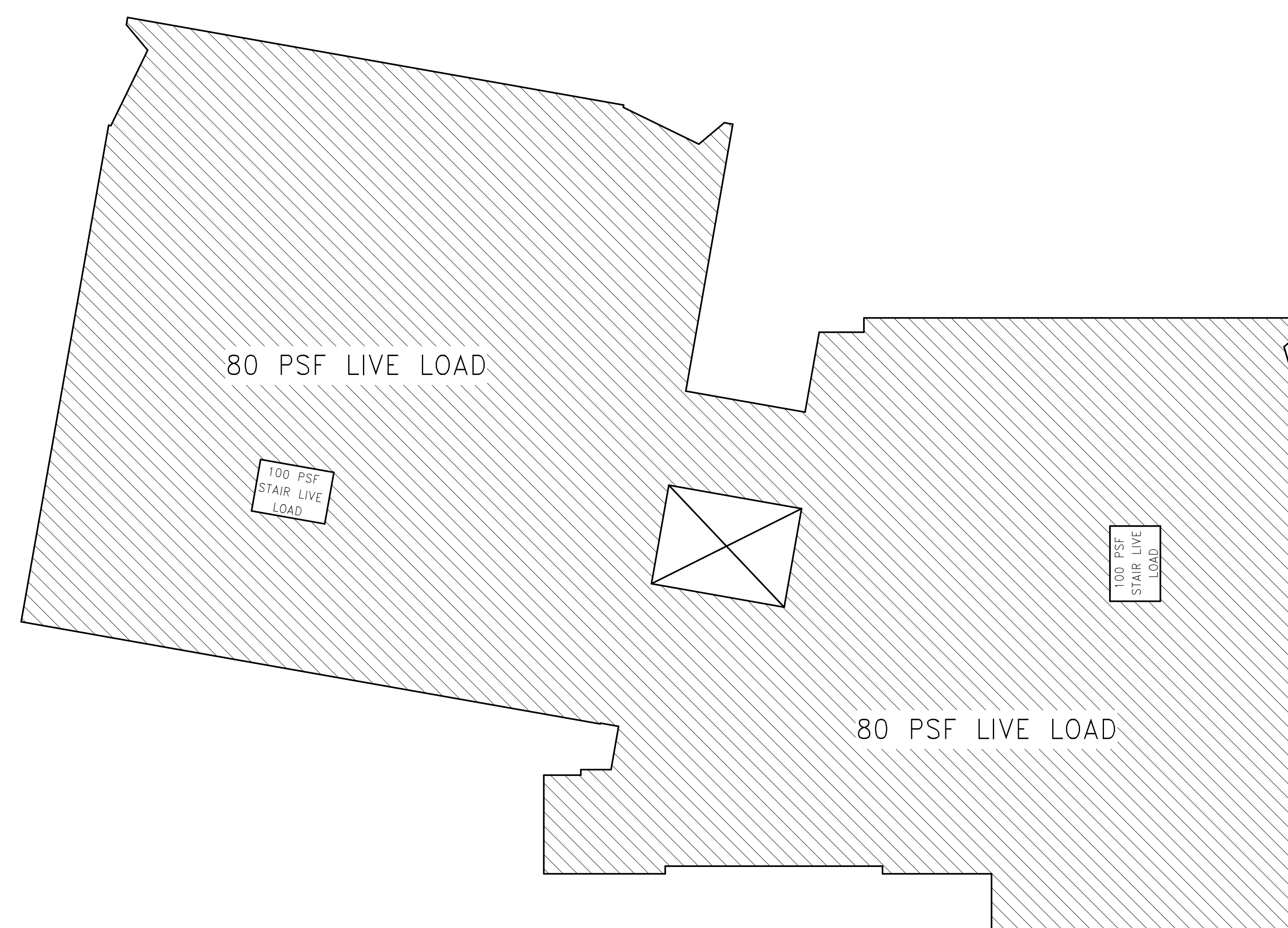
LEVEL 7 LIVE LOADS 1/16" = 1'-0"
