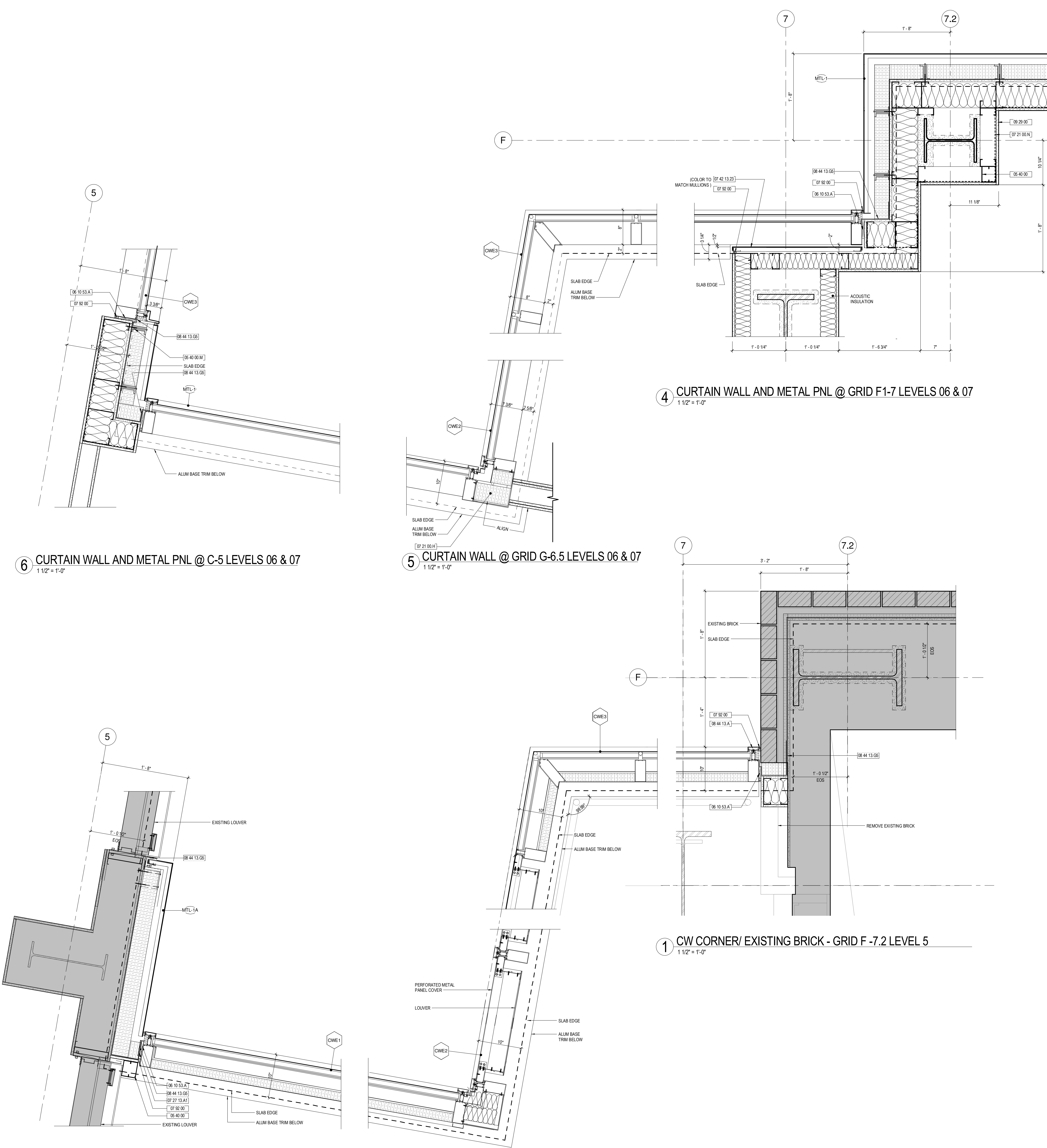
3 CW / METAL PANEL - EXISTING WALL LEVEL 5 1 1/2" = 1'-0"
