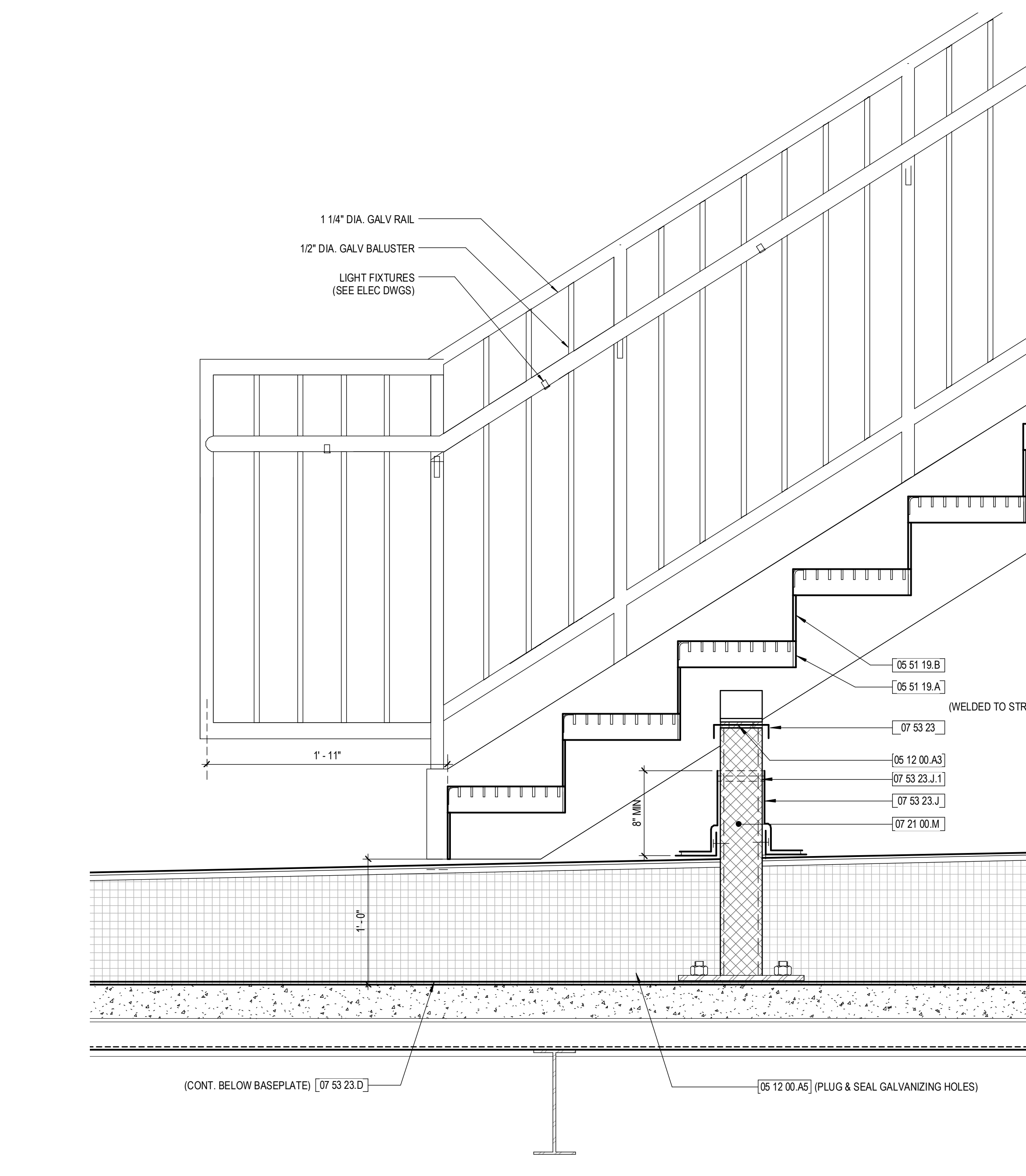
4 HELIPAD STAIR - ROOF 1 1/2" = 1'-0"
