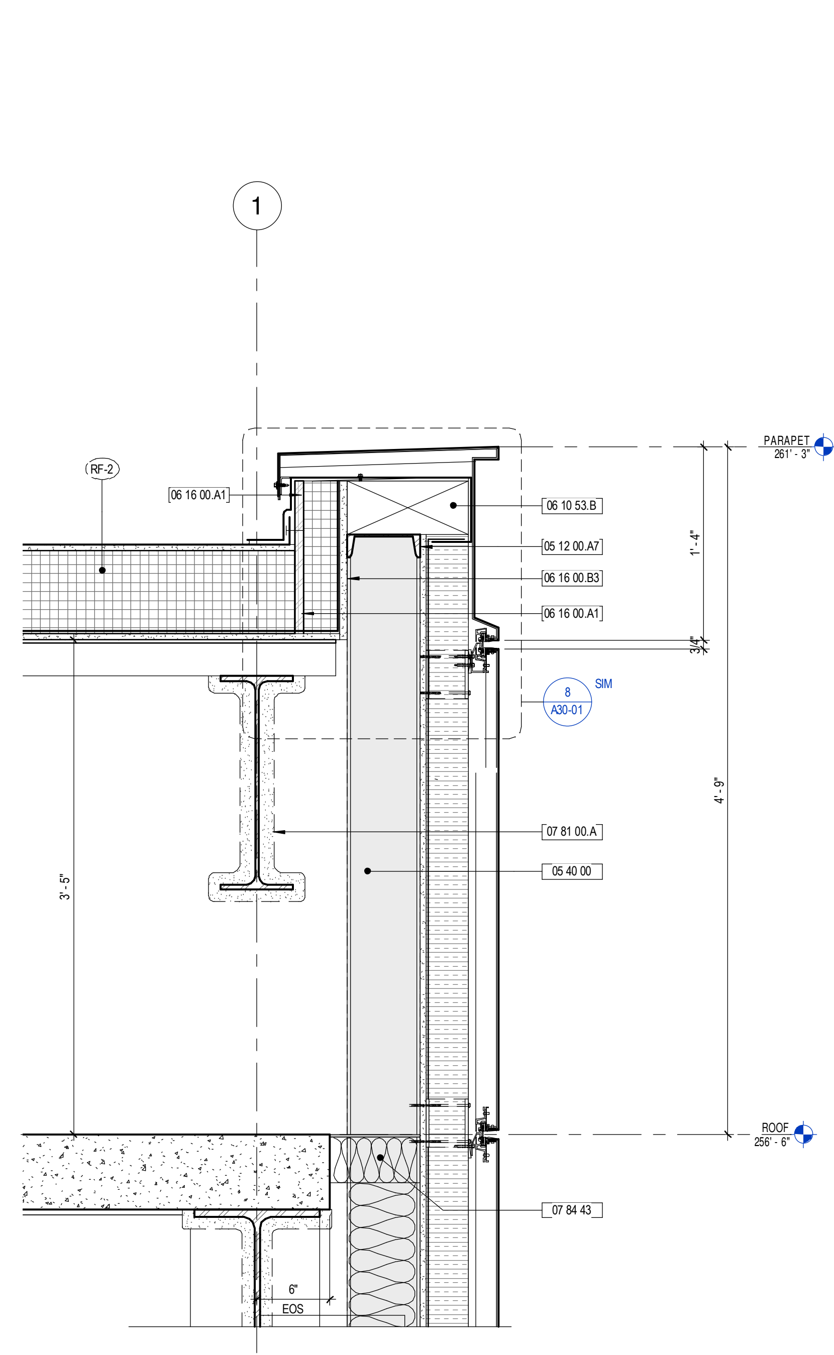
1 HELIPAD - DUNNAGE AT PARAPET 1 1/2" = 1'-0"
