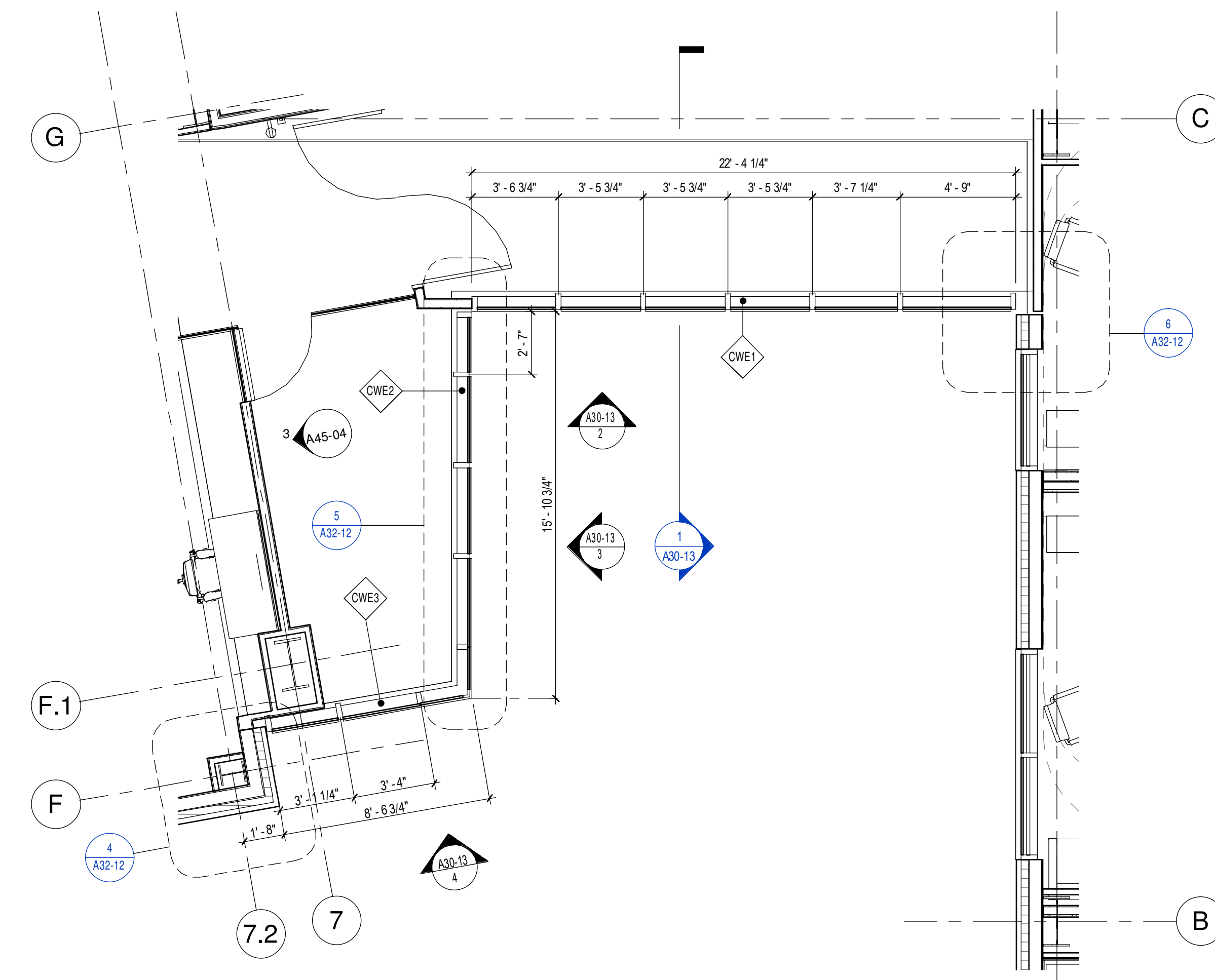
5 CURTAIN WALL - CWE 1/4" = 1'-0"
