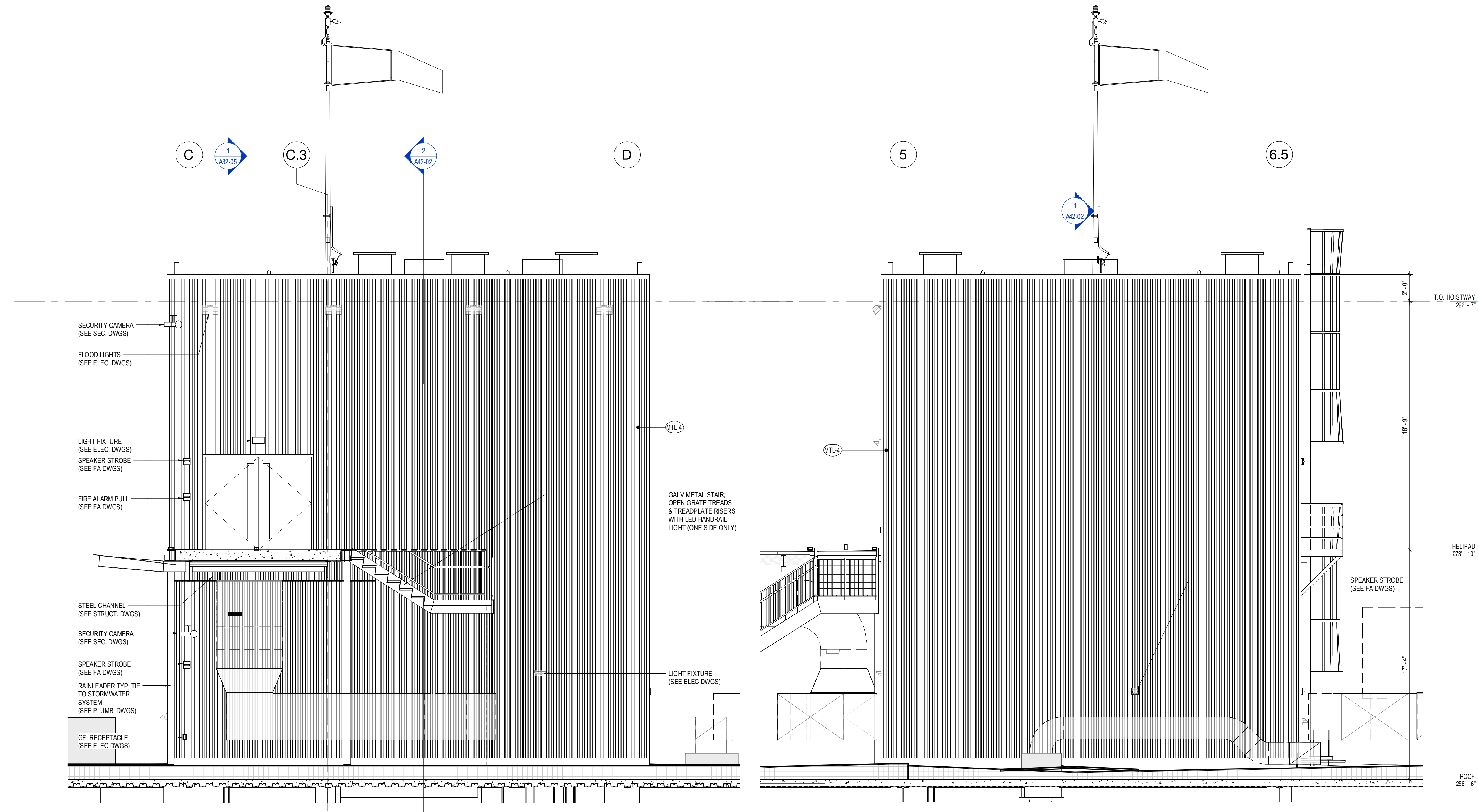
2 ELEVATOR HEADHOUSE - WEST 1/4" = 1'-0"
