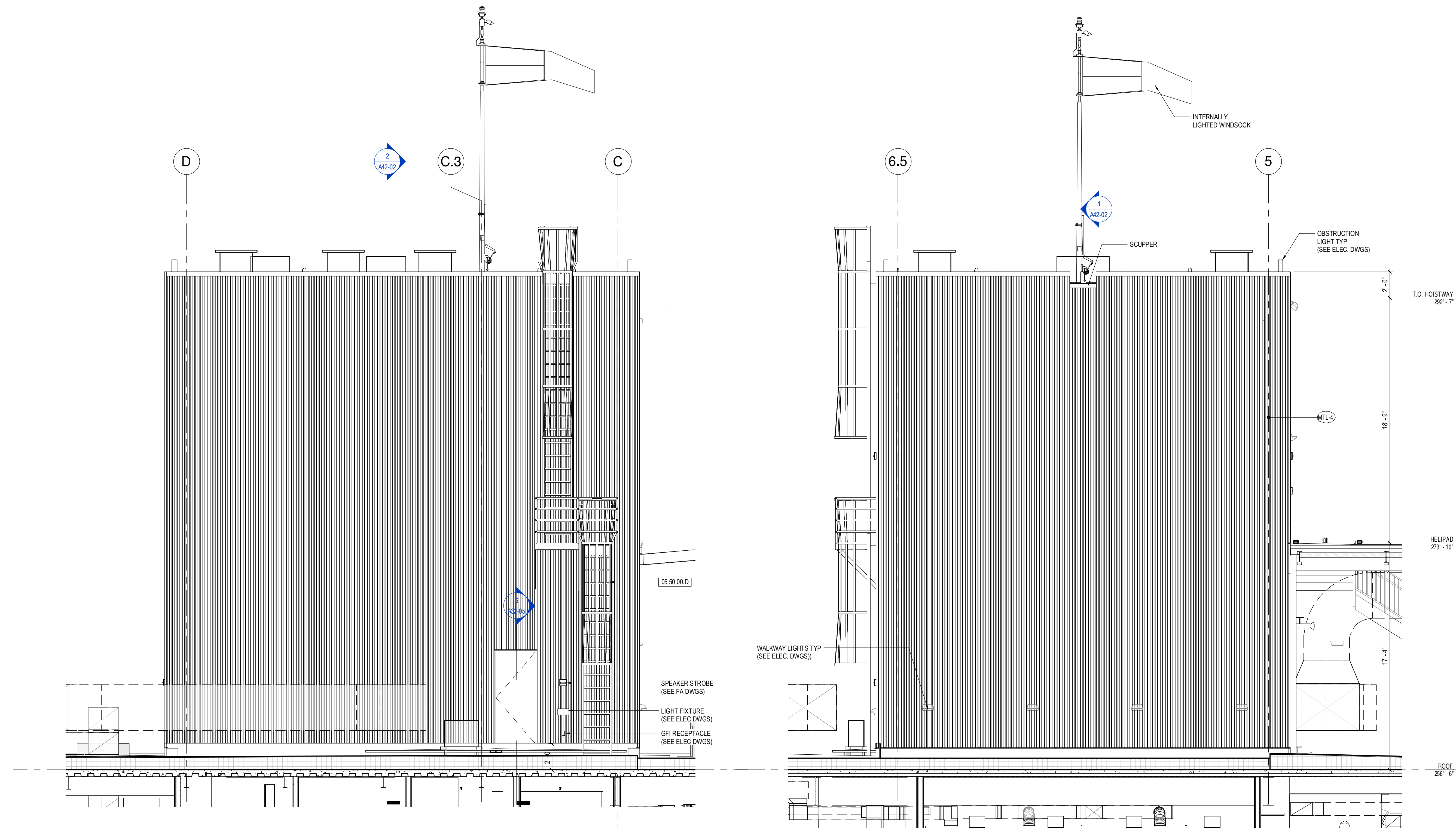
4 ELEVATOR HEADHOUSE - EAST 1/4" = 1'-0"
