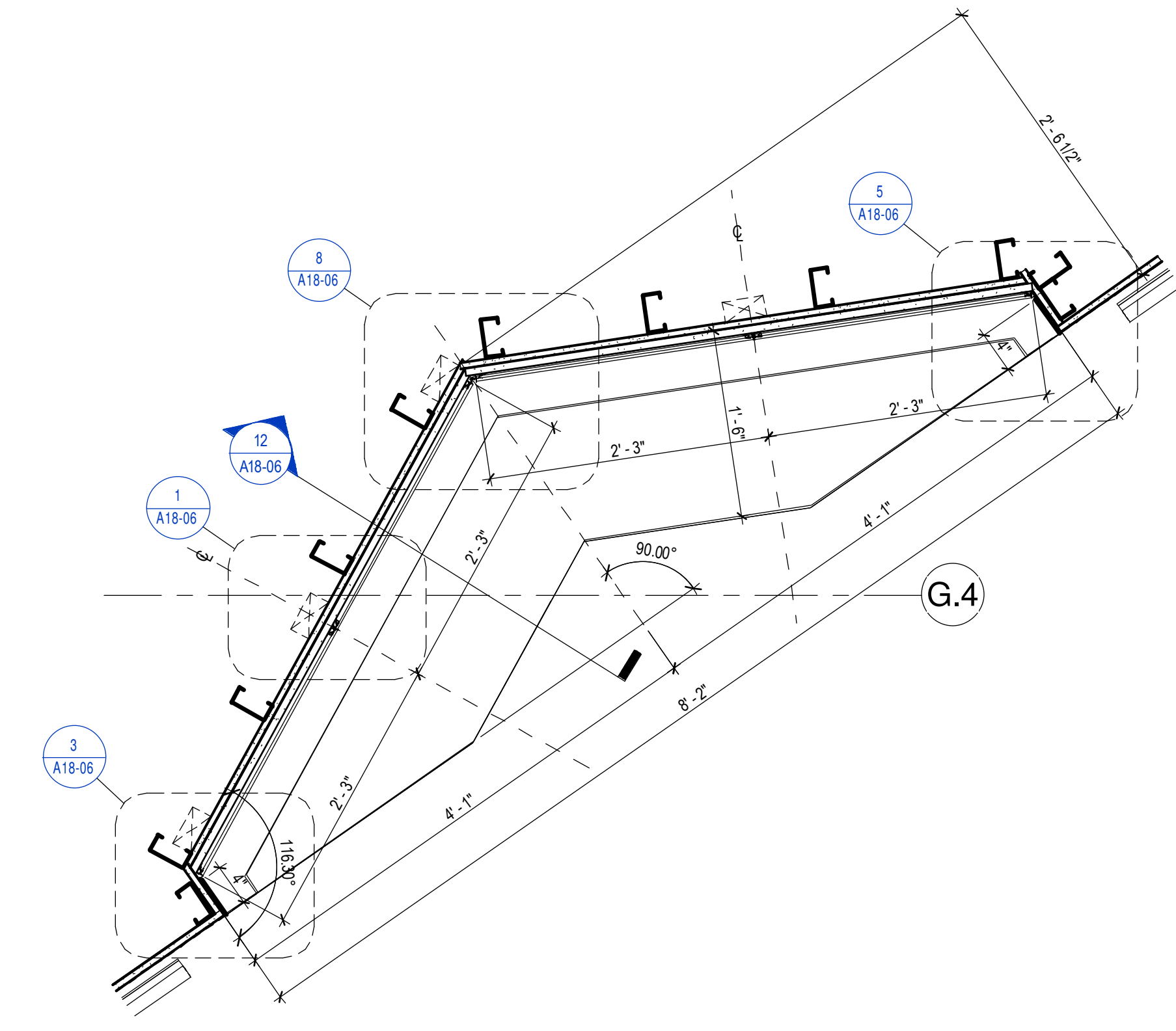
4 SEATING 6076 ENLARGED PLAN 1" = 1'-0"
