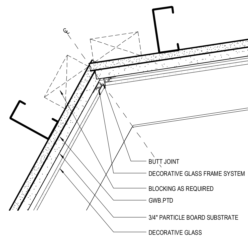
8 PLAN DETAIL MID CONER 3" = 1'-0"
