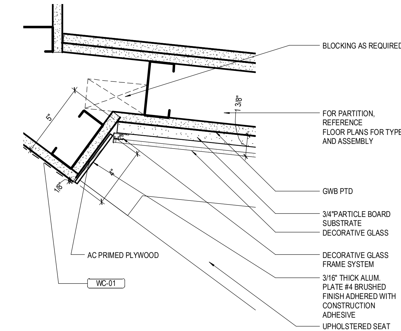
7 PLAN DETAIL CORNER LEFT 3" = 1'-0"
