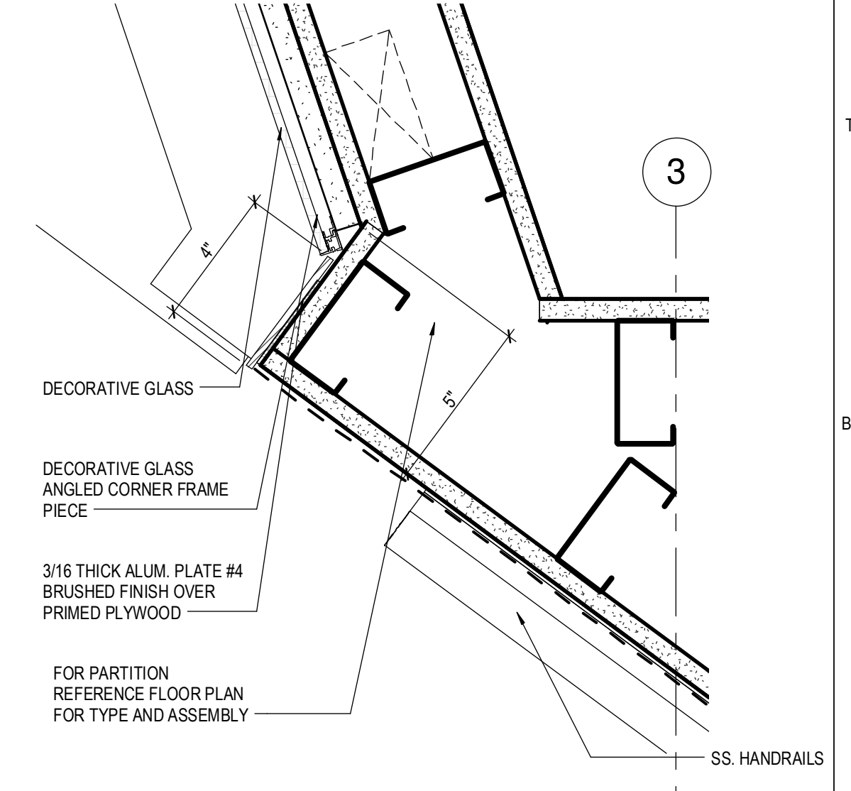
3 PLAN DETAIL CORNER RIGHT 3" = 1'-0"
