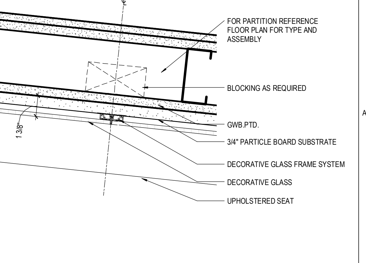
1 PLAN DETAIL - MIDDLE GLASS FRAME JOINT 3" = 1'-0"
