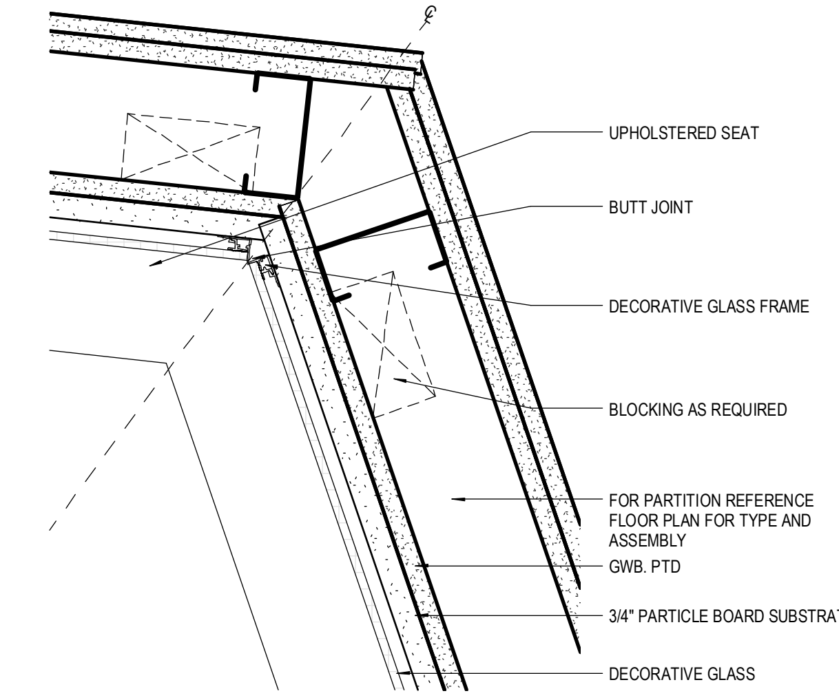
6 PLAN DETAIL BENCH CORNER 3" = 1'-0"
