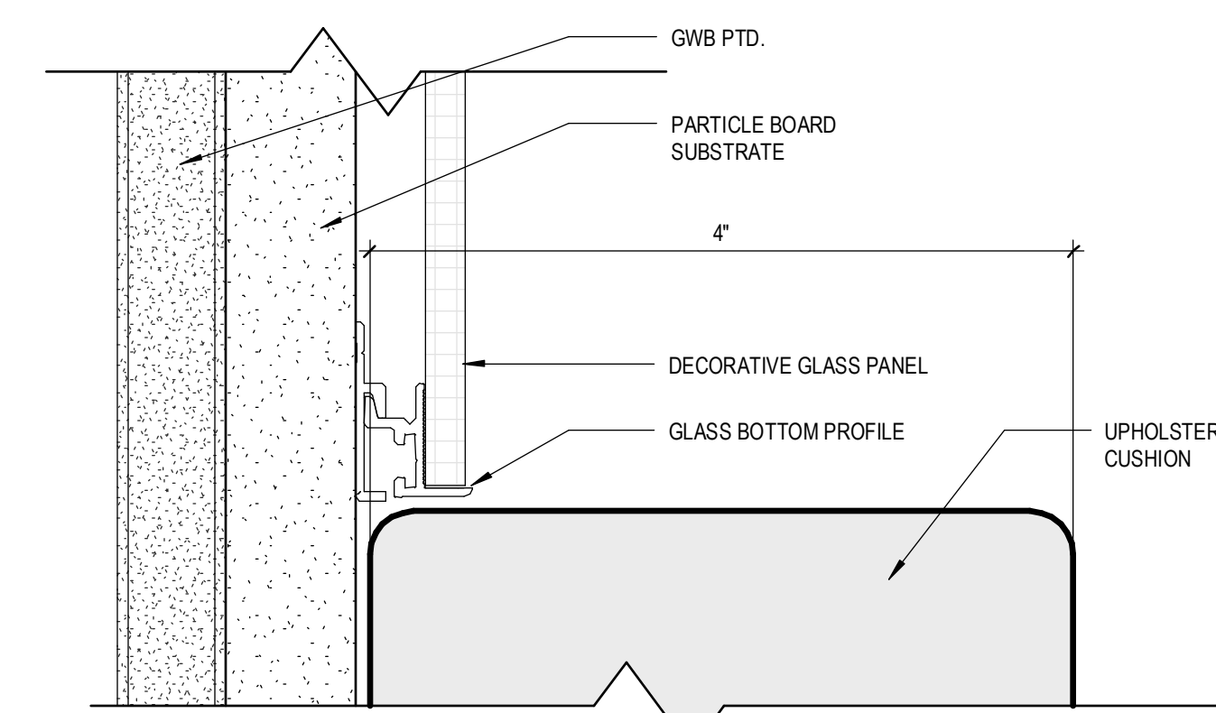
10 DETAIL GLASS BOTTOM FRAME 12" = 1'-0"
