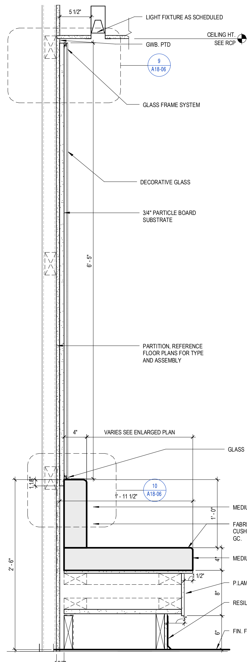
12 SECTION AT DECORATIVE GLASS WITH HIGH TOP BENCH 1 1/2" = 1'-0"
