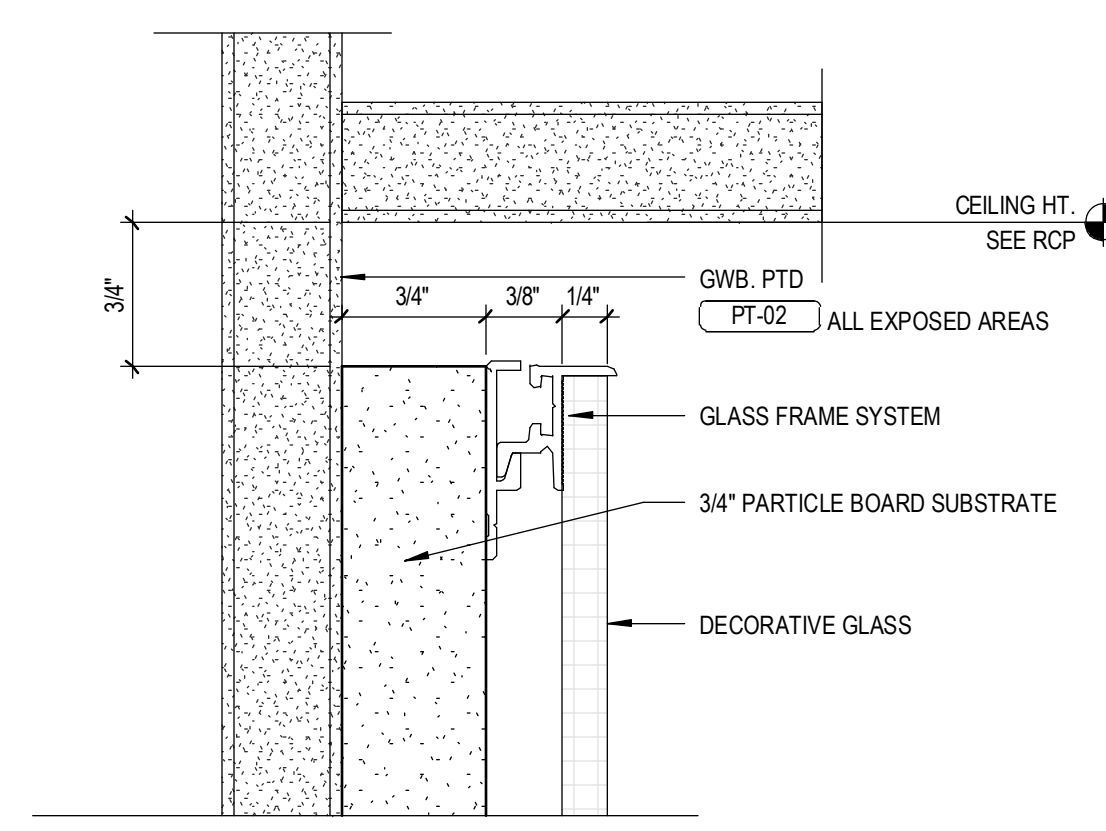
9 DETAIL AT TOP OF GLASS 12" = 1'-0"
