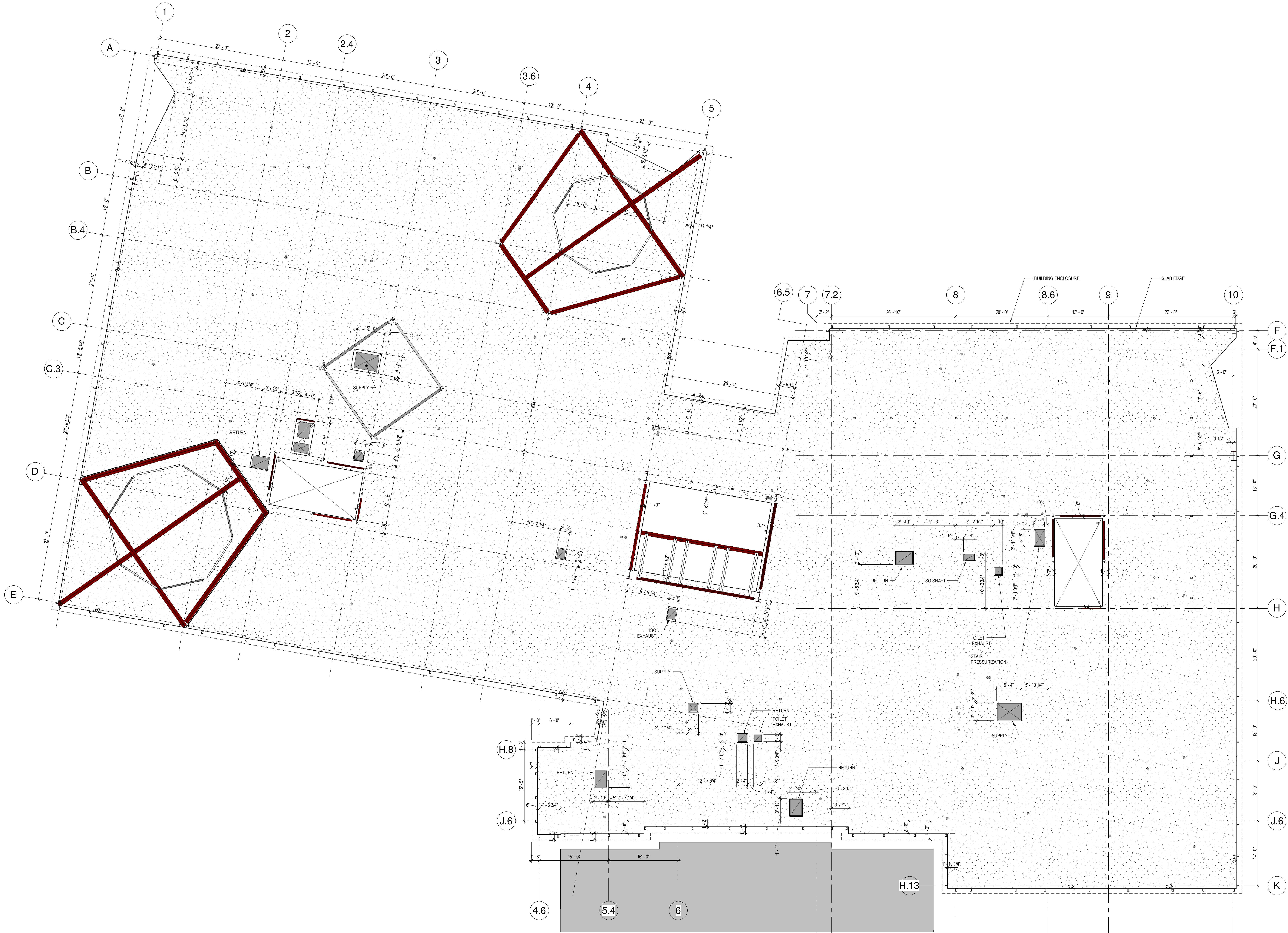
1 ROOF SLAB EDGE PLAN 1/8" = 1'-0"
