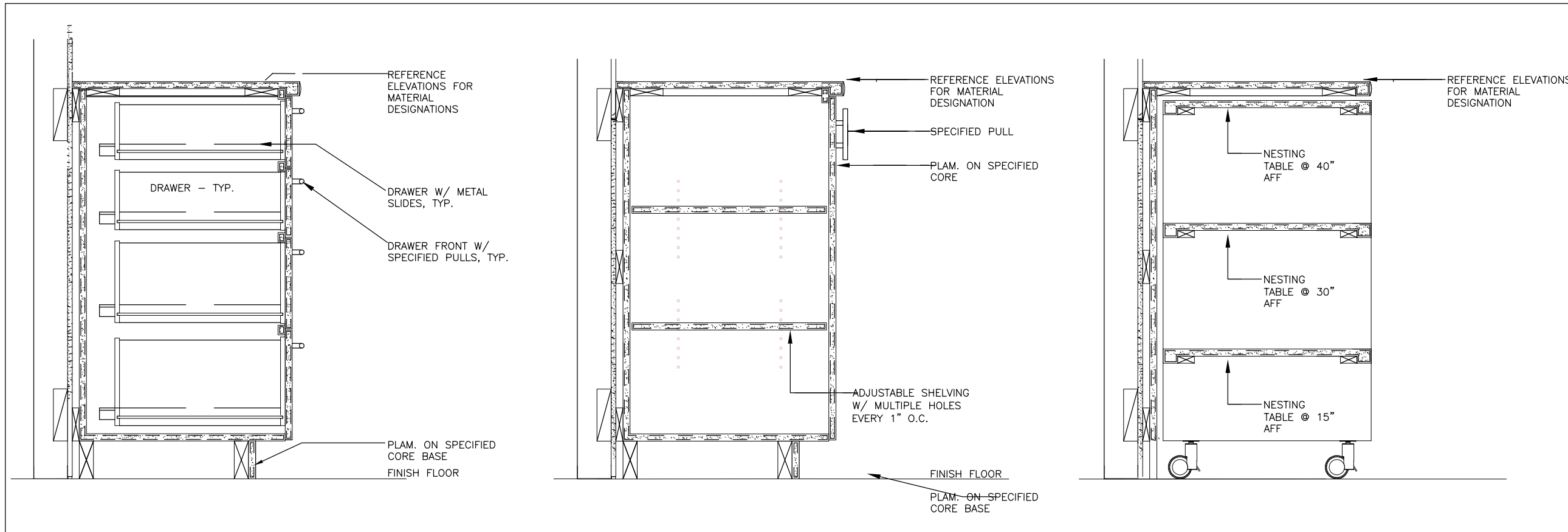
1 SECTION CUT: BANK OF DRAWERS
