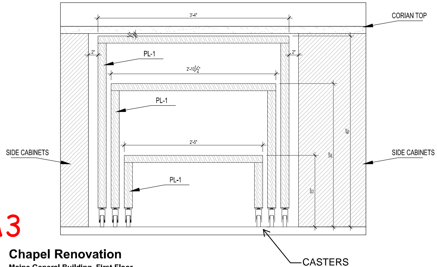
1 SECTION CUT: BANK OF DRAWERS
