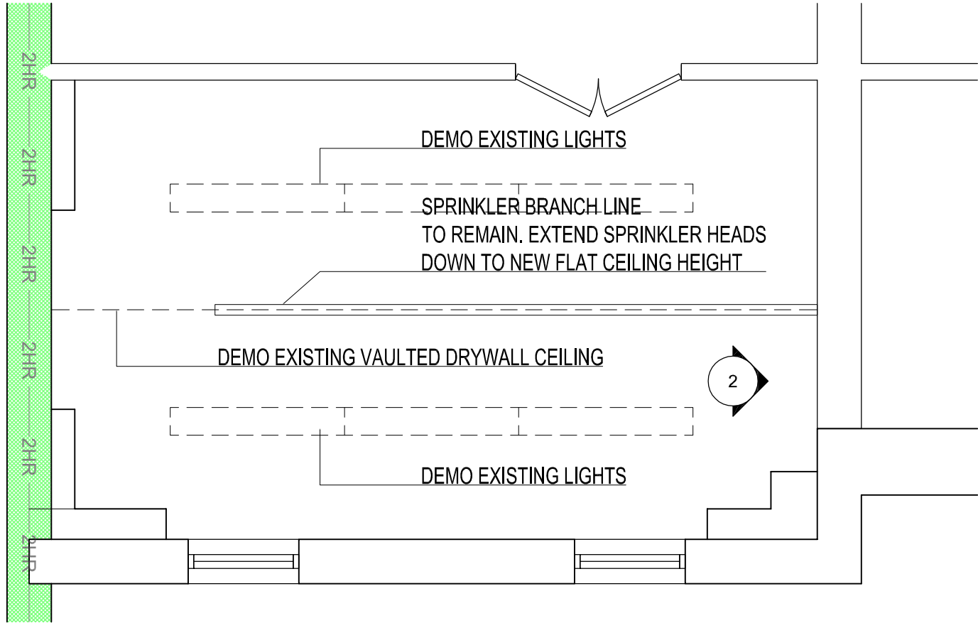
1 DEMOLITION OF CEILING A1.1 | A1.1 0 4'-0" SCALE: 1/4" = 1'-0"
