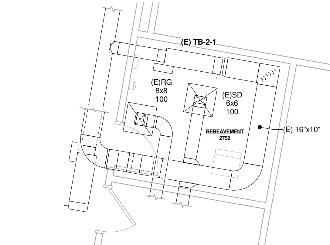
2 SECOND FLOOR BEREAVEMENT DUCT PLAN M302 1/4" = 1'-0"
