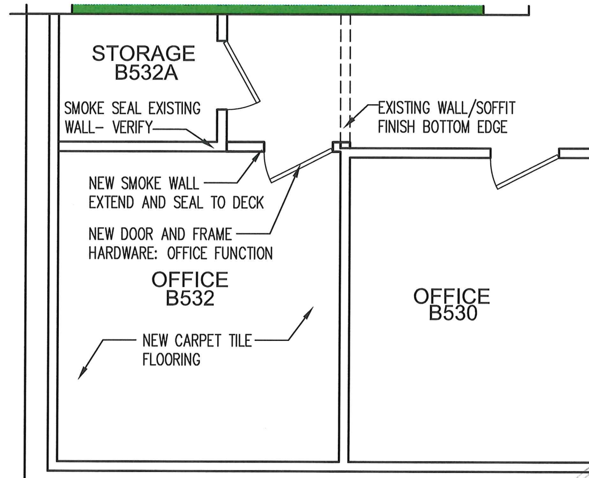
Floor Plan
