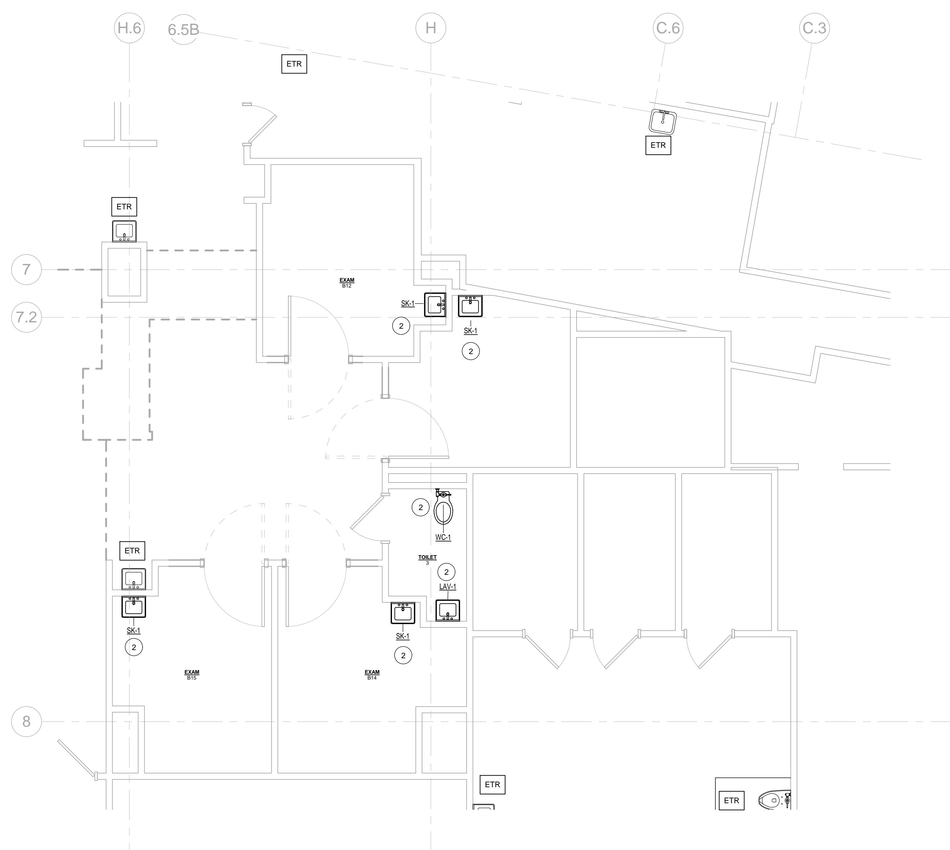
2 FIRST FLOOR PLUMBING NEW WORK P1.0 1/4" = 1'-0"
