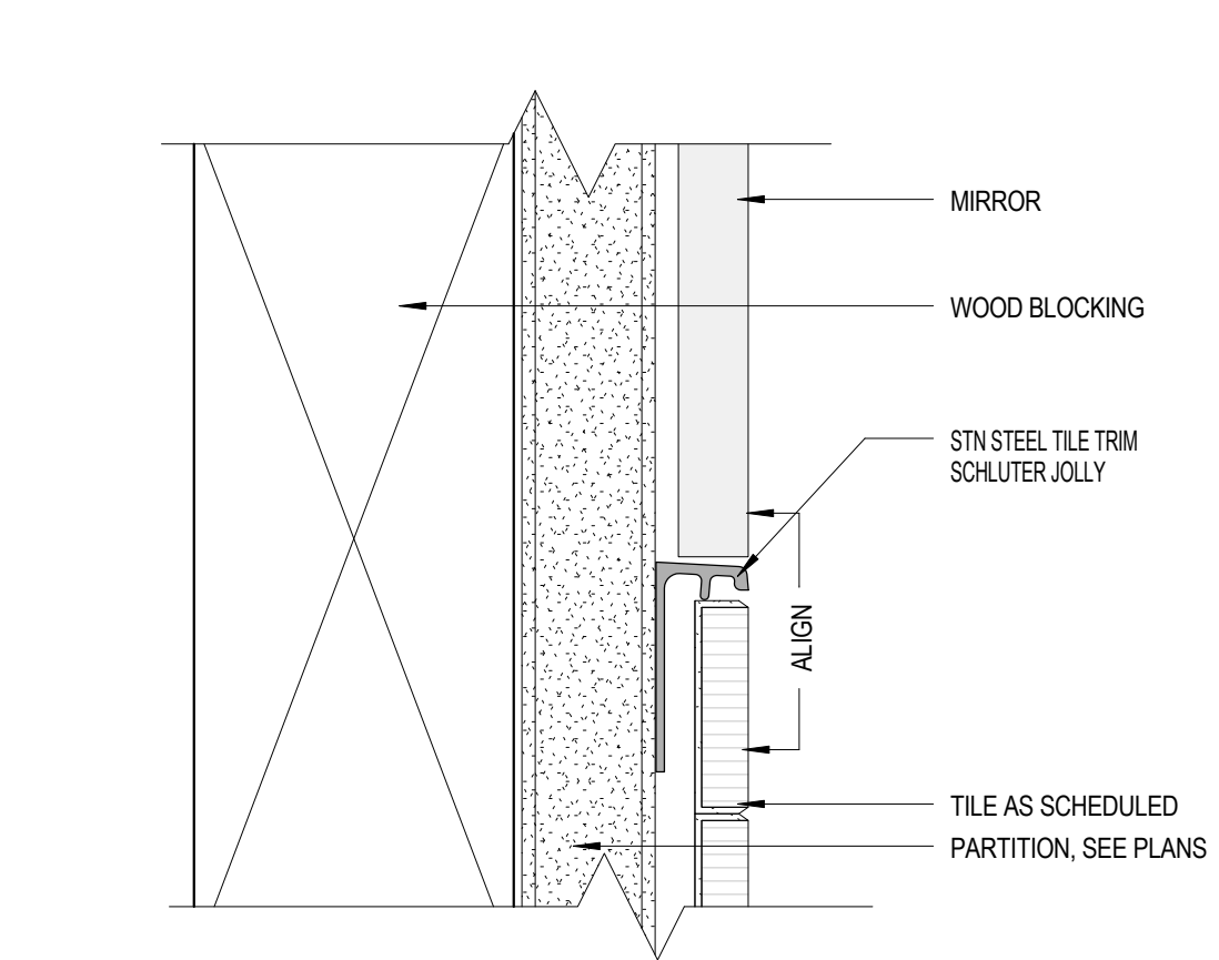
C2 SCHLUTER COVE TRIM 3" = 1'-0"
