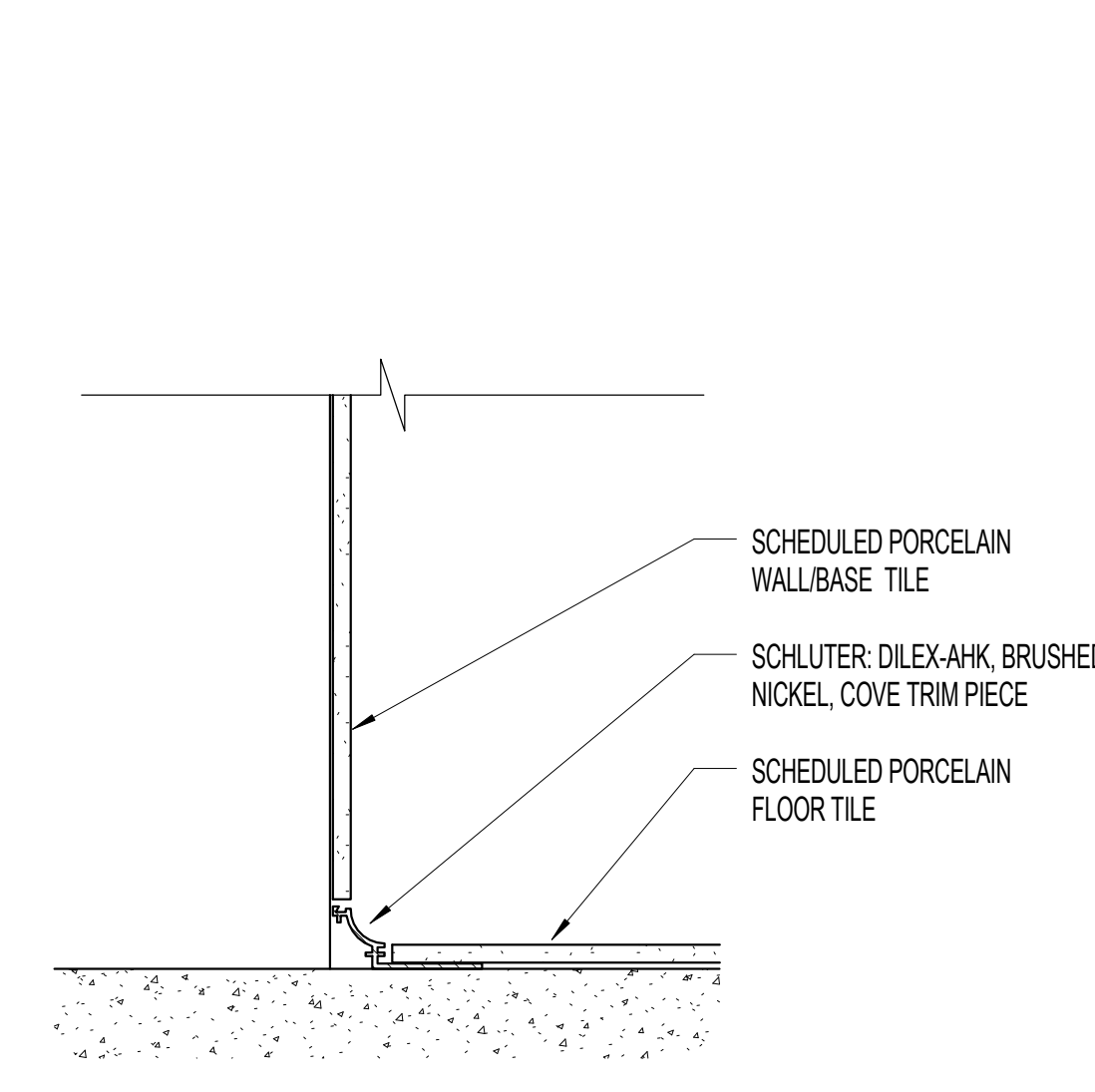
C2 SCHLUTER COVE TRIM 3" = 1'-0"
