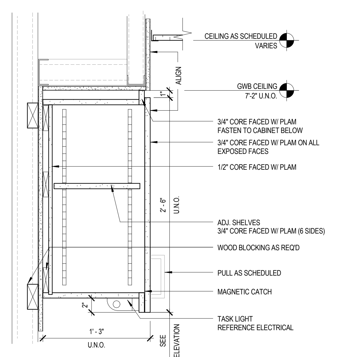
A4 WALL CABINET 1 1/2" = 1'-0"
