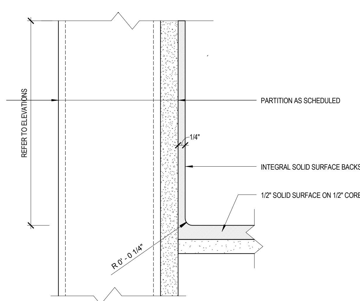
B1 DETAIL - INTEGRAL BACKSPASH 6" = 1'-0"
