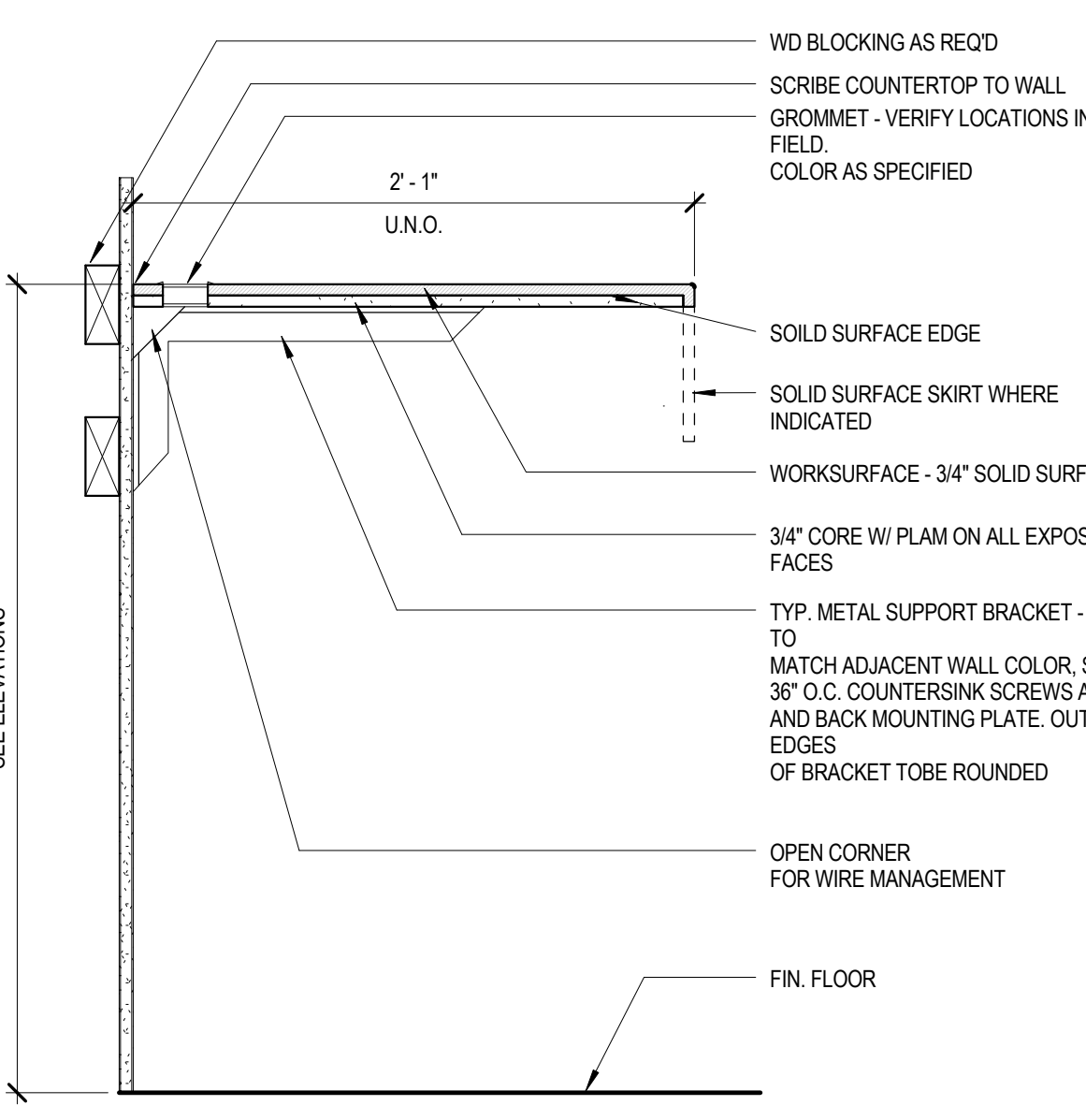
A3 COUNTER - SOLID SURFACE 1 1/2" = 1'-0"
