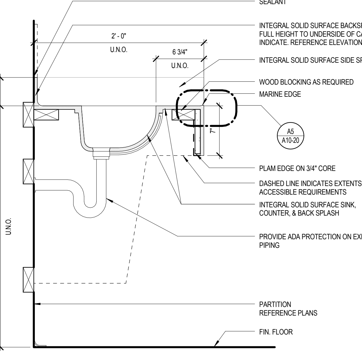
A2 COUNTER W/ INTEGRAL SINK - ROUND 1 1/2" = 1'-0"
