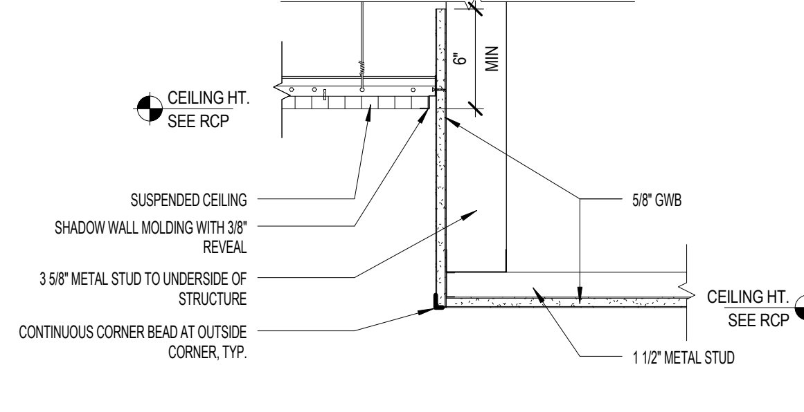
D3 CEILING DETAIL @ GWB/ACT SOFFIT 1 1/2" = 1'-0"
