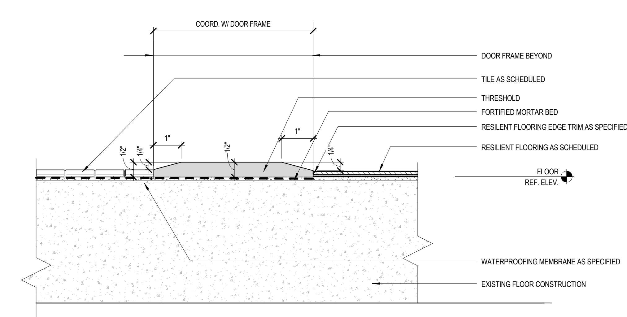
B5 DETAIL - THRESHOLD 6" = 1'-0"
