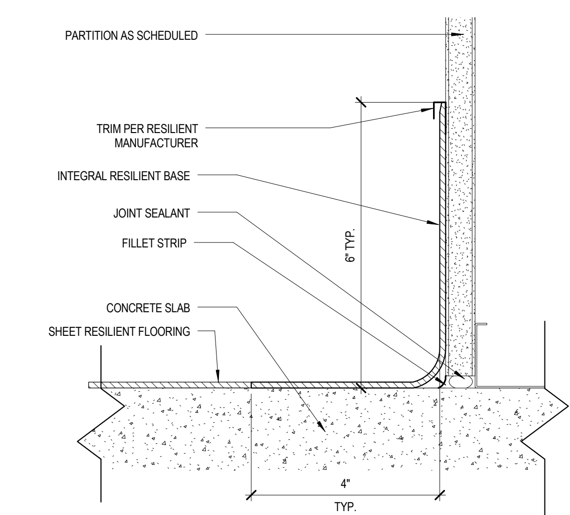
B3 WALL BASE DETAIL RESILIENT BASE @ SHEET RESILIENT FLOORING 6" = 1'-0"
