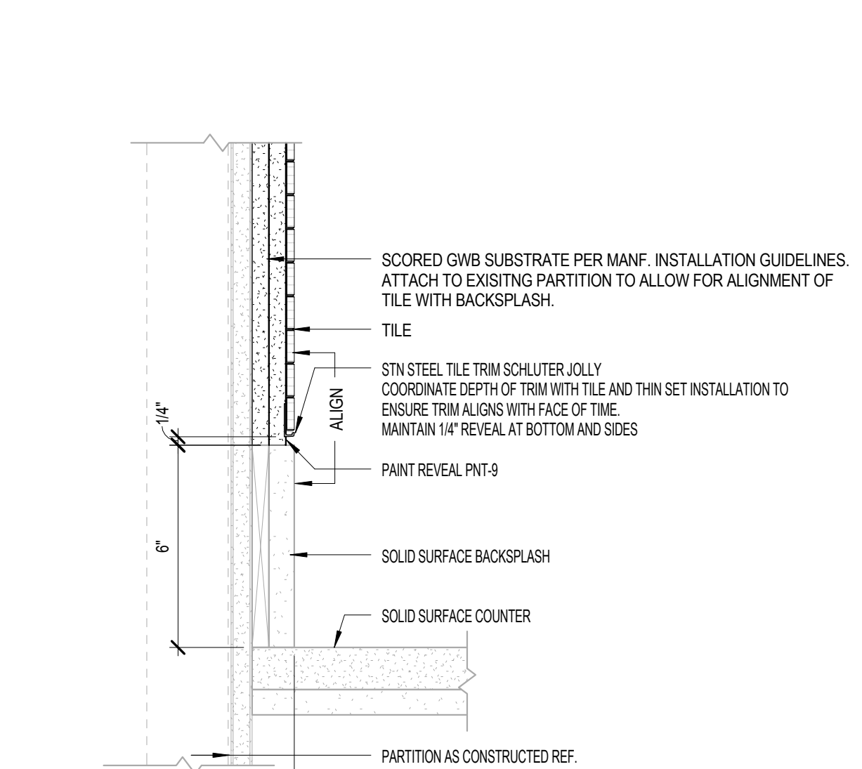
C1 DETAIL - TILE AT BACKSPASH 3" = 1'-0"
