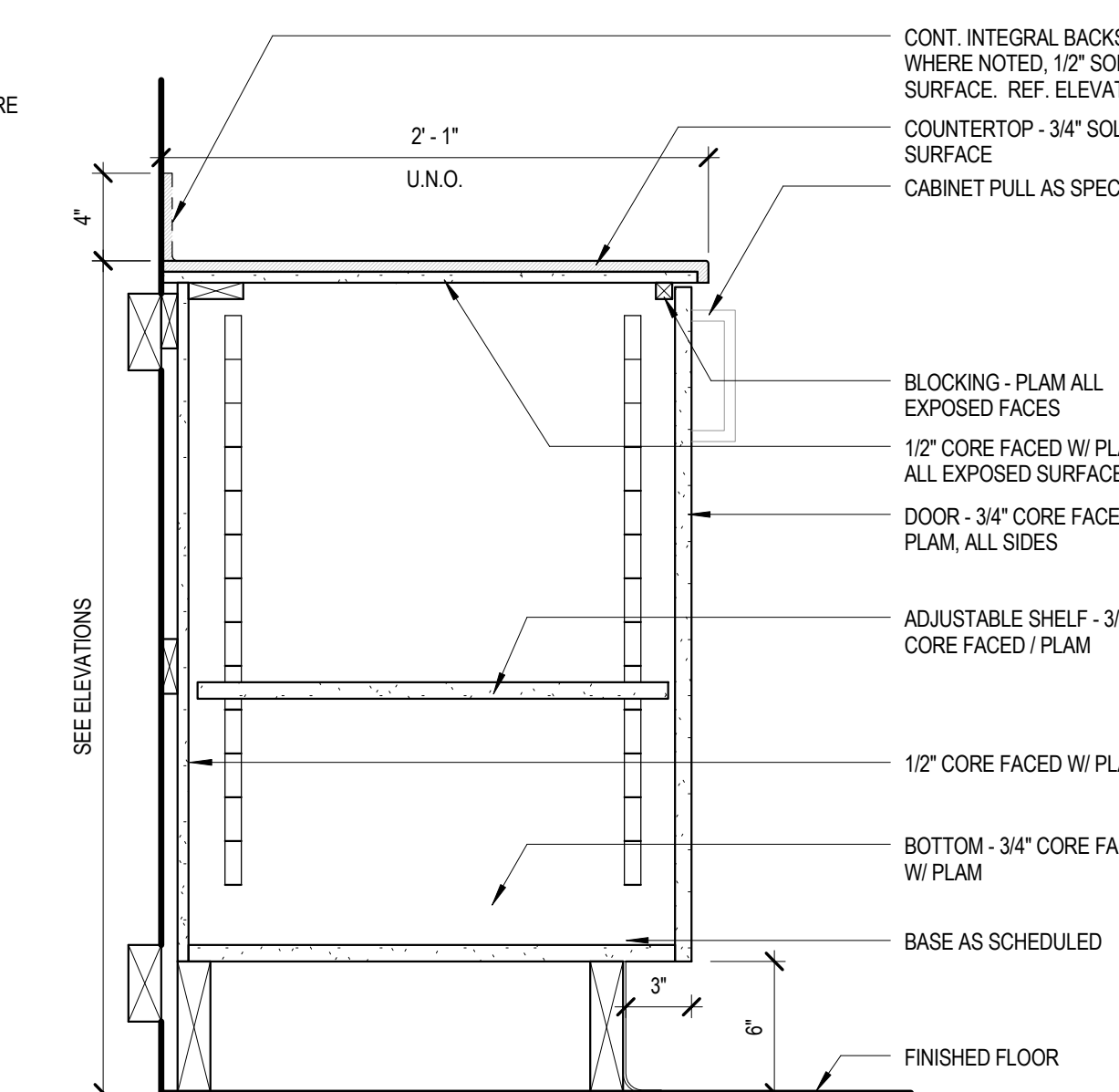
A1 BASE CABINET W/SHELF - SOLID SURFACE 1 1/2" = 1'-0"
