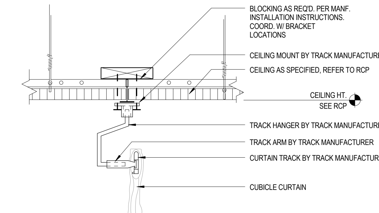
D1 CEILING DETAIL @ CUBICLE CURTAIN 3" = 1'-0"
