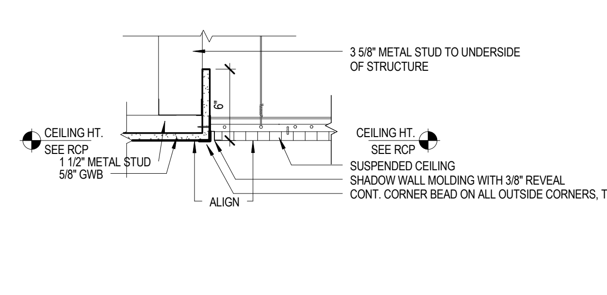
D2 CEILING DETAIL @ GWB/ACT COPLANAR 1 1/2" = 1'-0"
