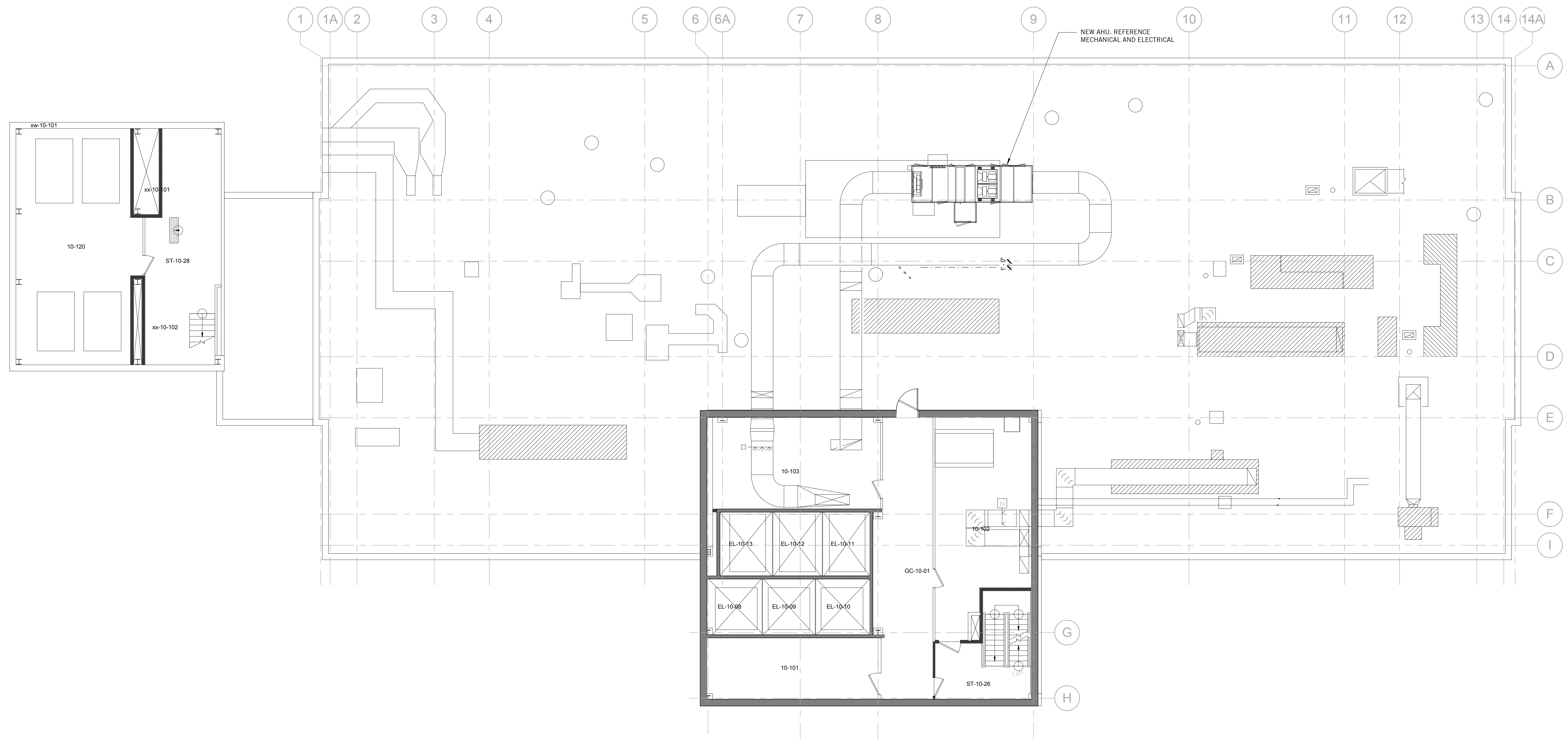
1 RICHARDS PENTHOUSE 1/8" = 1'-0"
