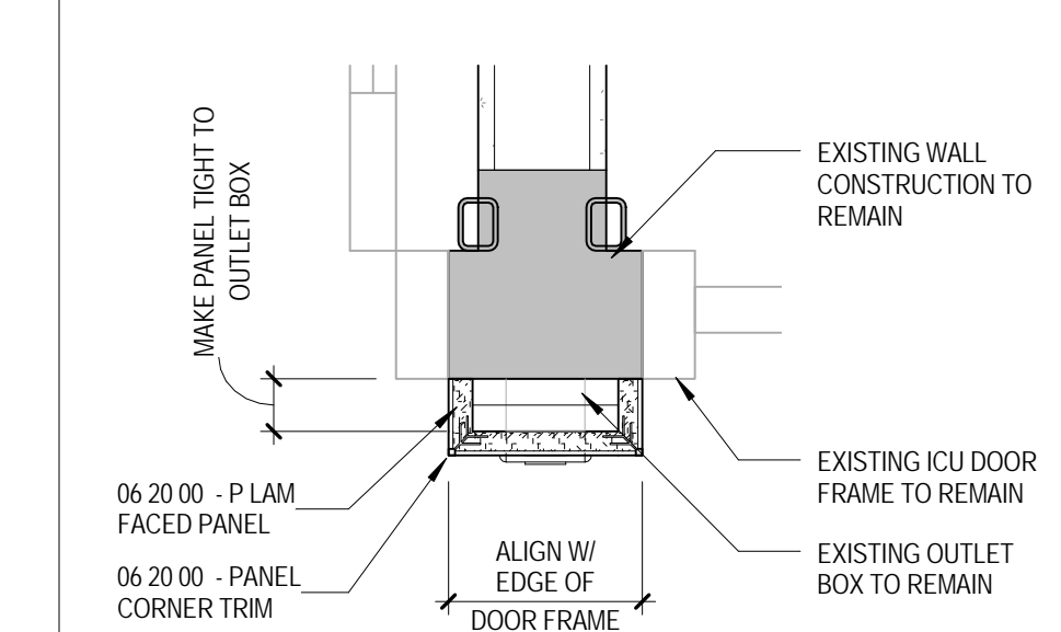
F13 PLAN DETAIL - PLAM OUTLET COVER - TYP. A7.1s 1/16" = 1'-0"
