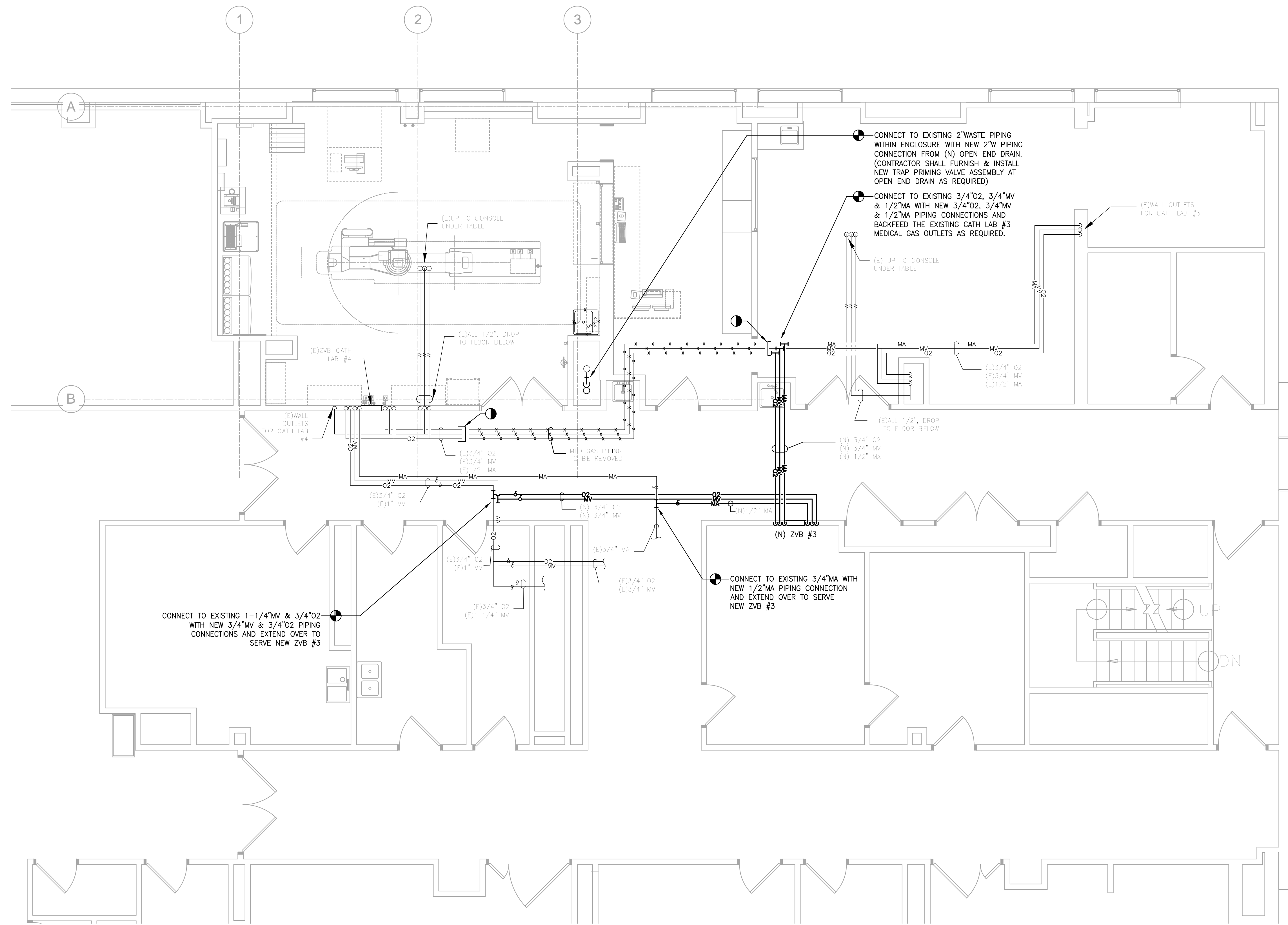
1 NEW WORK FLOOR PLAN SCALE: 1/4"=1'-0"
