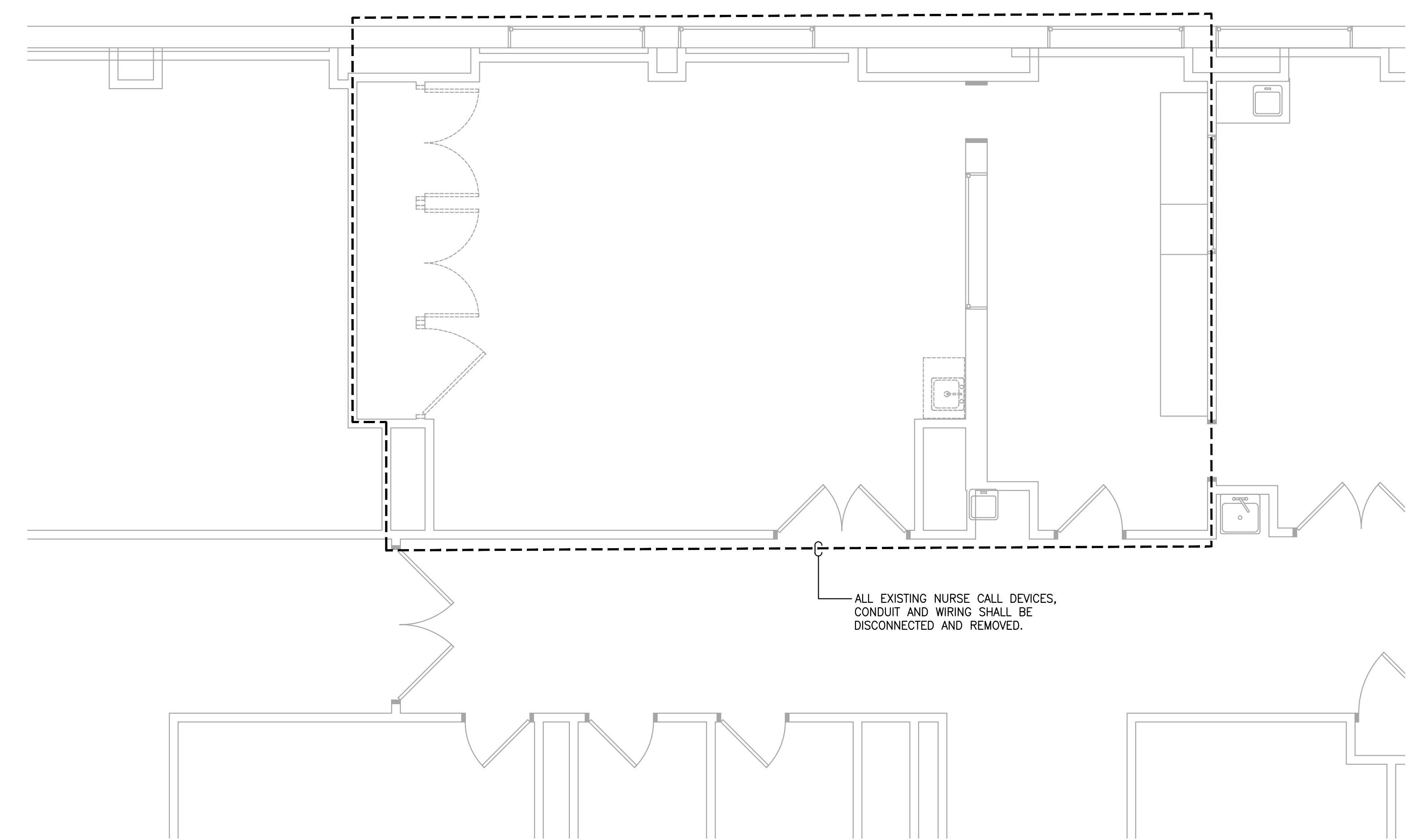
1 DEMOLITION 8TH FLOOR NURSE CALL PLAN SCALE: 1/4"=1'-0"
