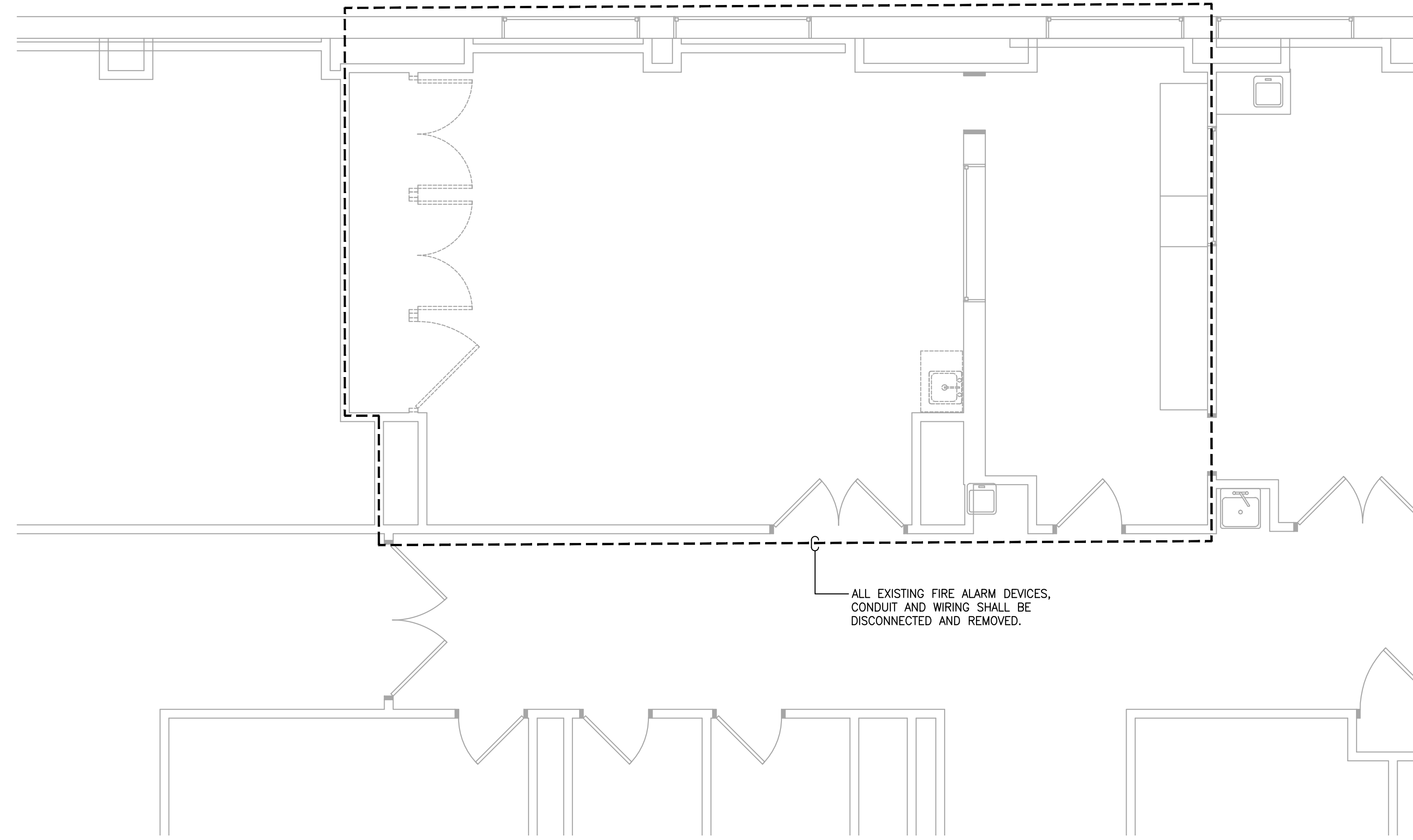
1 DEMOLITION 8TH FLOOR FIRE ALARM PLAN SCALE: 1/4"=1'-0"
