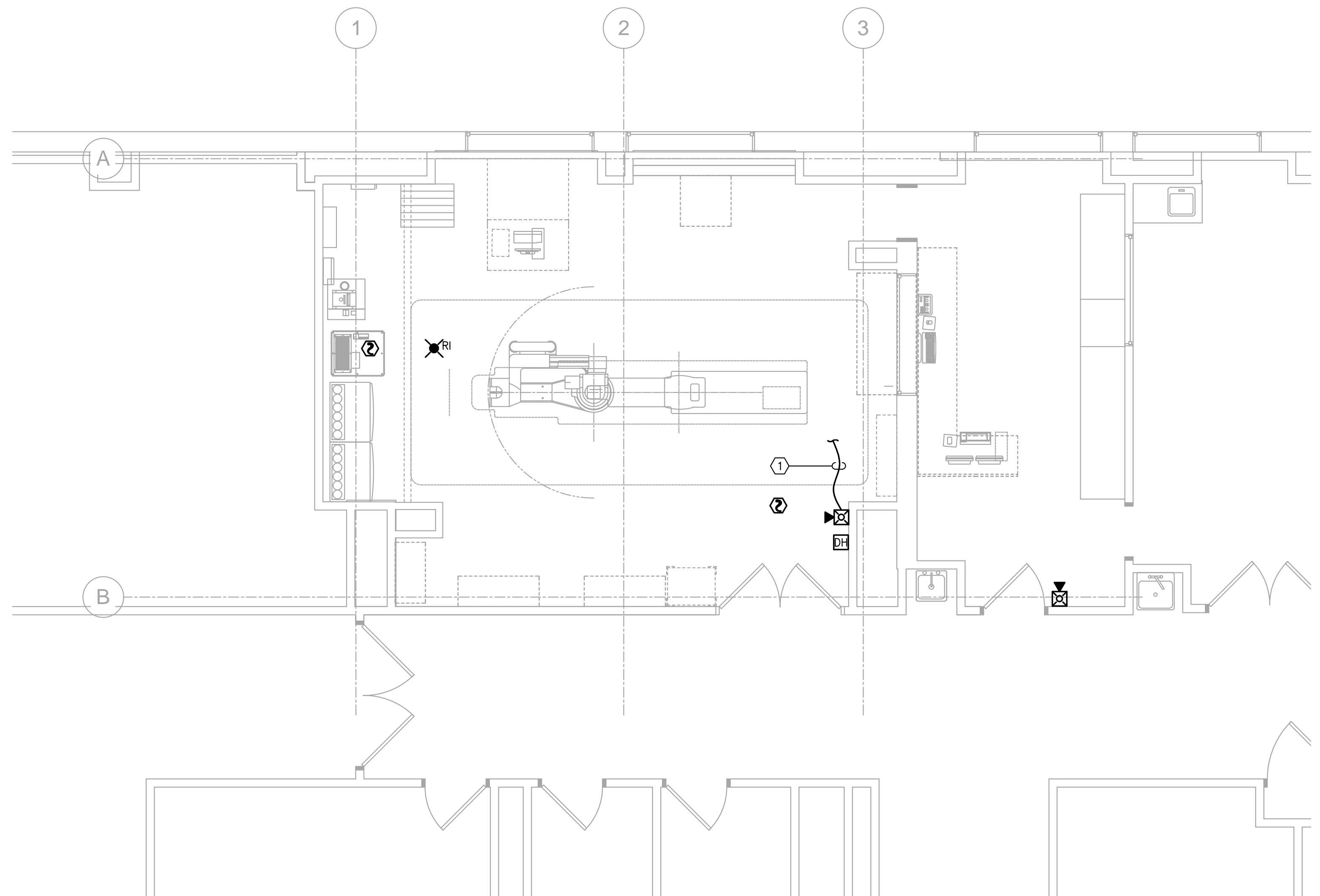
2 NEW 8TH FLOOR FIRE ALARM PLAN SCALE: 1/4"=1'-0"
