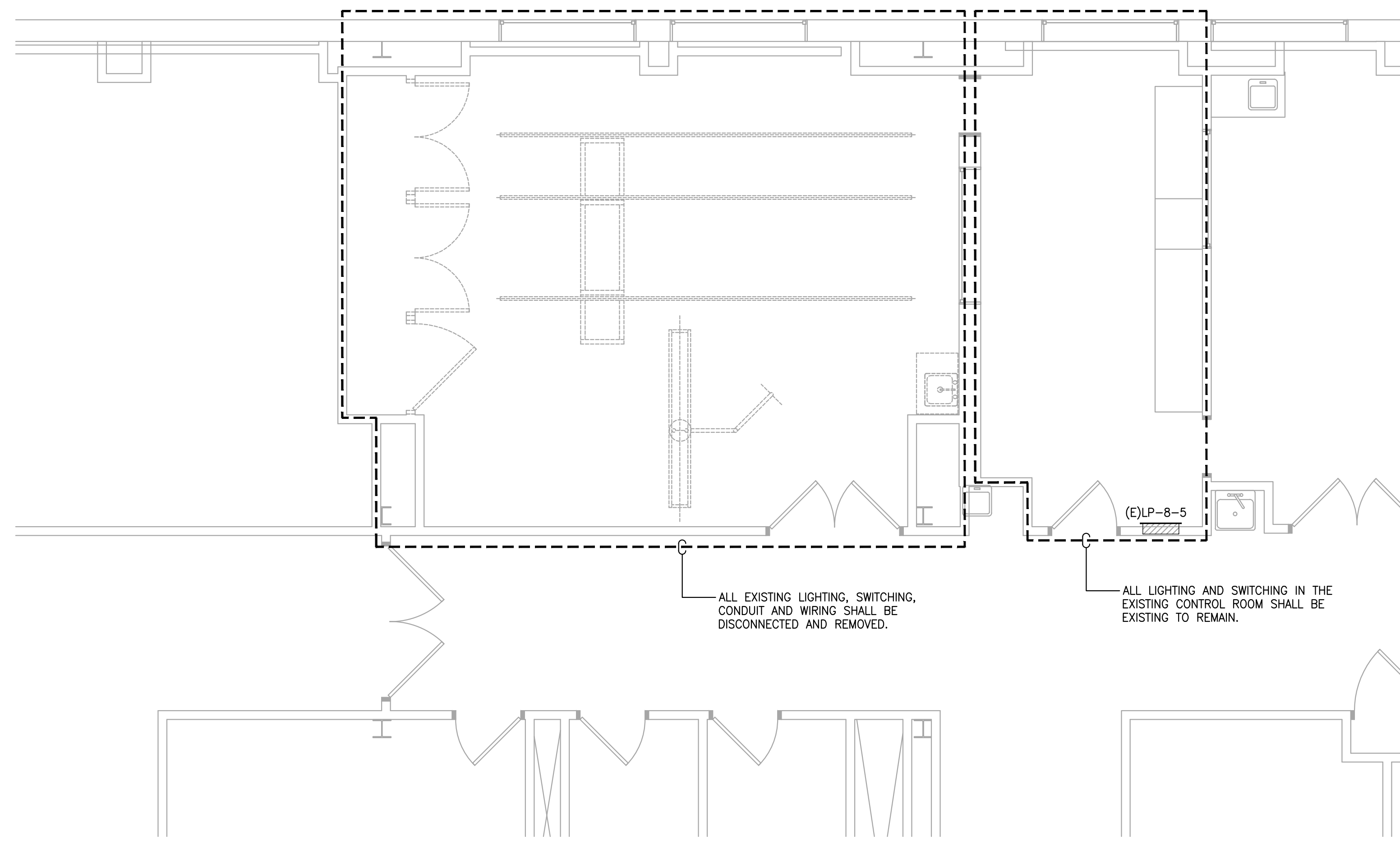
1 DEMOLITION 8TH FLOOR LIGHTING PLAN SCALE: 1/4"=1'-0"
