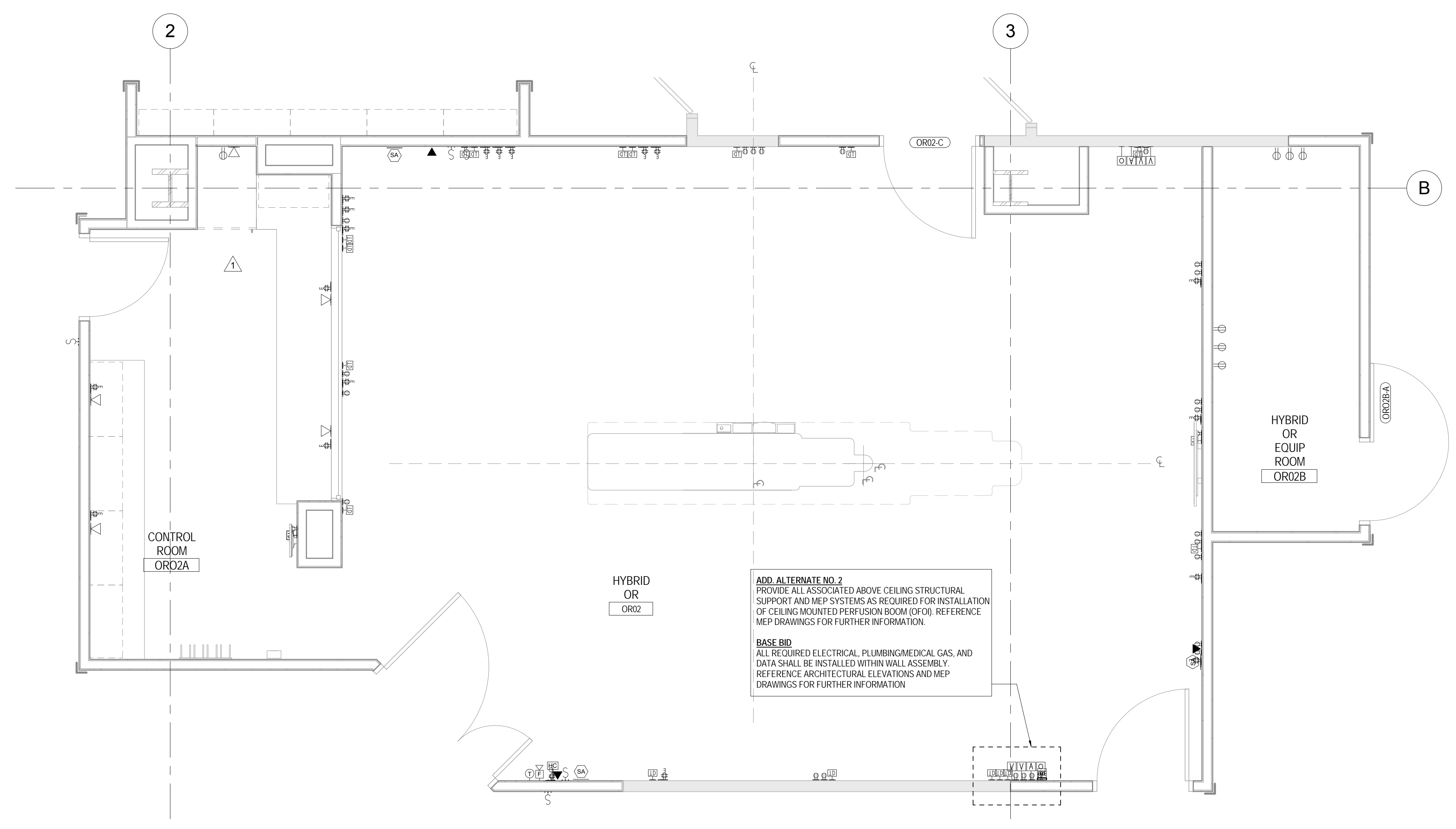
1 HYBRID OR 3/8" = 1'-0"
