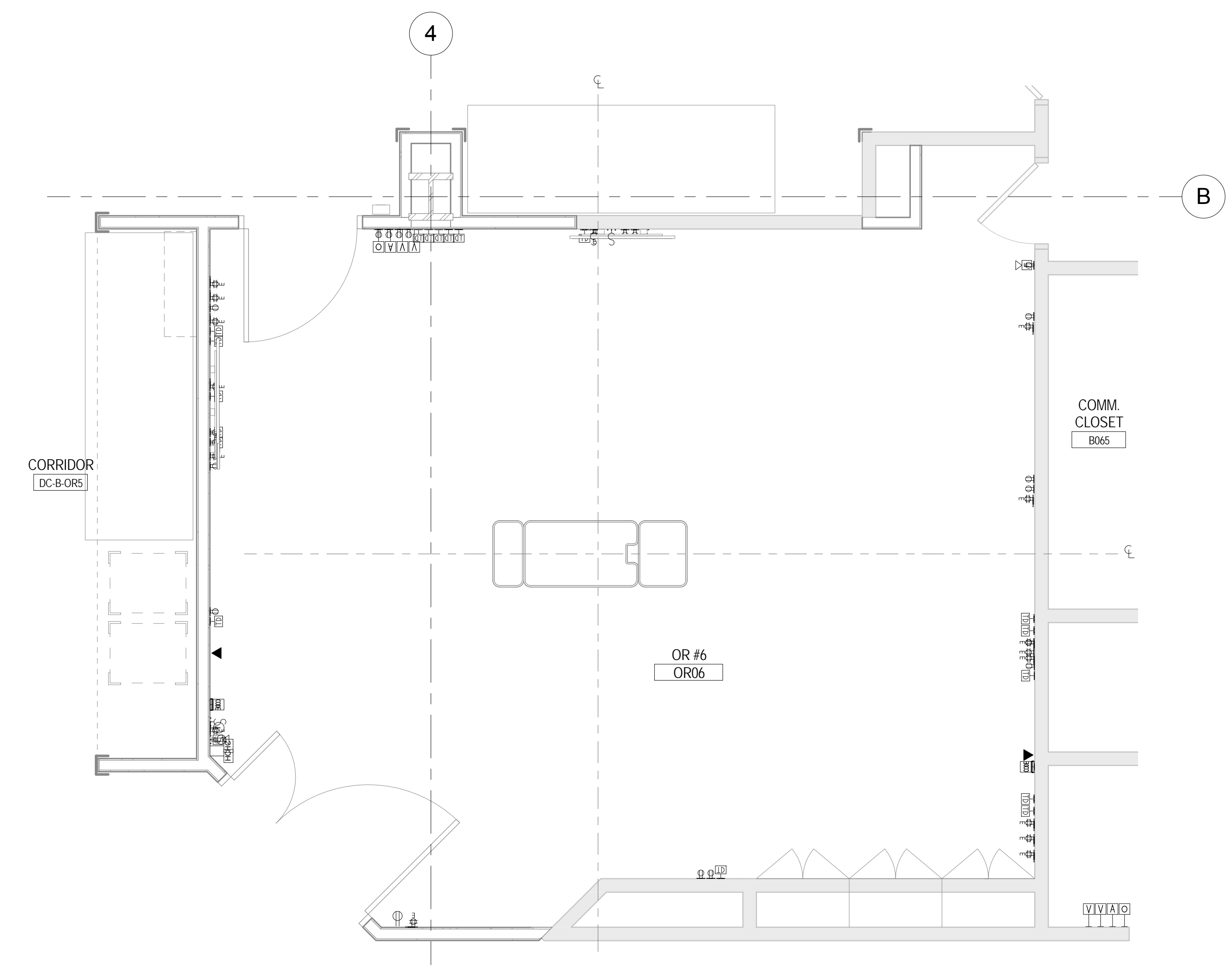
2 OR 6 3/8" = 1'-0"
