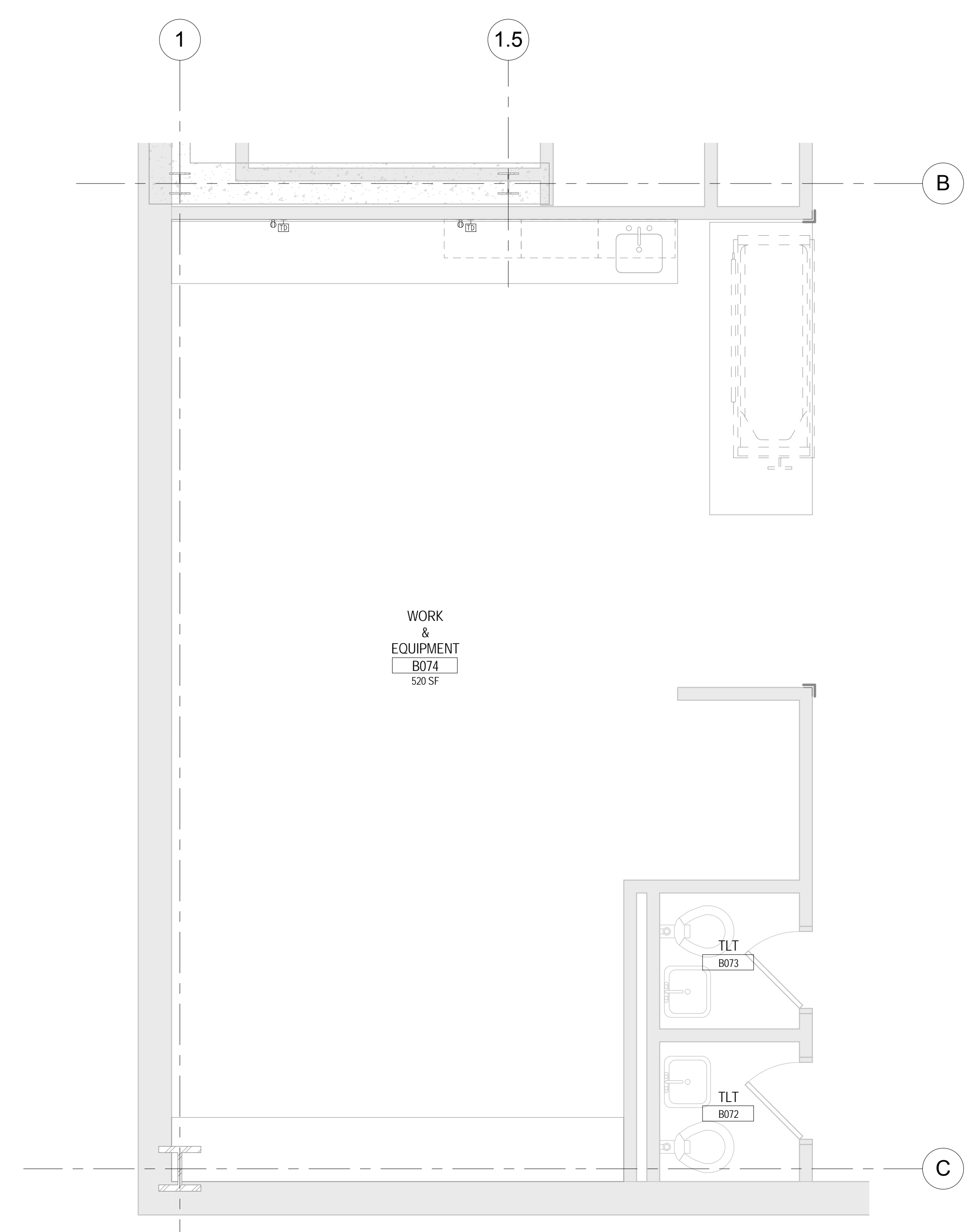
3 ALTERNATE #1 WORK & EQUIPMENT 3/8" = 1'-0"
